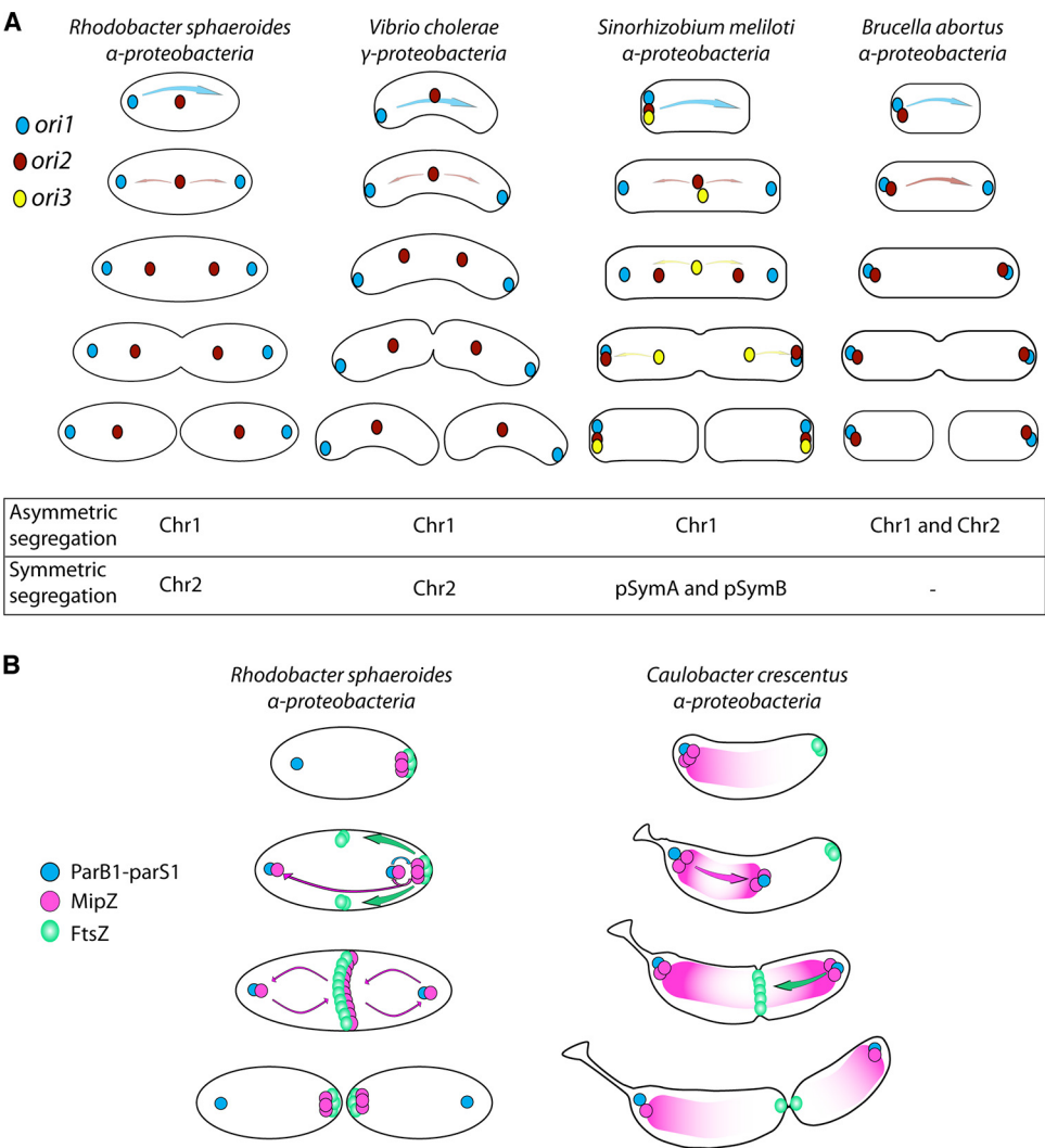
FIG 7 (A) Comparative segregation model for origins of replicons in multichromosomal bacteria. Replicons contained in multichromosomal proteobacteria mainly exhibit two different modes of segregation. Some replicons segregate according to an asymmetric migration from cell pole to cell pole, while others segregate bidirectionally and symmetrically from midcell. Interestingly, various combinations of segregation patterns are observed for the multiple replicons contained in different bacterial species, as show here for Rhodobacter sphaeroides (this work), Vibrio cholerae (21), Sinorhizobium meliloti (22), and Brucella abortus (31). (B) Comparison of protein dynamics through the cell cycle of R. sphaeroides and C. crescentus .
