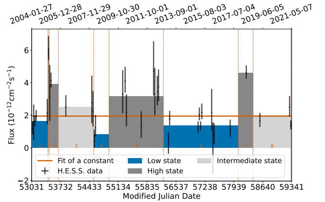
Fig. 1. Thirty-day-binned H.E.S.S. light curve above 300 GeV with its Bayesian blocks and source states. The H.E.S.S. data points are represented by the black data points and a constant fit by the solid orange line. Dashed orange lines indicate a change in the flux level. The blue blocks represent the low state, the light gray the intermediate state, and the dark gray blocks the high state blocks. The orange numbers at the bottom indicate the labels of the blocks.
