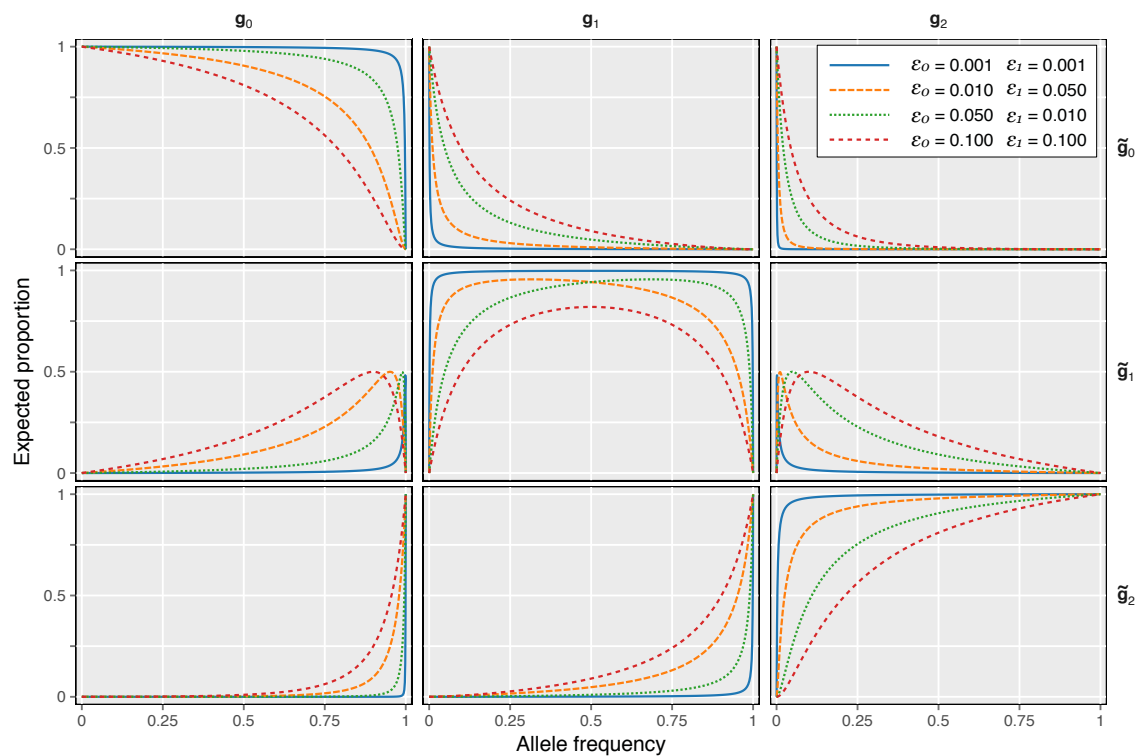
Figure 4.1: Expected error distributions in genotype and allele-based models. The graphs show the expected proportion of true genotype g_j observed genotype as (\tilde{g}_i) given the population allele frequency; calculated at different, nominal error rates (see legend). The error functions provided in Table 4.1 (page 112) were used as in Equation (4.3) (page 111) and results were normalised to sum to 1 per true genotype class (columns).
