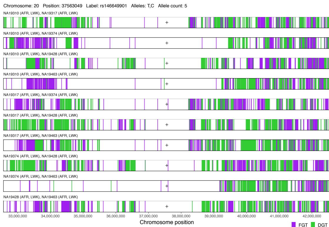
Figure 3.15: Example of breakpoints detected in 1000 Genomes, chr. 20. One of the target sites analysed was randomly selected and breakpoint detection was performed for all pairs of individuals sharing the focal allele. The plot shows all breakpoints detected using the FGT and DGT relative to the allelic configuration observed at the target site ( cross ), within a 10 Mb region around the target position. Sample IDs (and population codes) as found in 1000 Genomes data are shown on the top of each pairwise analysis. Note that any breakpoint detected using the DGT also implies detection through the FGT.
