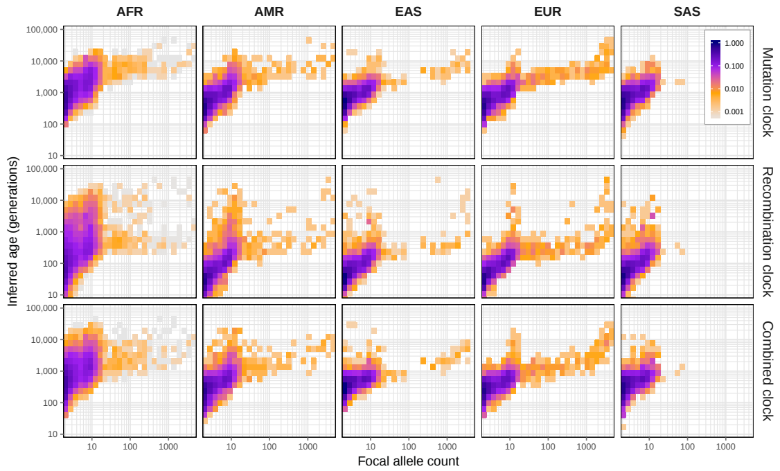
Figure 5.20: Allele age estimated by population in 1000 Genomes, chr. 20. Age was estimated for alleles shared within the same population group contained in the 1000G sample, using the relaxed nearest neighbour approach to select discordant pairs. Shared haplotype detection was performed using the haplotype-based HMM and age was estimated under each of the three clock models ( \mathcal{T}_M , \mathcal{T}_R , and \mathcal{T}_{MR} ). Colours indicate the maximised density of allele age by focal allele frequency. Note that results are shown on log-log-scale.
