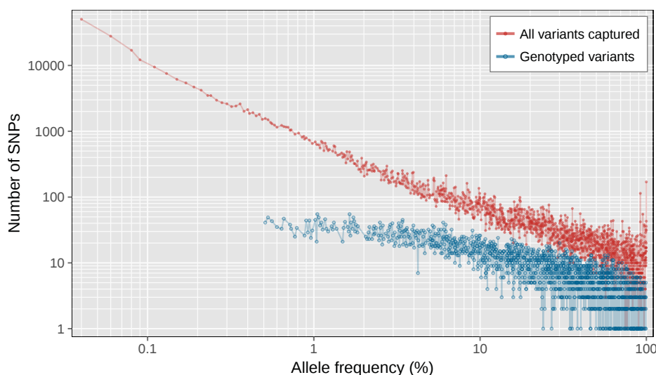
Figure 2.3: Site frequency spectrum of variants captured in GoT2D, chr. 20. The site frequency spectrum (SFS) is shown for SNPs as captured in the full GoT2D dataset ( red ) and SNPs genotyped using Illumina Omni2.5 Array ( blue ), given the allele frequencies observed in the full GoT2D sample for chromosome 20, after removing singletons and monomorphic sites.
