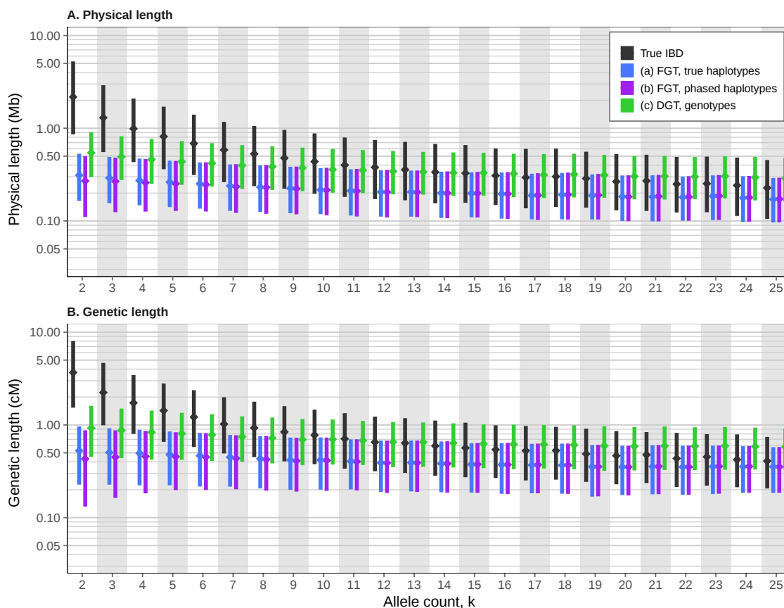
Figure 4.8: IBD length distribution using tidy after inclusion of genotype error. The distribution of physical (A) and genetic (B) segment length is shown by allele count ( f_k category). Results are shown for three approaches; (a) FGT on true haplotypes, (b) FGT on phased haplotypes, and (c) DGT on genotype data. Corresponding true lengths are shown in for comparison. Bottom and top of each bar indicate 1st and 3rd quartiles, respectively, between which the median (2nd quartile) is marked ( diamonds ).
