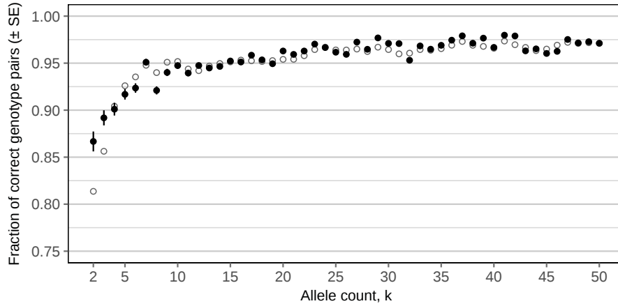
Figure 5.6: Initial state probability of discordant pairs in the genotype-based HMM. The proportion of discordant pairs that were correctly identified by their genotypes was empirically determined from data before and after the inclusion of realistic genotype error rates. The mean per f_k was used as the initial state probability of the HMM-based approach for IBD detection around target sites. For comparison, the initial state probability of concordant pairs is shown ( hollow circles ).
