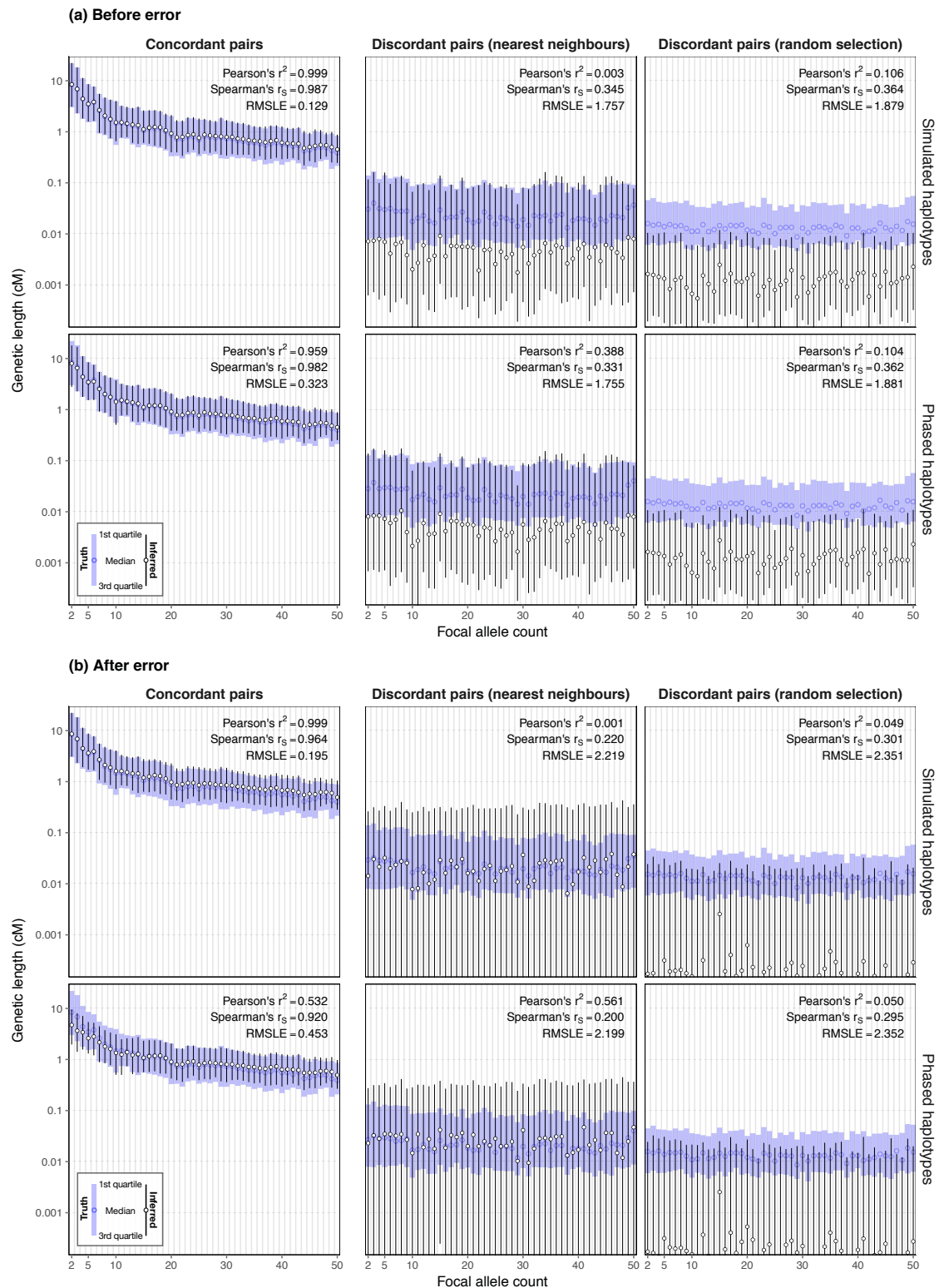
Figure 5.15: Genetic length of shared haplotype segments using the haplotype-based HMM. Inferred genetic length is shown by allele count of the focal variant in the simulated sample of N = 5,000 haplotypes, in direct comparison to the corresponding true segment lengths (blue). Pair selection was done using the relaxed nearest neighbour approach and at random. Note that concordant pairs were selected at random throughout. Results were obtained on data before (a) and after error (b), separately on simulated and phased haplotypes.
