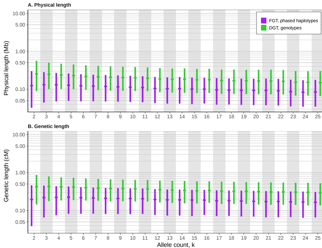
Figure 3.14: Distribution of inferred IBD lengths in 1000 Genomes data, chr. 20. Results are shown for the detected physical and genetic lengths of shared haplotype segments by f_k , using chromosome 20 in the final release dataset of 1000 Genomes Project Phase III, including N = 2,504 individuals. IBD segments were detected using the FGT (on phased haplotypes) and the DGT (on genotype data). Bottom and top of each bar represent the 1st and 3rd quartile, respectively, between which the median (2nd quartile) is marked ( diamonds ).
