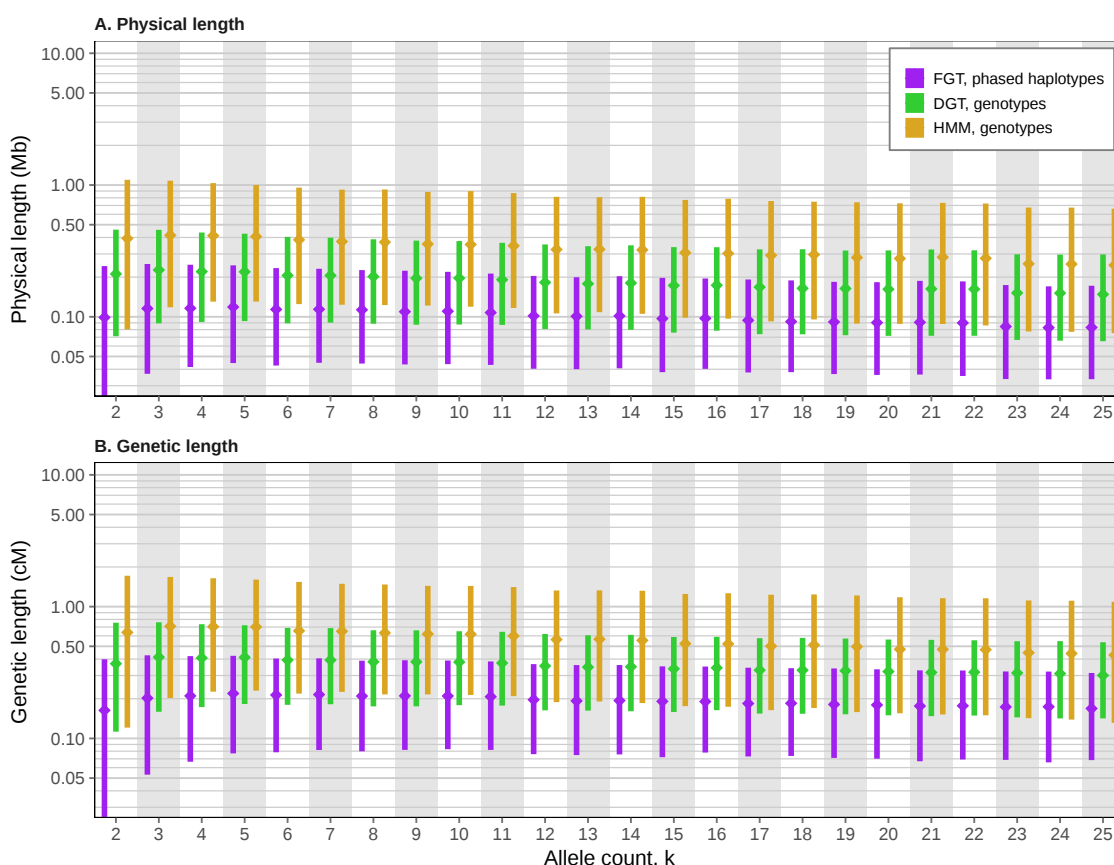
Figure 4.20: IBD inference using the HMM on 1000 Genomes data, chr. 20. IBD detection using the HMM-based method was performed under the empirical error model defined on genotype data from the 1000 Genomes Project. The resulting length distribution is compared to previous results obtained on the same set of target sites using the FGT and DGT. Bottom and top of each bar indicate 1st and 3rd quartiles, respectively, between which the median (2nd quartile) is marked ( diamonds ).
