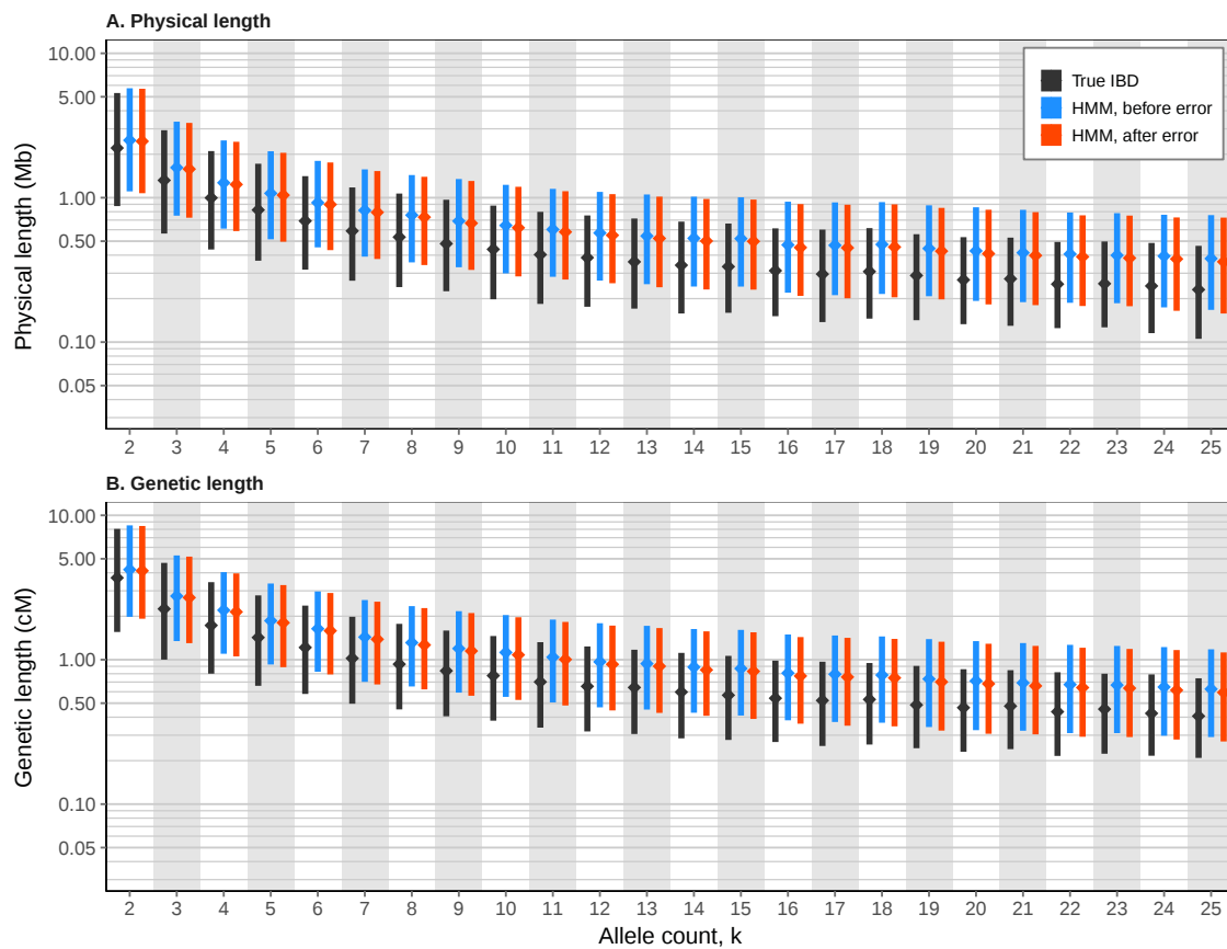
Figure 4.19: IBD lengths using the HMM before and after error. The HMM-based approach for targeted IBD detection was applied to simulated data before and after the integration of error; i.e. datasets D and D^* , respectively. Lengths were compared to the corresponding set of true breakpoint segments as determined from simulation records. Bottom and top of each bar indicate 1st and 3rd quartiles, respectively, between which the median (2nd quartile) is marked (diamonds).
