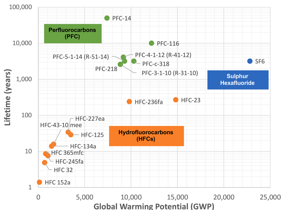
Fig. 1. Common f-gases types: Perfluorocarbons (PFCs, green), Sulphur Hexafluoride (SF 6 , blue) and Hydrofluorocarbons (HFCs, orange), their Global Warming Potential (GWP 100 , x-axis) and lifetime in the atmosphere (logarithmic scale on y-axis). (For interpretation of the references to colour in this figure legend, the reader is referred to the web version of this article.)
