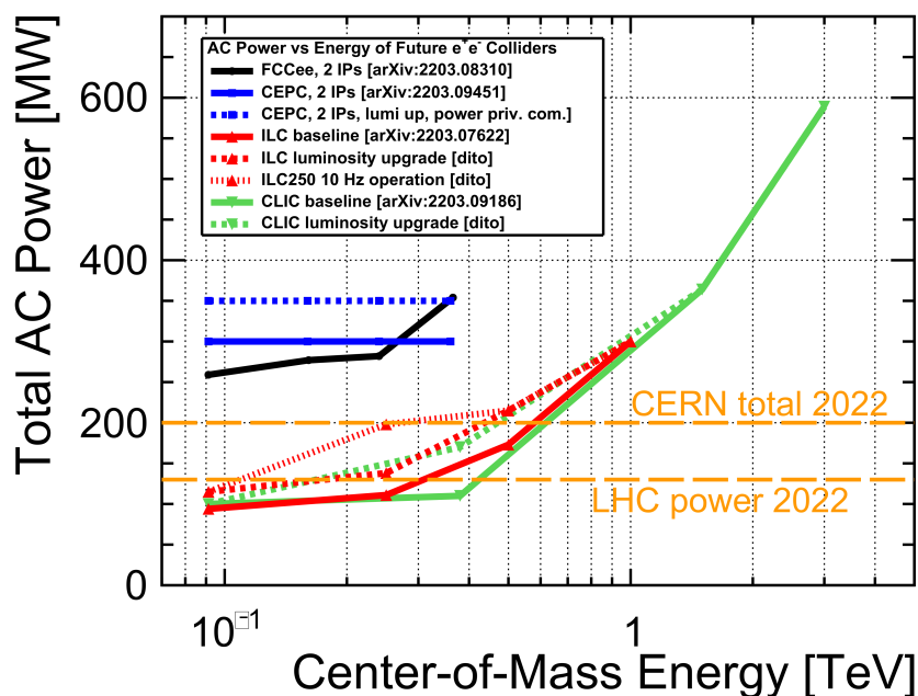
Figure 18. Site power required for proposed electron-positron ( e^+e^- ) collider projects at different center-of-mass energies, compared to the average power consumption of CERN and the LHC, during accelerator operation in 2022 [234, 235]. Reproduced with permission from Jenny List [236].
