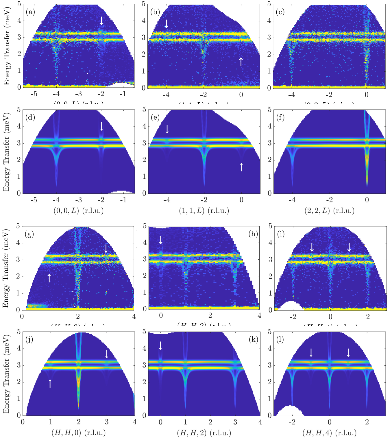
FIG. 8. Low-energy inelastic neutron scattering data collected on LET along several directions in reciprocal space, shown intercalated with the calculated spectra for the model Hamiltonian in Eq. (12). Panels (a)–(c) and (g)–(i) show experimental data, (d)–(f) and (j)–(l) correspond to calculated spectra using the Fe–Fe exchange model of Shamoto et al. [10]. White arrows denote points of interest in the hybridisation of the modes, reproduced very well by the model.
