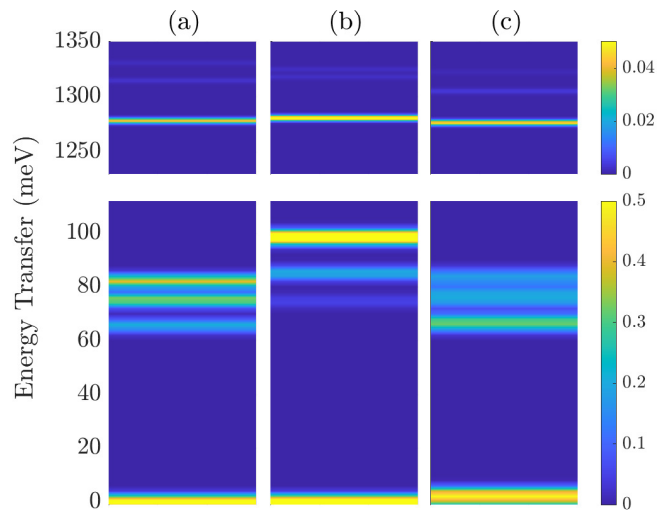
FIG. 7. Diagram representing energy levels and intensities at T = 5 K deduced for (a) Yb 3 Ga 5 O 12 and (b) Yb 3 Al 5 O 12 in Ref. 36. In (c) the best fit for Yb 3 Fe 5 O 12 obtained in this work is shown. The calculated intensities were convolved with a Gaussian with the instrumental resolution width. Note the different colour scale in the bottom and top panels. Intensities were calculated using the dipole approximation, and are rigorously correct only for \mathbf{Q} = 0 .
