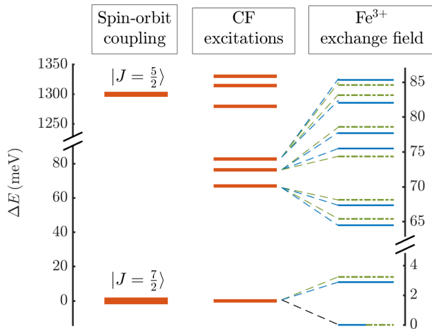
FIG. 2. Evolution of the single-ion \text{Yb}^{3+} spectrum in \text{YbIG} . In the absence of time-reversal symmetry breaking, all the CF levels are Kramers doublets. The exchange field caused by the magnetic ordering of the \text{Fe}^{3+} sublattice, as much as breaking the Kramers degeneracy, also splits the twelve rare-earth sites into two groups. On the right-hand side panel, the ground state multiplet ( |J = 7/2\rangle ) excitations for each of those two sites (continuous and dashed lines) are shown.
