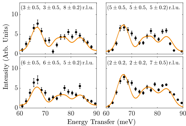
FIG. 6. Examples of experimental scattering from CF excitations (circles, with error bars), obtained following the procedure detailed in the text. The orange line corresponds to the best fit found in this work. The spectra are averaged over the range in \mathbf{Q} indicated in each panel.
