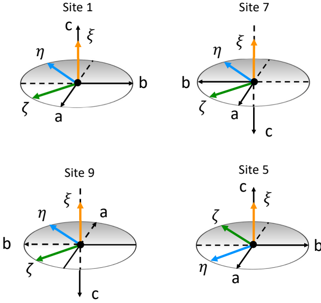
FIG. 11. Representation of local and global coordinate systems for atoms 1, 5, 7 and 9. Coordinates for the remaining 8 atoms in the primitive unit cell may be obtained by successive 3-fold rotations about the [111] direction.
