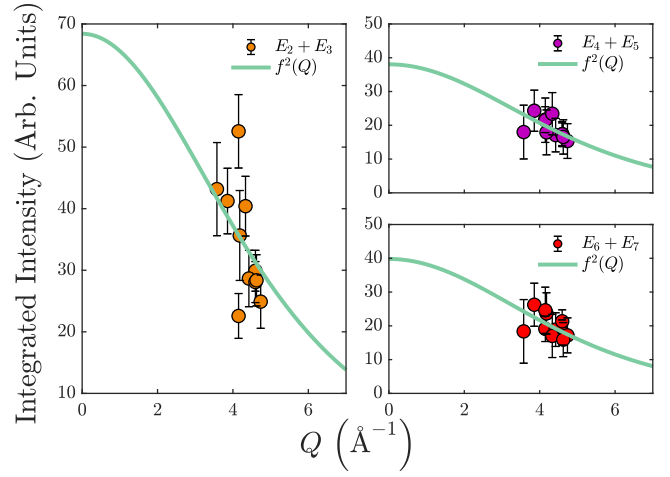
FIG. 13. Integrated intensities, obtained as detailed in the text, of the constant- \mathbf{Q} cuts performed on MAPS data.
