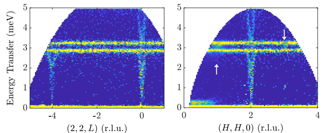
FIG. 4. Low-energy inelastic neutron scattering data measured on LET at 1.8 K showing the ground-state splitting of the CF excitations of the \text{Yb}^{3+} ions. White arrows on the right panel highlight regions where zero intensity dispersions of Fe magnons cross the CF levels.
