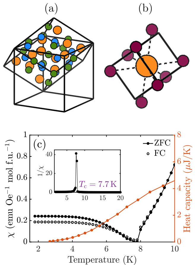
FIG. 1. (a) Garnet primitive unit cell, displayed within the conventional cubic vertices. Trivalent rare-earths are shown in orange, while green and blue circles correspond to \text{Fe}^{3+} at 24d and 16a positions, respectively. Oxygens are omitted in (a) for clarity. (b) Pseudocubic oxygen environment of the \text{Yb}^{3+} , as seen along one of the equivalent cubic \langle 001 \rangle directions. The point symmetry of the central atom is 222 . (c) Magnetic susceptibility \chi for \text{Yb}_3\text{Fe}_5\text{O}_{12} , measured in a magnetic field of 100\text{Oe} applied along the [110] direction. The compensation temperature T_c occurs at about 7.7\text{K} . Heat capacity data are plotted along with \chi in order to emphasise that the compensation temperature is not accompanied by a phase transition. The inset in (c) shows the inverse susceptibility over the same temperature interval, where the crossover at T_c can be more clearly seen.
