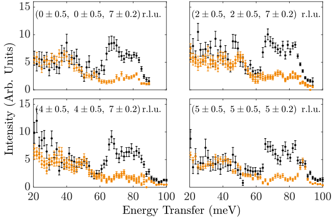
FIG. 12. Procedure used to separate scattering from crystal-field excitations from scattering due to optical Fe spin-wave modes and phonons. Data on \text{Y}_3\text{Fe}_5\text{O}_{12} (orange) were scaled to data on \text{Yb}_3\text{Fe}_5\text{O}_{12} (black), and subsequently subtracted from them. The resulting pattern, noticeably within the [60,90] meV energy interval, is attributed to the single-ion excitations of the rare-earth. Integration ranges are indicated at the top of each panel.
