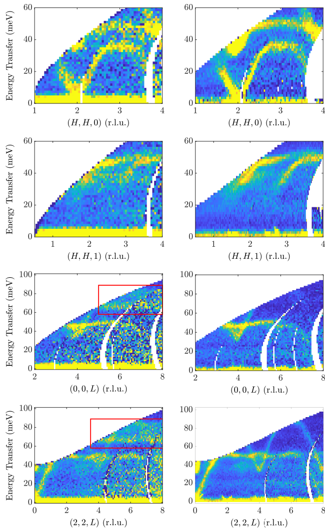
FIG. 3. Data measured on MAPS at \sim 6 K for \text{Yb}_3\text{Fe}_5\text{O}_{12} (left) and \text{Y}_3\text{Fe}_5\text{O}_{12} (right). Note the similarity between the dispersive Fe spin-wave modes in both compounds. Yb single-ion excitations in YbIG are highlighted by red rectangles in the lower left panels.
