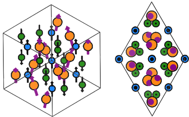
FIG. 10. Zero-temperature magnetic structure of \text{Yb}_3\text{Fe}_5\text{O}_{12} , shown down the [11\bar{1}] (left) and [111] (right) axes. The colour code is the same as that of Fig. 1(a). Arrows crossing Yb atoms point along the ground-state magnetic moment of \mathcal{H}_1 . Size of arrows does not indicate magnetic moment magnitude and is not represented in scale, being used only to denote spin orientation.
