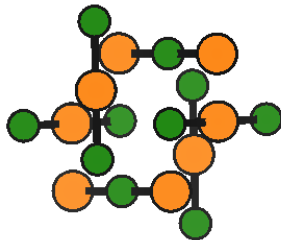
FIG. 5. Expanded view of the 24c (orange, Yb) and 24d (green, Fe) sublattices. Each Yb has two nearest neighbour Fe at 24d positions. Only bonding atoms are shown.
