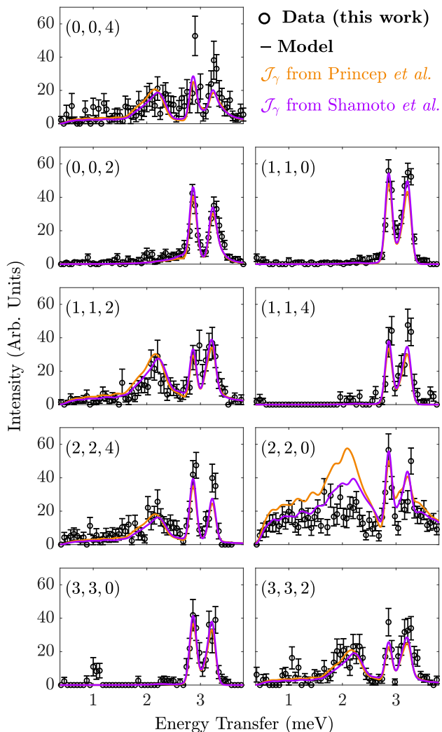
FIG. 9. Constant- \mathbf{Q} cuts (black circles, with error bars) performed on data shown in Fig. 8. Intensities were averaged over \pm 0.1 r.l.u. in all directions around the wavevector \mathbf{Q} shown in the panels. The colored lines are calculated from our model using the parameters given in Refs. 9 and 10, also listed in Table I.
