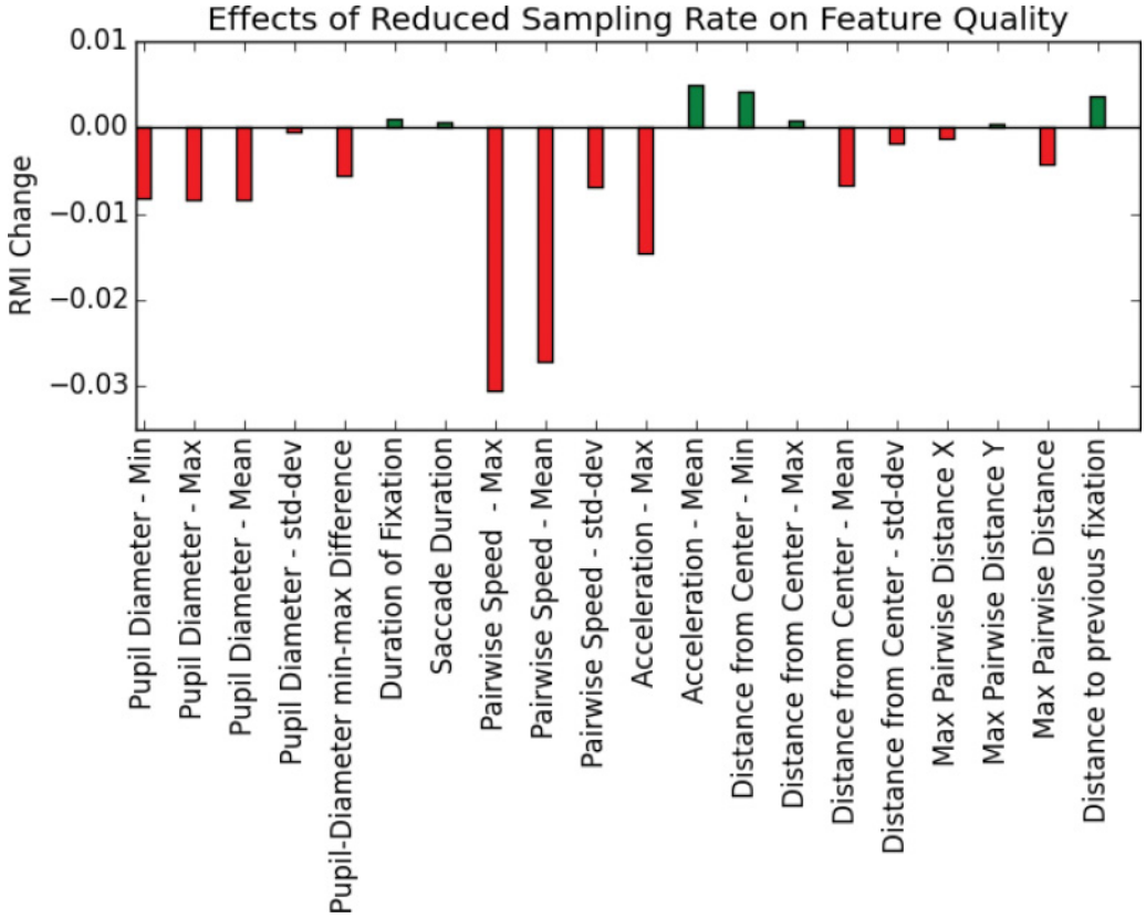
Fig. 11. Changes to the RMI of individual features when reducing the sampling rate to 50Hz. The temporal features reflecting the properties of microsaccades (speed and acceleration) are most strongly affected.
