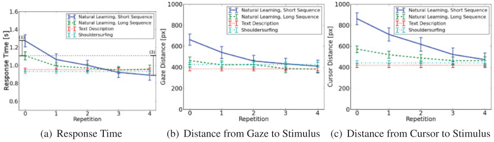
Fig. 14. Changes of three different performance metrics caused by natural learning, text descriptions, and shoulder surfing: (1) shows the effects of increased familiarity with game mechanics, and (2) shows the memory effects of learning a sequence. The error bars indicate the 95% confidence intervals.
