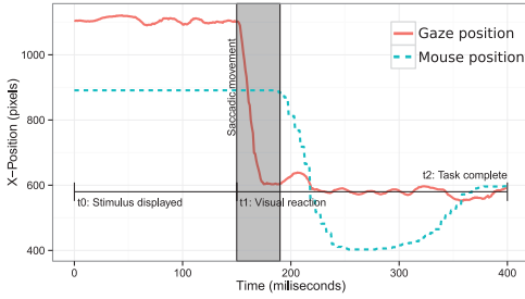
Fig. 4. At time t_0 a new dot appears followed by a period of inactivity (reaction time) in which neither the gaze nor the cursor moves significantly. After about 150ms, at t_1 , a visual reaction in the form of a large saccade occurs (the gray area) and the gaze and cursor converge to the position of the stimulus.
