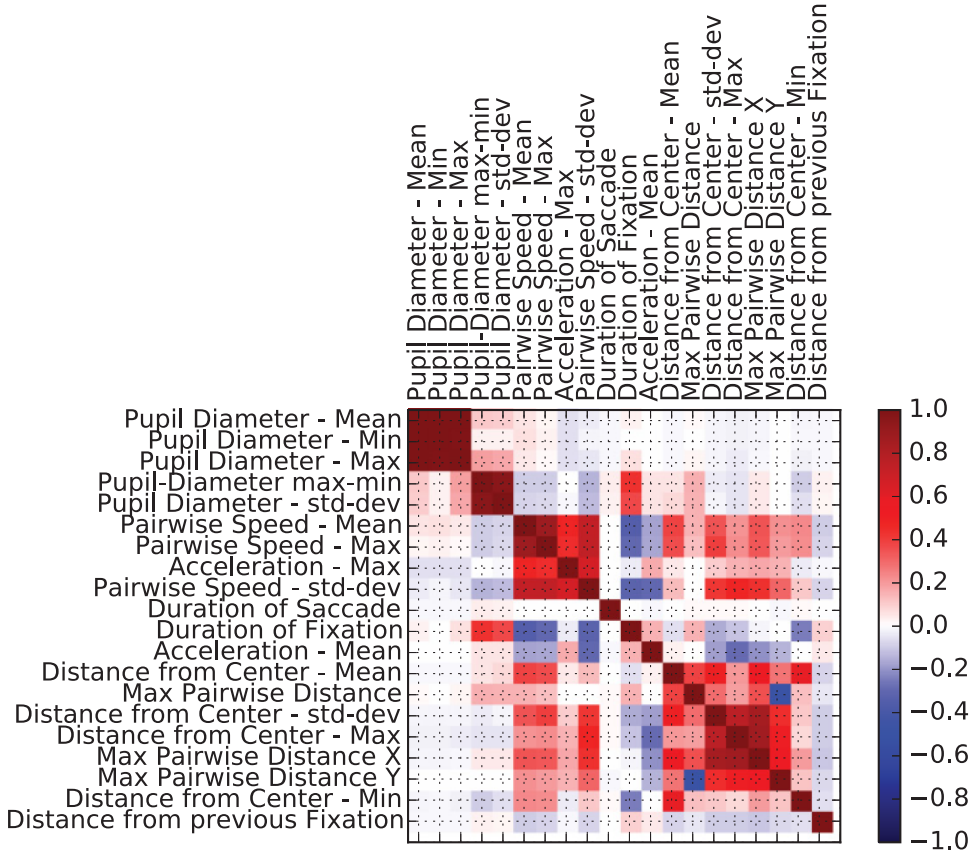
Fig. 8. Feature correlation measured by the Pearson correlation coefficient. A value of 0 indicates no correlation; values of 1 and -1 signify positive and negative correlation, respectively.
