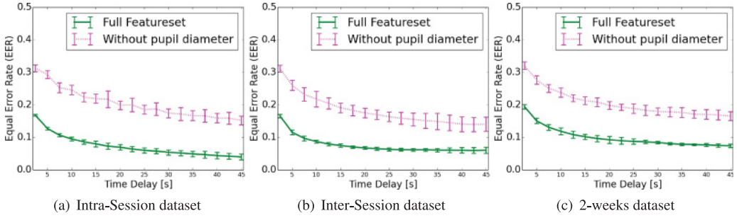
Fig. 12. Average equal error rates obtained through fivefold stratified cross-validation on three different datasets using the closed-set SVM classifier. The error bars indicate 95% confidence intervals.
