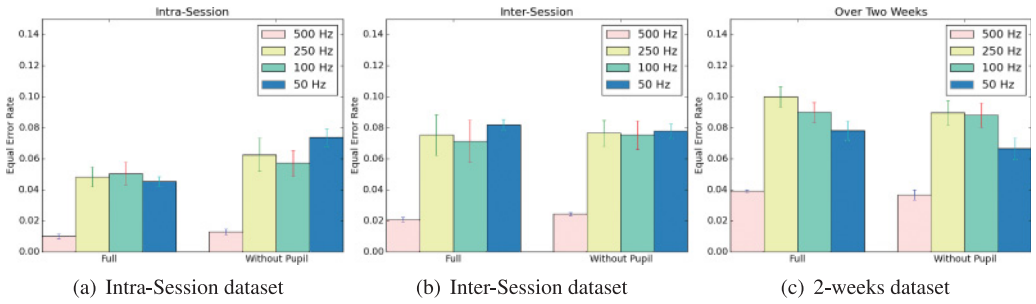
Fig. 13. Average equal error rates obtained with the one-class SVM classifier for different sampling rates. The error bars indicate 95% confidence intervals. Reducing the sampling rate to 250Hz has a large effect on the error rates; any subsequent reduction does not produce a statistically significant increase in the EER.
