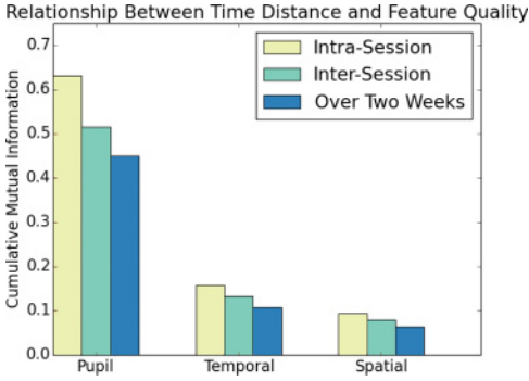
Fig. 9. Influence of data collection time span.
