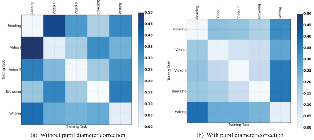
Fig. 16. Equal error rates for different combinations of training and testing tasks. The right figure uses the pupil diameter correction described in Section 8.3.1.
