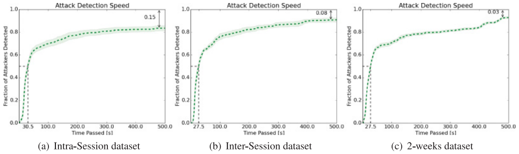
Fig. 15. Attack detection speed of the open-set classifier with parameter settings that never reject legitimate users. The dotted line represents the average, and the shaded area the 95% confidence interval over the five folds of the cross-validation. These results were obtained using the full feature set and sampling rate; see Table II for the remaining results.
