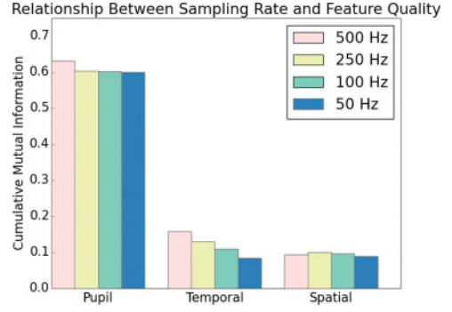
Fig. 10. Influence of sampling rate.
