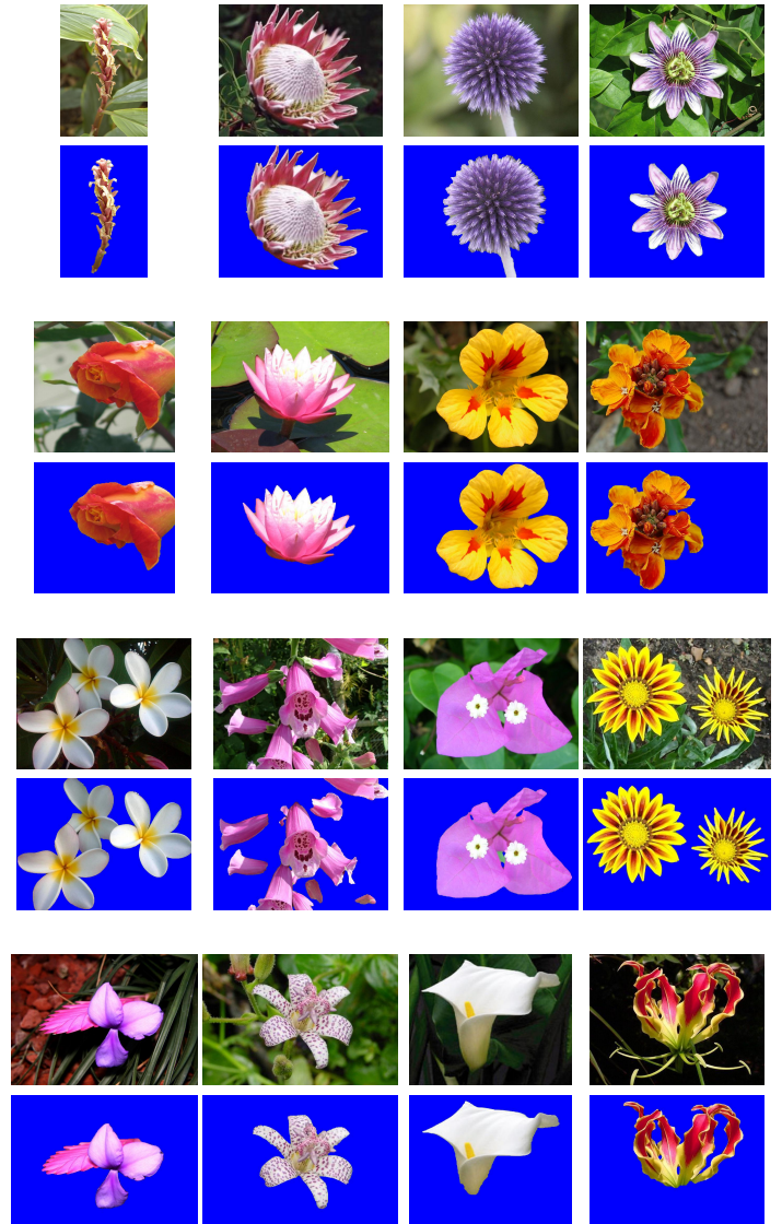
Figure 2: Example segmentations.
