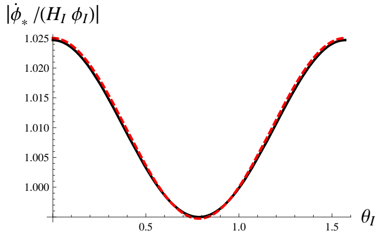
Figure 3.2: The angular dependence of the flat direction velocity |\dot{\phi}_*| at \phi_* (the minimum distance from the origin) plotted for a_{\text{osc}} = 0.003 and n = 4 in units of H_I|\phi_I| (see Appendix A). The numerical evaluation (with \beta = 0.1 and \lambda = 0.01 ) is represented by the continuous line, while the analytical estimate of Eq. (3.13) is dashed.
