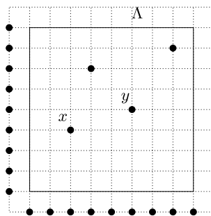
FIG. 2. A configuration \eta extended with maximal boundary conditions. The gap of the vacancies at x, y are: g_x(\eta) = 3 , g_y(\eta) = 4 .
