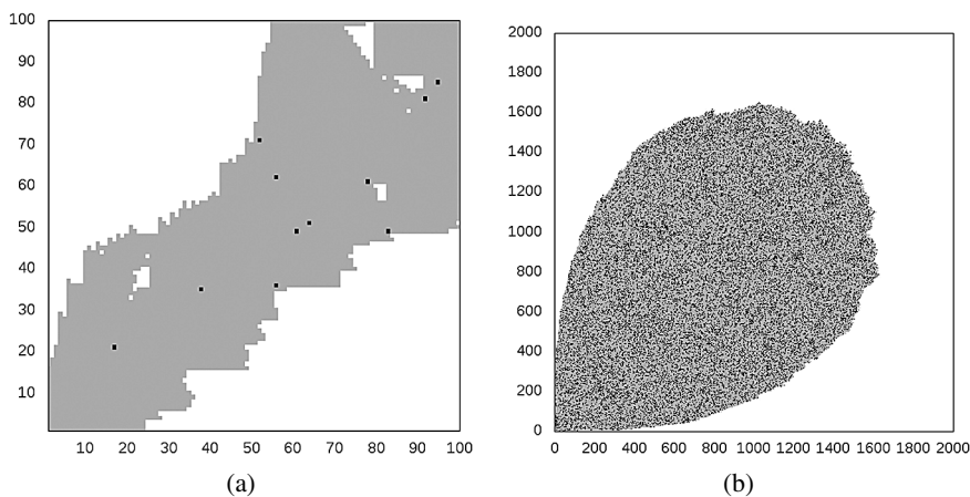
FIG. 1. A snapshot of a simulation of the East-like process with minimal boundary conditions and initial condition constantly identically equal to 1. White dots are vertices that have never been updated, grey dots correspond to vertices that have been updated at least once and the black dots are the vacancies present in the snapshot. (a) q = 0.002 , t = 3 \times 10^{12} ; (b) q = 0.25 , t = 9 \times 10^3 .
