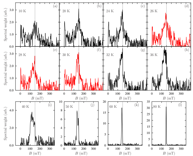
FIG. 2. Fourier transform \mu^+ SR spectra measured for a MnSi film in an applied field of B_{\text{app}} = 149 mT for muons implanted to the center of the MnSi layer in the film. The skyrmion A-phase region in the bulk is found between 26 \lesssim T \lesssim 30 K [spectra (d-f)]. Note the change of scale in panels (i-l).
