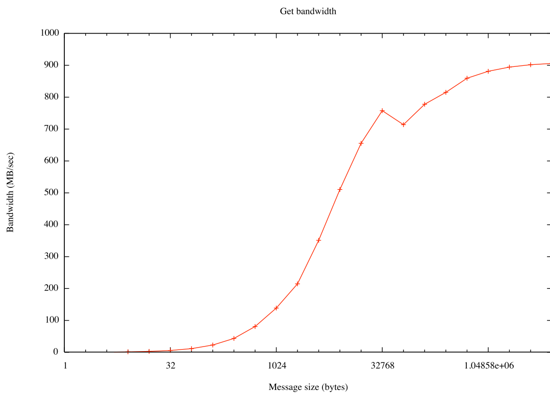
Figure 6.15: Get bandwidth between two nodes (OpenFabrics)
