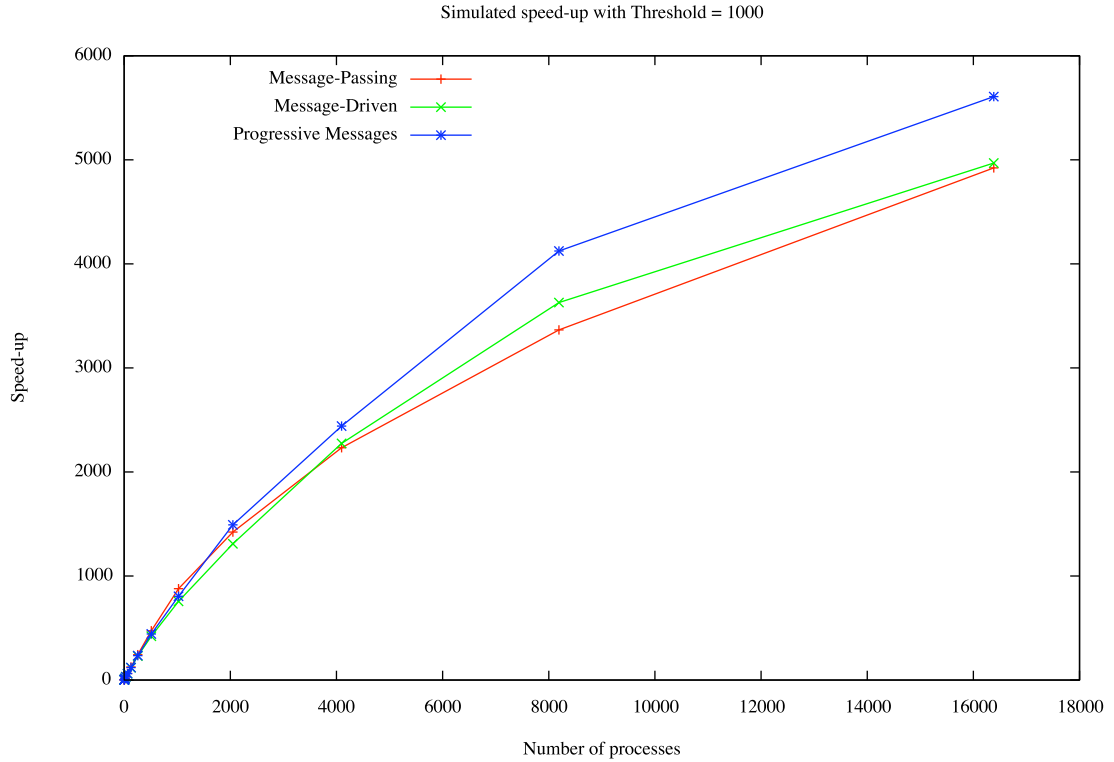
Figure 6.3: Speed-ups for when load-balancing threshold is 1000
