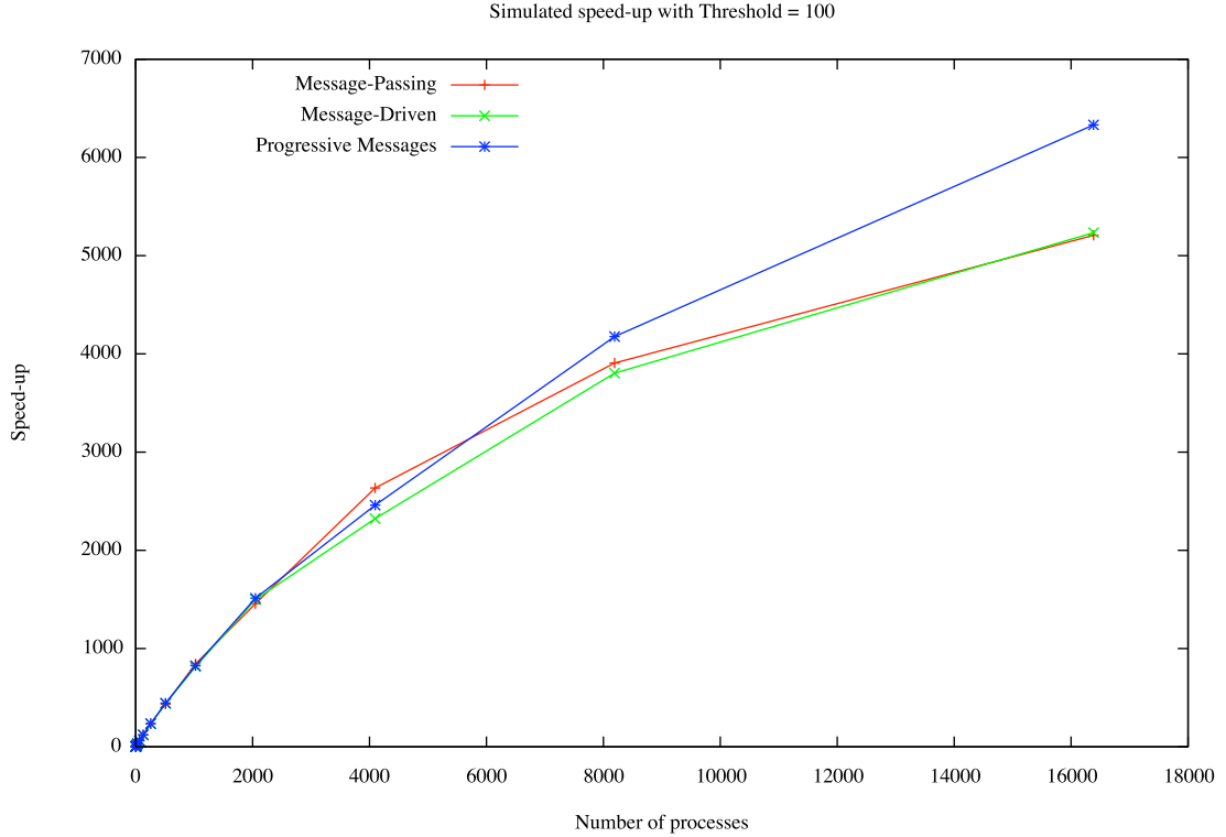
Figure 6.2: Speed-ups for when load-balancing threshold is 100
