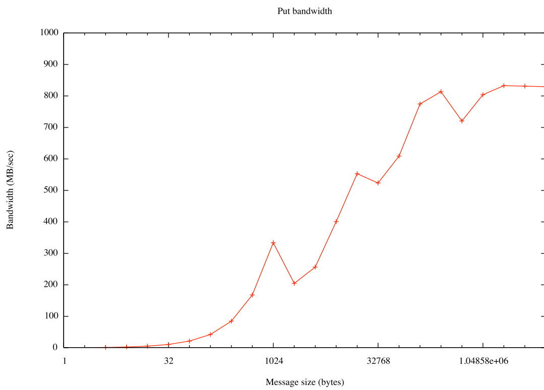
Figure 6.13: Put bandwidth between two nodes (OpenFabrics)
