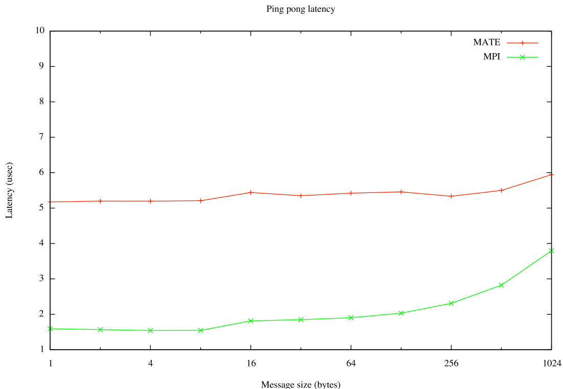
Figure 6.8: Ping pong latency between two nodes
