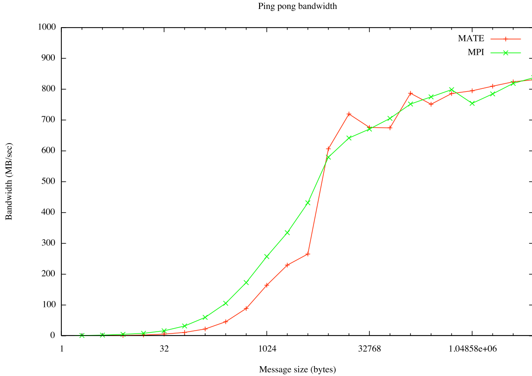
Figure 6.9: Ping pong bandwidth between two nodes
