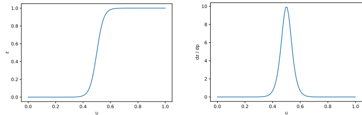
(a) Relation between \mathbf{z} \sim \text{Concrete}(p) and u \sim \text{Uniform}[0, 1] , given by a sigmoid function. (b) Derivative of \mathbf{z} w.r.t. the dropout parameter p .
