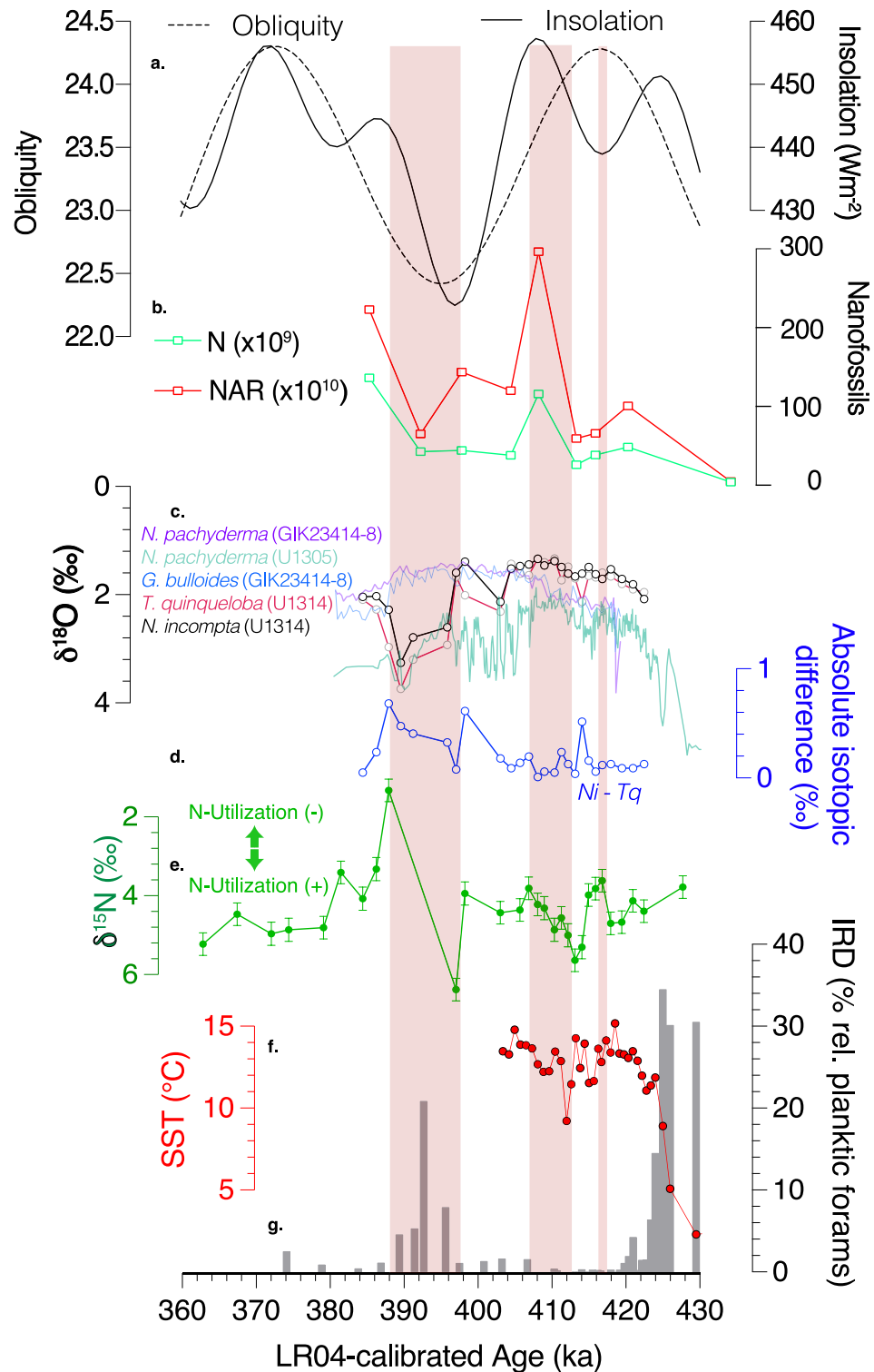
Figure 3. Results of coring site U1314. (a) Insolation at 65°N and obliquity (Berger & Loutre, 1991); (b) Relative changes in surface primary productivity at site U1314 from changes in nannofossil absolute concentration in sediments (N) and nannofossil accumulation rate (NAR; this study); (c) planktic \delta^{18}\text{O} values from sites U1314 (this study), U1305 (Irvah et al., 2020) and GIK23414-8 (Kandiano & Bauch, 2007); (d) Absolute difference in the \delta^{18}\text{O} composition between Neogloboquadrina incompta and Turborotalita quinqueloba (this study); (e) \delta^{15}\text{N} of N. incompta (this study); (f) Sea-surface temperature (SST) reconstructed via transfer functions (Alonso-Garcia, Sierro, Kucera, et al., 2011); and (g) Ice-rafted debris (IRD) % relative to planktic foraminifera from site U1314 (including data from Alonso-Garcia, Sierro, Kucera, et al., 2011). The red shaded areas highlight the three period of decrease in FB- \delta^{15}\text{N} (discussed in Section 3.2–3.4).
