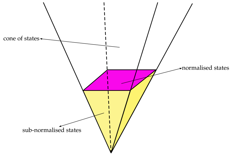
Figure 2.2: The cone of states of a causal theory. The set of normalised states (in purple) is given by the intersection of the hyperplane \text{tr } \xi = 1 , for \xi in \text{St}_R(A) , with the cone of states \text{St}_+(A) . Below that hyperplane are the sub-normalised states (in yellow). The coloured part in the cone of states is the set of states \text{St}(A) . The white part corresponds to super-normalised elements of \text{St}_+(A) , which are non-physical.
