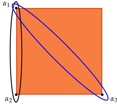
Figure 5.4: Normalised states of the square bit. The two sets \{\alpha_1, \alpha_2\} (circled in black) and \{\alpha_1, \alpha_3\} (circled in blue) consist of perfectly distinguishable pure states. Permutability holds, because every permutation of every pair of perfectly distinguishable pure states can be implemented by a reversible channel, corresponding to a symmetry of the square. However, no reversible channel can transform \alpha_2 into \alpha_3 while leaving \alpha_1 unchanged. Hence, Strong Symmetry cannot hold for the square bit.
