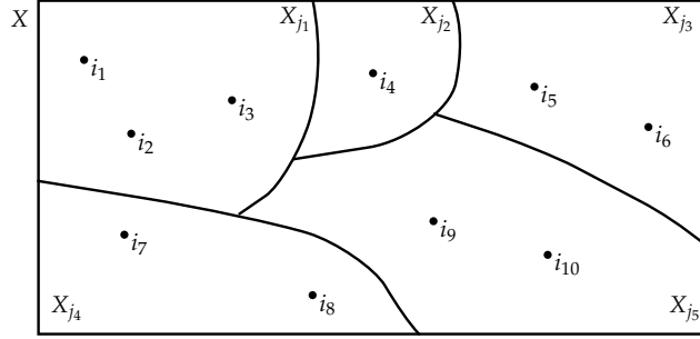
Figure 2.1: The outcome set X of the test \{\mathcal{A}_i\}_{i \in X} has 10 outcomes. To perform a coarse-graining of it, we lump together some of its outcomes, relabelling them as a new outcome. For example, the outcomes i_1 , i_2 , and i_3 are relabelled as j_1 . This gives rise to a partition \{X_j\}_{j \in Y} of X . We associate a new transformation with each set in the partition, such that it is the sum of the transformations associated with the outcomes contained in that set. Thus \mathcal{B}_{j_1} = \mathcal{A}_{i_1} + \mathcal{A}_{i_2} + \mathcal{A}_{i_3} . The new test \{\mathcal{B}_j\}_{j \in Y} has 5 outcomes.
