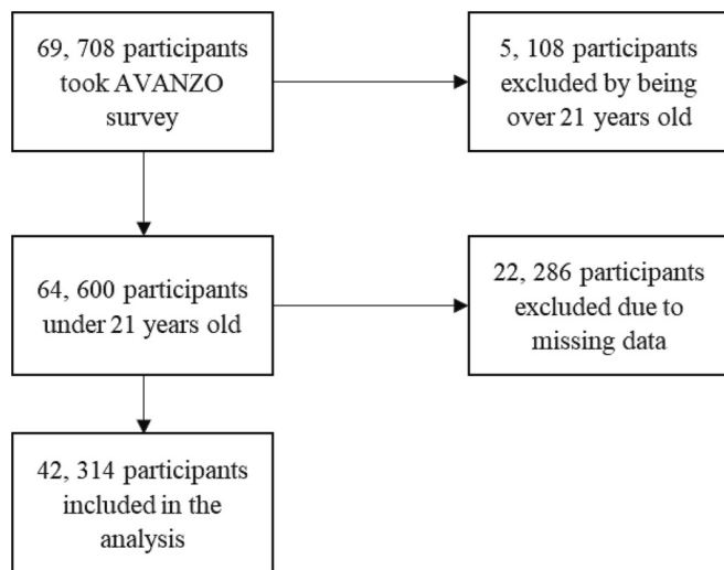
Fig. 1. Flow-chart selection of participants in the analytical sample.
