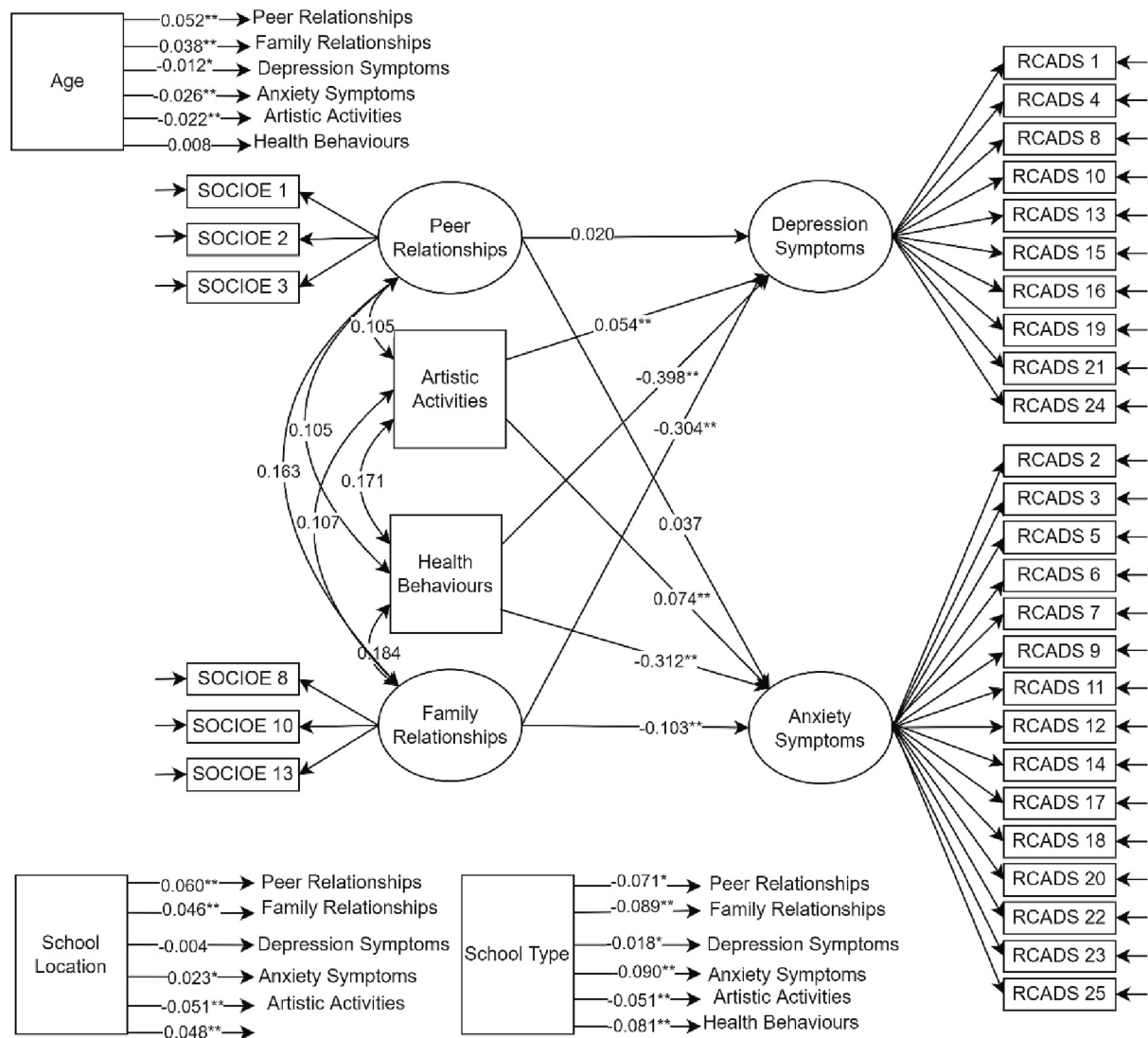
Fig. 2. SEM diagram of model 4 with standardized regression path estimates. Note: ** p < .001 , * p < .05 . The type of school was coded as 1 (public) and 2 (private), and the type of school location was coded as 1 (urban) and 2 (rural).
