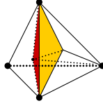
FIGURE 1. The Worsey-Farin split of a tetrahedron (relative to one face)
