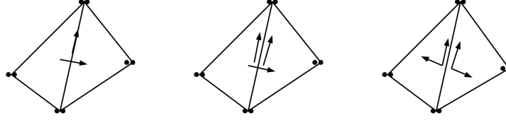
FIGURE 2. Continuous, partially discontinuous elements, and discontinuous. Left: vector-valued Lagrange elements. Both the tangential and the normal components are continuous across edges. Middle: partially discontinuous nodal elements for H(\text{div}) (Stenberg element). The normal component is continuous while the tangential component is discontinuous in general. Right: discontinuous elements. Both tangential and normal components are discontinuous in general.
