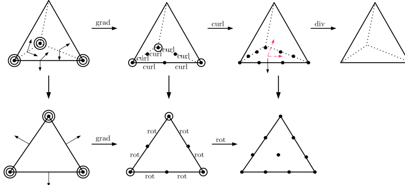
FIGURE 5. The complex containing the 3D H(\text{div}) nodal element and its 2D restriction. For H(\text{rot})/H(\text{curl})/H(\text{div}) elements, a dot \bullet represents the evaluation of the vector valued function, which counts as two/three degrees of freedom. In the 3D H(\text{div}) element, the two red dashed lines indicate the two tangential components associated with the Lagrange point on the face. They are regarded as interior degrees of freedom, which do not contribute to inter-element continuity.
