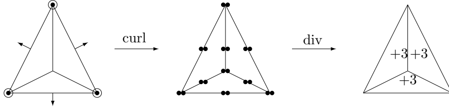
FIGURE 3. Clough-Tocher complex with discontinuous pressure. The figure shows the lowest order case: the first space is piecewise cubic, the second is continuous piecewise quadratic and the third is piecewise linear.
