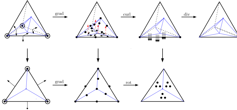
FIGURE 4. The complex containing the 3D H(\text{curl}) nodal element and its 2D restriction. For H(\text{rot})/H(\text{curl})/H(\text{div}) elements, a dot \bullet represents the evaluation of the vector-valued function, which counts as two/three degrees of freedom. In the 3D H(\text{curl}) element, the four red dashed lines indicate the normal components associated with the four Lagrange points on the face. They are counted as interior degrees of freedom and do not yield inter-element continuity.
