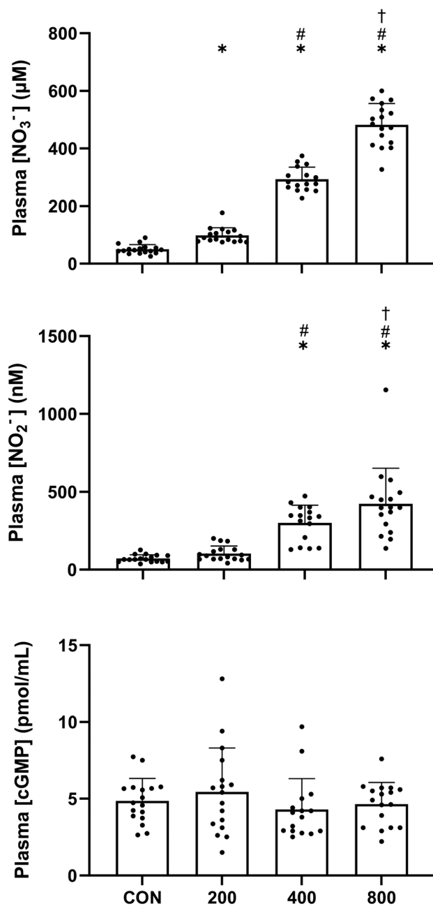
Fig. 2 Plasma nitrate ( [\text{NO}_3^-] ), nitrite ( [\text{NO}_2^-] ), and cyclic guanosine monophosphate ( [\text{cGMP}] ) concentrations following four conditions: no supplement (CON), and \text{NO}_3^- -rich beetroot powder providing 200 mg (200), 400 mg (400) or 800 mg (800) \text{NO}_3^- . The bars represent the group mean \pm SD responses with the filled circles representing individual participants. * denotes significantly different from CON ( P < 0.05 ). # denotes significantly different from 200 ( P < 0.05 ). † denotes significantly different from 400 ( P < 0.05 ).
