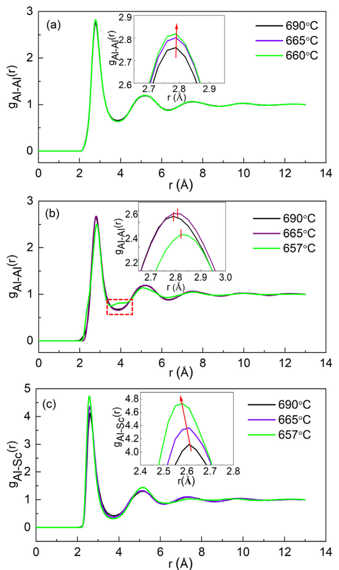
Fig. 3. (a) The PDFs of the Al-Al pair obtained from the EPSR modelling in pure liquid Al at different temperatures. (b) The partial PDFs of the Al-Al pair and (c) Al-Sc pair in the Al-0.4Sc melt at different temperatures.
