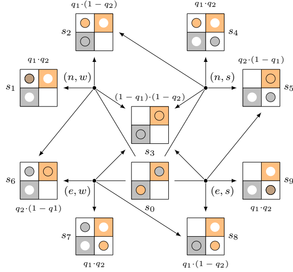
Figure 4.5: Concurrent example of two robots moving over a grid. ■
