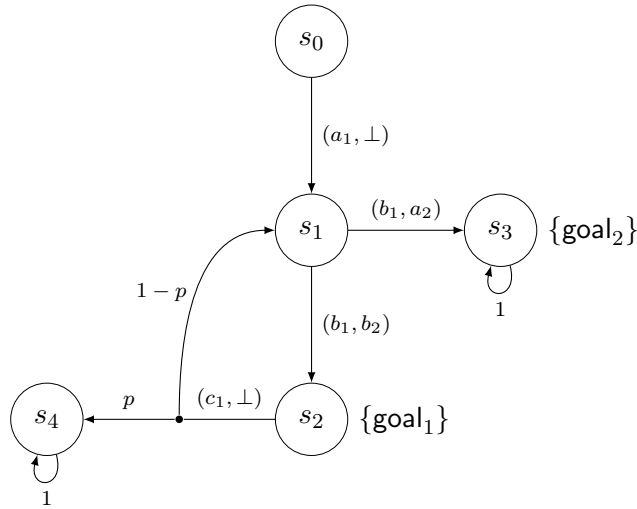
Figure 5.4: CSG example where memory may be required for synthesising an optimal strategy ( 0 < p < 1. ).
