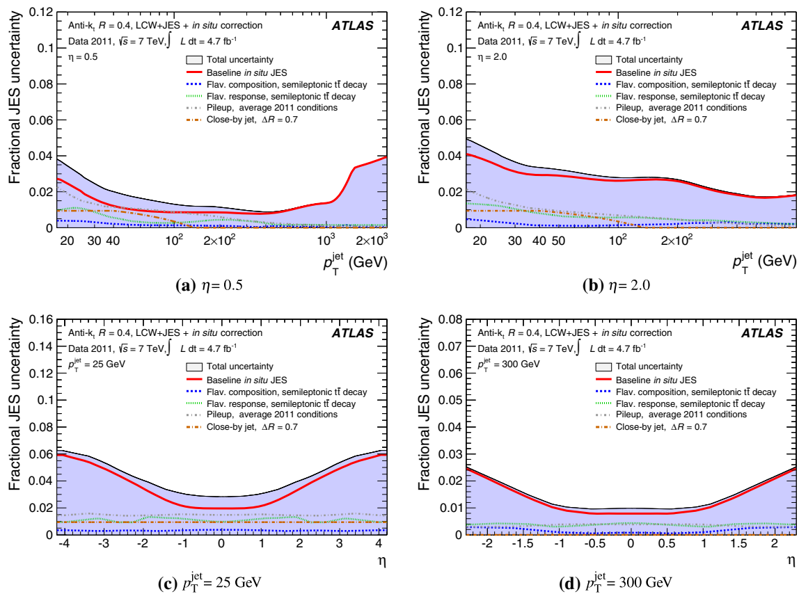
Fig. 62 Sample-dependent fractional jet energy scale systematic uncertainty as a function of a, b p_T^{\text{jet}} and c, d jet pseudorapidity for anti- k_t jets with distance parameter of R = 0.4 calibrated using
