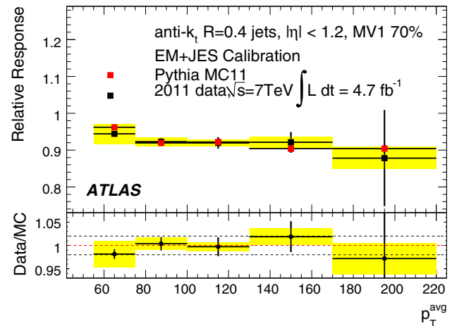
Fig. 57 Relative response of the semileptonic sample with respect to the inclusive b -jet sample as calculated from the dijet p_T asymmetry. The uncertainty band around the data denotes systematic uncertainties in the asymmetry measurement
