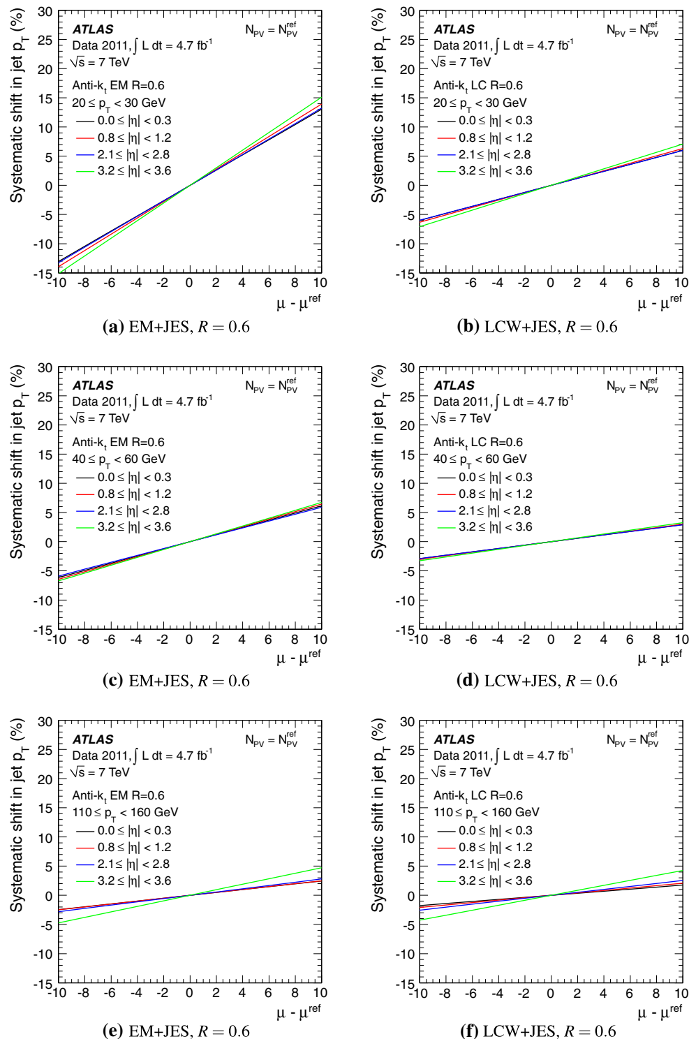
Fig. 49 The fractional systematic shift due to mis-modelling of the effect of out-of-time pile-up on the transverse momentum p_{T, \text{EM+JES}}^{\text{jet}} of jets reconstructed with the anti- k_t algorithm with R = 0.6 and calibrated with the EM+JES scheme, is shown as a function of (\mu - \mu^{\text{ref}})
