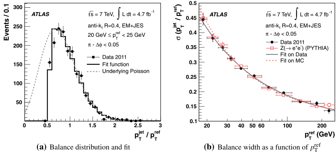
Fig. 15 The p_T^{\text{jet}}/p_T^{\text{ref}} distribution in the data for 20 \leq p_T^{\text{ref}} < 25 GeV and \pi - \Delta\phi(\text{jet}, Z) < 0.05 is shown in a . The black solid histogram represents the fit function, a Poisson distribution extended to non-integer values, multiplied by a turn-on curve. The value used in each bin is the mean value of that function in the bin. The gray dashed line shows the underlying Poisson distribution, from which the mean is taken as
