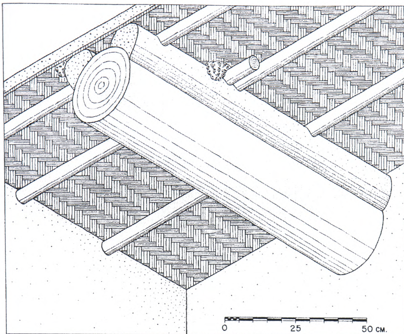
ISOMETRIC DRAWING OF THE RESTORED CEILING OF ROOM L. 43:9, SHOWING DETAILS INDICATED BY REMAINS FOUND IN THE ROOM. SCALE, 1:10
