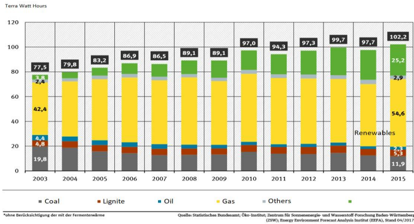
Figures 8 and 9: Electricity and Heat Produced in CHP Plants in Germany in Twh
