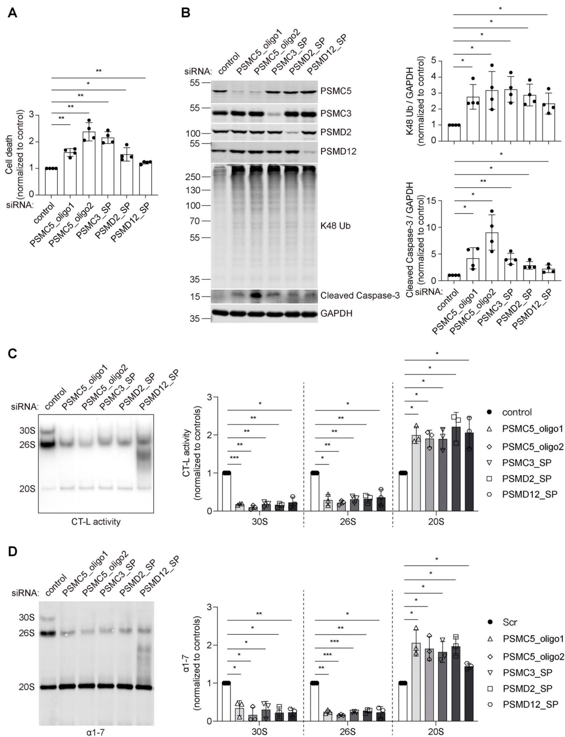
Figure 2. Knockdowns of the 19S RP subunits of the 26S proteasome impairs proteasome function and leads to apoptosis in HeLa cells. (A) LDH cytotoxicity assay to measure cell death caused by PSMC5, PSMC3, PSMD2, or PSMD12 siRNA knockdown. Plots represent mean \pm SD ( n = 4 independent experiments). P values were calculated using two-tailed, paired Student's t -test. (B) Western blotting of PSMC5, PSMC3, PSMD2, PSMD12, K48-ubiquitinated proteins, and cleaved caspase-3 levels, and quantification of K48-ubiquitinated proteins and cleaved caspase-3 in PSMC5, PSMC3, PSMD2, or PSMD12-knockdown cells. GAPDH served as protein loading control. Plots represent mean \pm SD ( n = 4 independent experiments). P values were calculated using two-tailed, paired Student's t -test. (C) In-gel proteasome chymotrypsin-like (CT-L) activity of the 30S, 26S, and 20S proteasome complexes and quantification thereof in PSMC5, PSMC3, PSMD2, or PSMD12-knockdown cells. The CT-L activity of proteasome complexes is visualized by their ability to cleave the Suc-LLVY-AMC fluorogenic peptide. The CT-L activity of the 30S, 26S, and 20S proteasome complexes of different knockdowns was normalized to the corresponding controls in the quantification plots. Plots represent mean \pm SD ( n = 3 independent experiments). P values were calculated using two-tailed, paired Student's t -test. (D) Immunoblotting of the native gel in (C) and probing of the membrane with anti- \alpha 1-7 antibody and quantification the amount of 30S, 26S, and 20S proteasome complexes indicated by \alpha 1-7. The protein level of \alpha 1-7 in the 30S, 26S, and 20S proteasome complexes of different knockdowns was normalized to the corresponding controls in the quantification plots. Plots represent mean \pm SD ( n = 3 independent experiments). P values were calculated using two-tailed, paired Student's t -test. * indicates P < 0.05 ; ** indicates P < 0.01 ; *** indicates P < 0.001 ; NS, not significant.
