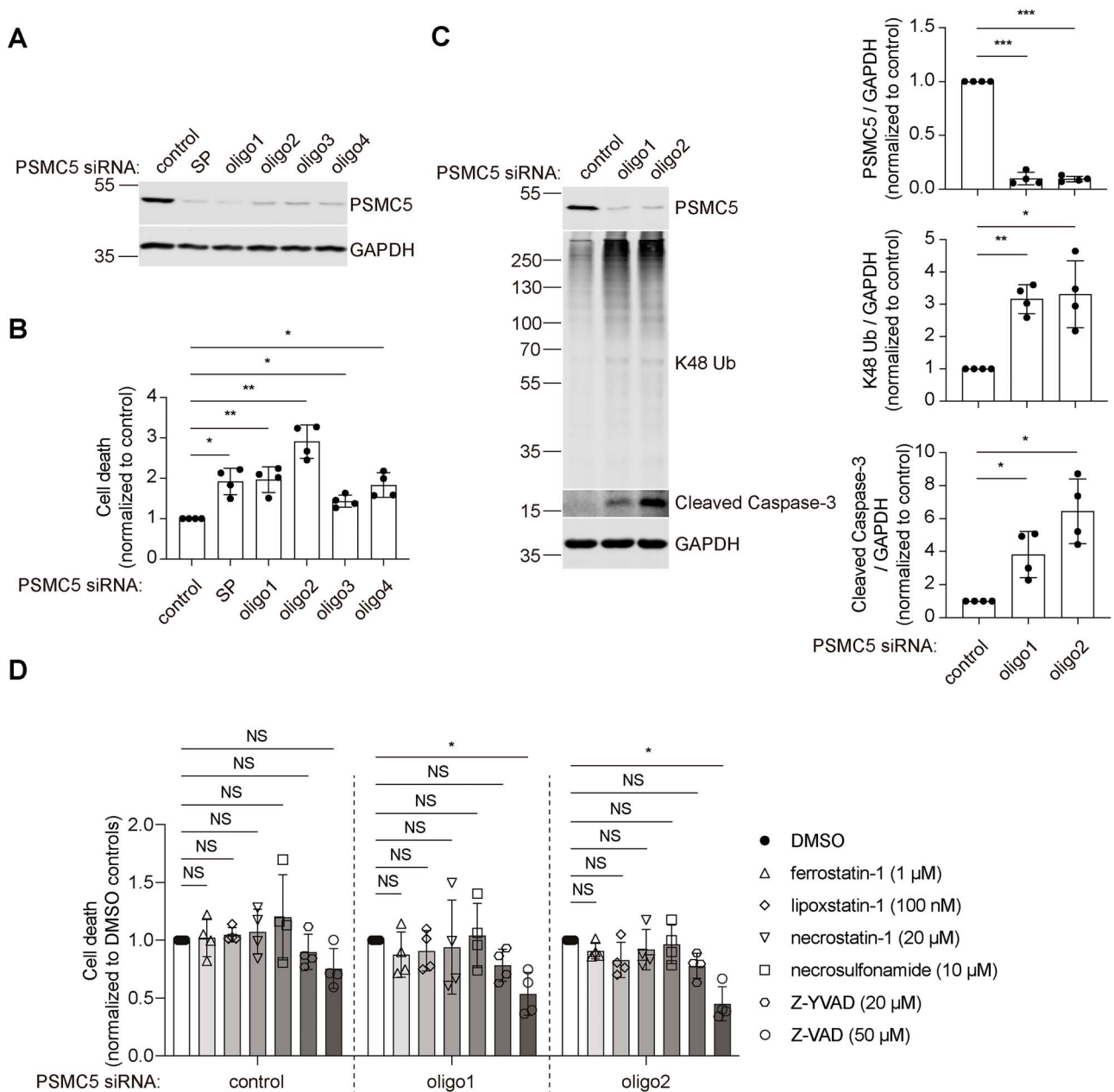
Figure 1. PSMC5 knockdown results in accumulation of K48-ubiquitinated proteins and apoptotic cell death in HeLa cells. (A) Western blotting of PSMC5 levels after PSMC5 siRNA knockdown using SMARTpool or four deconvoluted oligos. GAPDH served as protein loading control. (B) LDH cytotoxicity assay to measure cell death caused by PSMC5 knockdown. Plots represent mean \pm SD ( n = 4 independent experiments). P values were calculated using two-tailed, paired Student's t -test. (C) Western blotting and quantification of PSMC5, K48-ubiquitinated proteins, and cleaved caspase-3 levels in PSMC5-knockdown cells. GAPDH served as protein loading control. Plots represent mean \pm SD ( n = 4 independent experiments). P values were calculated using two-tailed, paired Student's t -test. (D) LDH cytotoxicity assay to measure the inhibition effect of ferroptosis inhibitors (ferrostatin-1, lipoxstatin-1), necroptosis inhibitors (necrostatin-1, necrosulfonamide), pyroptosis inhibitor (Z-YVAD), and apoptosis inhibitor (Z-VAD) on cell death caused by PSMC5 knockdown. Cell death of drug treatment groups was normalized to DMSO treated wild-type, PSMC5 knockdown with oligo1 or oligo2, respectively. Plots represent mean \pm SD ( n = 4 independent experiments). P values were calculated using one-way ANOVA with post-hoc Dunnett's multiple comparison test. * indicates P < 0.05 ; ** indicates P < 0.01 ; *** indicates P < 0.001 ; NS, not significant.
