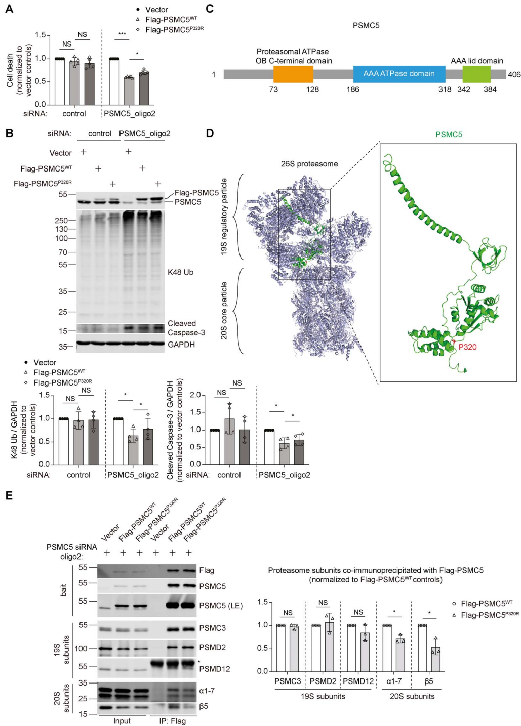
Figure 3. Transient expression of PSMC5 P320R in PSMC5-knockdown HeLa cells leads to the dissociation of the 19S RP from the 20S CP. (A) LDH cytotoxicity assay to compare cell death in PSMC5-knockdown HeLa cells transiently expressing Flag-PSMC5 WT or PSMC5 P320R . Cell death of control and PSMC5 knockdown groups was normalized to the corresponding vector groups, respectively. Plots represent mean ± SD (n = 5 independent experiments). P values were calculated using two-tailed, paired Student's t-test. (B) Western blotting of PSMC5, K48-ubiquitinated proteins, and cleaved caspase-3 levels and quantification of K48-ubiquitinated proteins, and cleaved caspase-3 in PSMC5-knockdown HeLa cells transiently expressing Flag-PSMC5 WT or PSMC5 P320R . GAPDH served as protein loading control. The protein levels of K48-ubiquitinated proteins and cleaved caspase-3 were normalized to the corresponding vector groups in the quantification plots. Plots represent mean ± SD (n = 4 independent experiments). P values were calculated using two-tailed, paired Student's t-test. (C) Domain organization of PSMC5. (D) The structure of 26S proteasome and PSMC5 are shown as ribbon diagrams with PSMC5 highlighted in green and PSMC5 P320 highlighted in red. The ribbon diagrams were generated using PyMOL software based on the solved structure of the human 26S proteasome (PDB 6MSH) [34]. (E) Immunoprecipitation of exogenously expressed Flag-PSMC5 WT or PSMC5 P320R in PSMC5-knockdown HeLa cells and quantification of the 19S RP and 20S CP subunits co-immunoprecipitated with Flag-PSMC5 WT or PSMC5 P320R . PSMC5 (LE) indicates a longer exposure of the PSMC5 blot. * in the blots indicates non-specific bands. The amount of all the preys (PSMC3, PSMD2, PSMD12, α1-7, and β5) co-immunoprecipitated with Flag-PSMC5 was normalized to the corresponding bait Flag-PSMC5 and then normalized to the corresponding Flag-PSMC5 WT groups in the quantification plots. Plots represent mean ± SD (n = 3 independent experiments). P values were calculated using two-tailed, paired Student's t-test. * indicates P < 0.05; ** indicates P < 0.01; NS, not significant. Endogenous PSMC5 is knocked down using PSMC5 siRNA oligo2 and exogenously expressed PSMC5 WT or PSMC5 P320R are PSMC5 siRNA oligo2-resistant.
