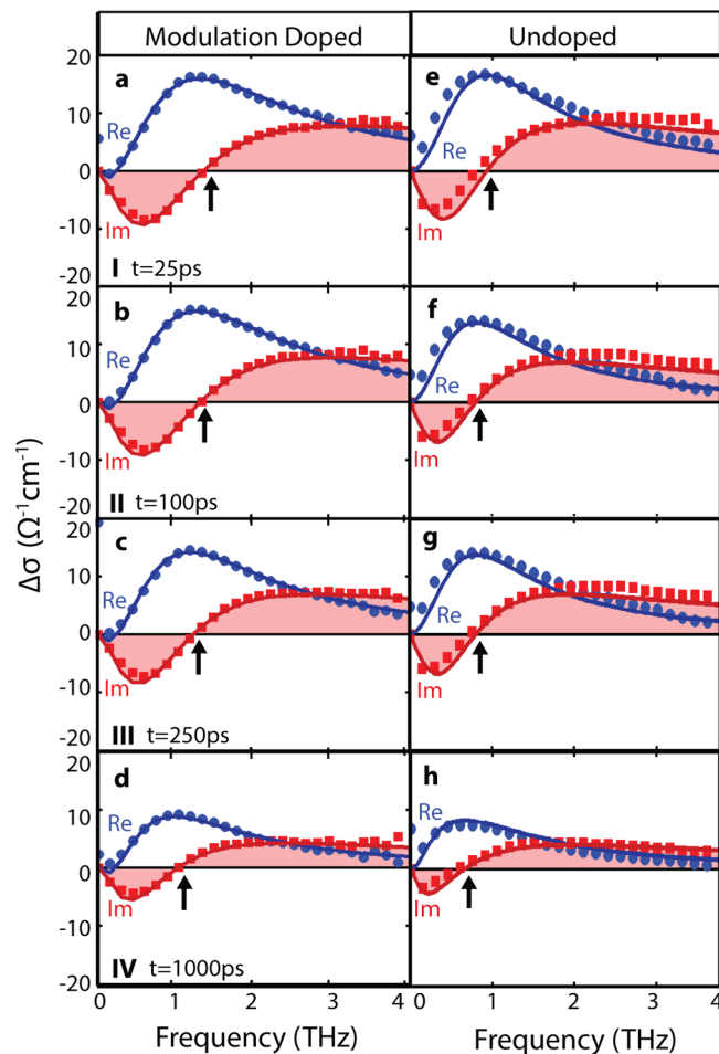
Figure 3. Time-resolved conductivity of photoexcited electrons for the n-type, modulation doped sample at times (a) 25, (b) 100, (c) 250, and (d) 1000 ps after photoexcitation and for the undoped sample at times (e) 25, (f) 100, (g) 250, and (h) 1000 ps after photoexcitation. Panels a–d correspond to times I, II, III, and IV shown in Figure 2. The incident pump pulse excitation fluence was 114 \mu\text{J}/\text{cm}^2 for both samples. The symbols represent the measured data and the solid lines the fitted plasmon responses. The real (blue) and imaginary (red) components of the conductivity are plotted with arrows indicating the resonant surface plasmon frequency, \omega_0 , for each spectrum. All measurements were performed at room temperature.
