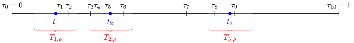
Figure 2: Example of \{\tau_l\}_{l=1}^m that satisfy the conditions in Definition 9 for m = 10 and k = 3.
