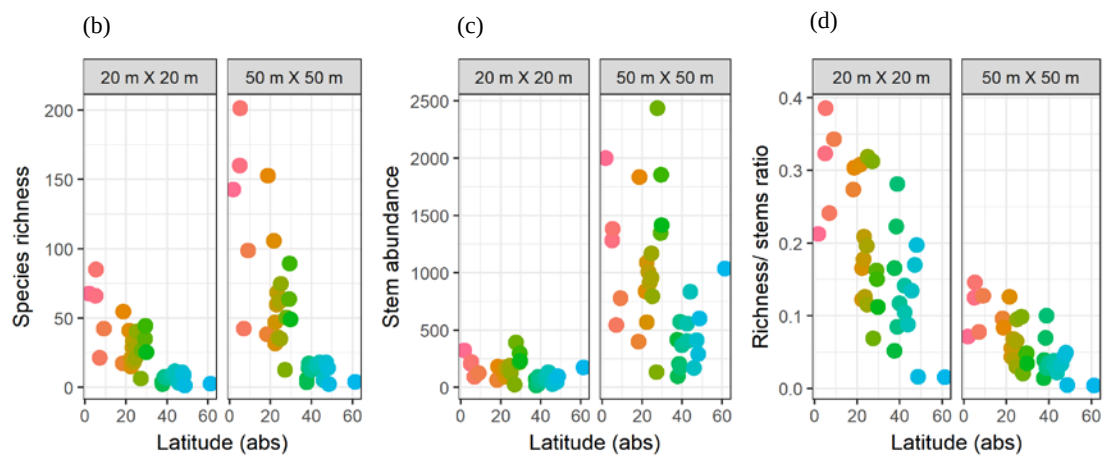
Figure 2 Global distribution of 35 forest dynamics plots used in this study (a), and the latitudinal gradients of tree species richness (b), stem abundance (c), and species richness/ stand stem ratios (d). Richness and stem abundance measured at plot scales of 20 m × 20 m and 50 m × 50 m. Descriptions of each site can be found in the Supplementary Information Table 1. Colors indicate increasing absolute latitude from pink to turquoise.
