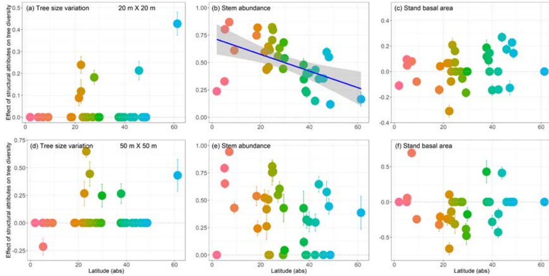
Figure 4 The effects of forest structural attributes on tree diversity derived from the within-forest plot SEM analyses. Panels a , b , and c at the scale of 20 m × 20 m, and panels d , e , and f at the scale of 50 m × 50 m. The effect of stem abundance on tree species richness showed a significant latitudinal trend at the scale of 20 m × 20 m (panel b ; P < 0.01 , R^2 = 0.27 ). Standardized path coefficients \pm 1 SE are shown; SE's are smaller than the size of the symbol for some forest plots. Colors indicate increasing absolute latitude from pink to turquoise.
