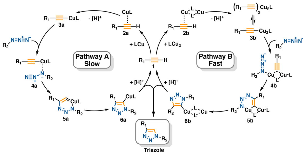
Scheme 1. Two Competitive Pathways for the Cu(I)-Catalyzed Azide–Alkyne Cycloaddition (CuAAC): A Slow Process Catalyzed by a Mononuclear Cu Species (Pathway A) and a More Kinetically Favored Route Promoted by the Formation of a Dinuclear Cu Catalyst (Pathway B) 37
