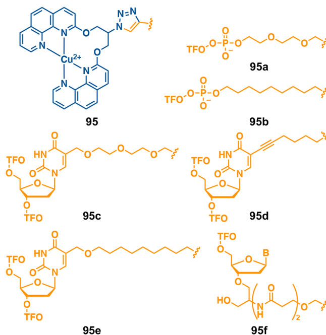
Figure 16. Clicked AMN–TFO hybrids with Clip-Phen developed by Hocke and co-workers. 143
