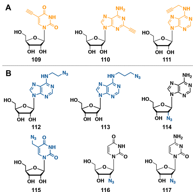
Figure 20. (A) Alkyne modified nucleosides used for cellular metabolic labeling of RNA: EU (109); 154 EA (110); 155 and N 6 pA (111). 156 (B) Azide modified purine (112–114) 158 and pyrimidine (115–117) 158,161,162 derivatives used for cellular metabolic labeling of RNA.
