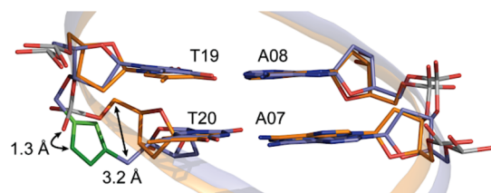
Figure 27. Close-up showing the overlaid average structures of a duplex containing the triazole (in purple 13merTAL, PDB: 2L8I) and an unmodified DNA duplex (in orange 13merRef, PDB: 2KUZ). The triazole modification is highlighted in green (Adapted with permission from ref 176. Copyright 2011, John Wiley & Sons). 176
