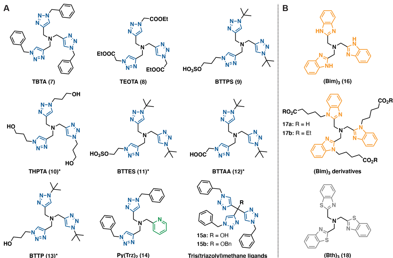
Figure 2. Polydentate ligands used to accelerate the CuAAC reaction. (A) Weaker ligands based on the 1,4-triazole ring suitable for environments with high water content: TBTA = tris[(1-benzyl-1H-1,2,3-triazol-4-yl)methyl]amine (7); TEOTA = tris[(1-(2-ethoxy-2-oxoethyl)-1H-1,2,3-triazol-4-yl)methyl]amine (8); BTTPS = 3-[4-{(bis[(1- tert -butyl-1H-1,2,3-triazol-4-yl)methyl]amino)methyl}-1H-1,2,3-triazol-1-yl]propyl hydrogen sulfate (9); THPTA = tris[(1-hydroxypropyl-1H-1,2,3-triazol-4-yl)methyl]amine (10); BTES = 2-[4-{(bis[(1- tert -butyl-1H-1,2,3-triazol-4-yl)methyl]amino)methyl}-1H-1,2,3-triazol-1-yl]ethyl hydrogen sulfate (11); BTAA = 2-[4-{(bis[(1- tert -butyl-1H-1,2,3-triazol-4-yl)methyl]amino)methyl}-1H-1,2,3-triazol-1-yl]acetic acid (12); BTTP = 3-[4-{(bis[(1- tert -butyl-1H-1,2,3-triazol-4-yl)methyl]amino)methyl}-1H-1,2,3-triazol-1-yl]propanol (13); Py = pyridine; Trz = (triazolylmethyl)amine. (B) Strong ligands based on benzimidazole (Bim) or benzothiazole (Bth) rings suitable for reaction environment with high concentration of coordinating organic solvents; *Ligands biocompatible with cellular conditions.
