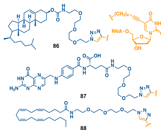
Figure 14. Clicked RNA-hybrids with receptor-binding molecules. 139
