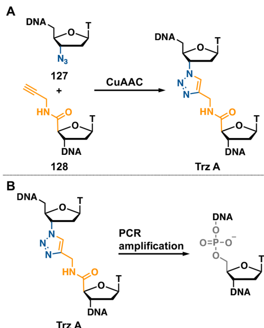
Scheme 7. Synthesis (A) and PCR Amplification (B) of Triazole A (Trz A) First Reported by Brown and Co-workers 180
