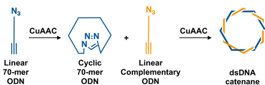
Figure 36. Generation of a dsDNA catenane by the templated click ligation of a linear ODN on a complementary cyclic oligonucleotide. 18
