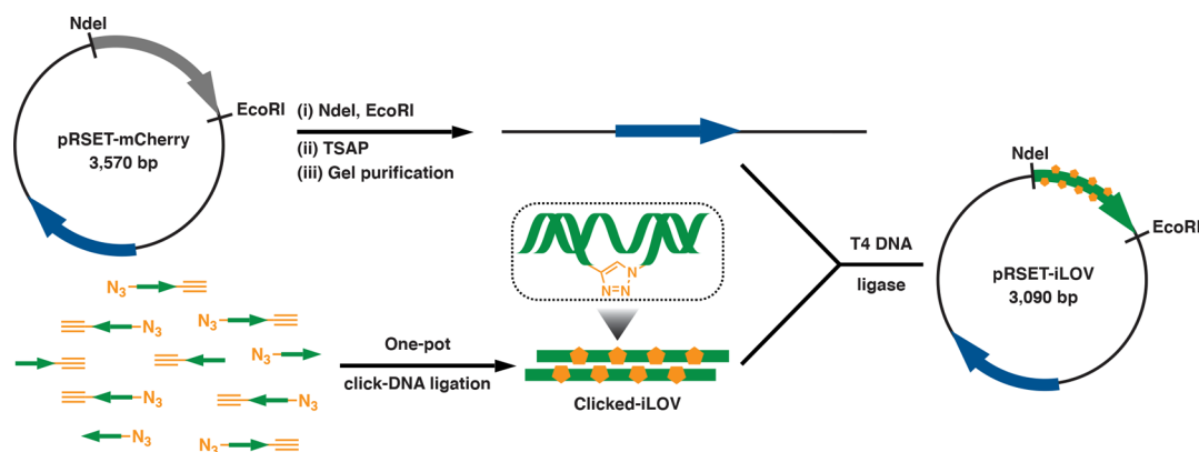
Figure 26. ILOV gene was assembled using templated CuAAC ligation from alkyne/azide oligonucleotides; a plasmid vector (pRSET-mCherry) was cleaved with NdeI and EcoRI restriction nucleases to remove the mCherry gene (encoding for a red fluorescent protein). The sticky ends of the linearized plasmid and artificial gene were then ligated using T4 DNA ligase to form the pRSET-iLOV plasmid (encoding for a green fluorescent protein). 183
