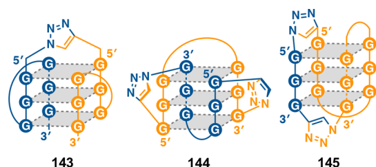
Figure 33. Conformational isomers of G-quadruplexes trapped by click chemistry. 200
