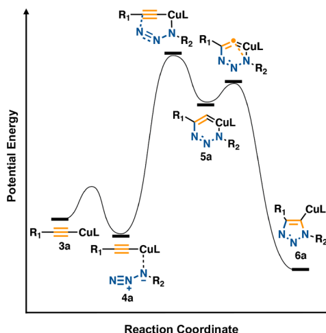
Figure 1. Energy profile of the reaction of copper(I) acetylides with organic azide based on DFT studies (L is CH 3 CN or H 2 O) and proposed by K. B. Sharpless. 37
