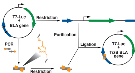
Figure 25. Triazole B is inserted into the BLA gene (blue) of plasmid DNA followed by transformation and growth of E. coli . The insert is gray, and the triazole linkages are orange. 24
