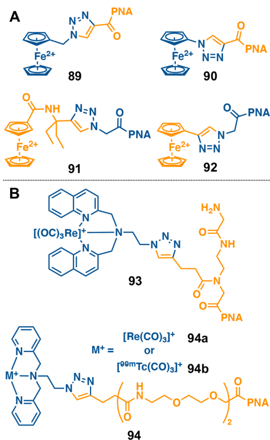
Figure 15. Clicked PNA–metal complex hybrids as electrochemical (A), 140 fluorescent, 141 or radioactive 142 (B) sensors.
