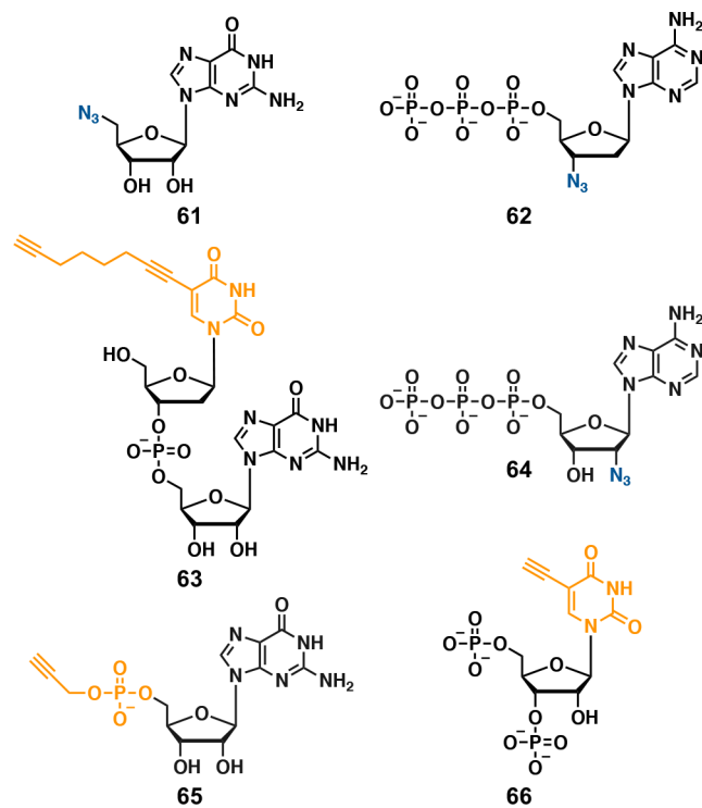
Figure 10. Alkyne and azide building blocks introduced into RNA enzymatically.
