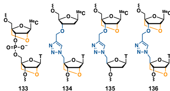
Figure 30. Structures of phosphodiester and triazole linked LNA backbones analyzed for DNA and RNA binding. 191
