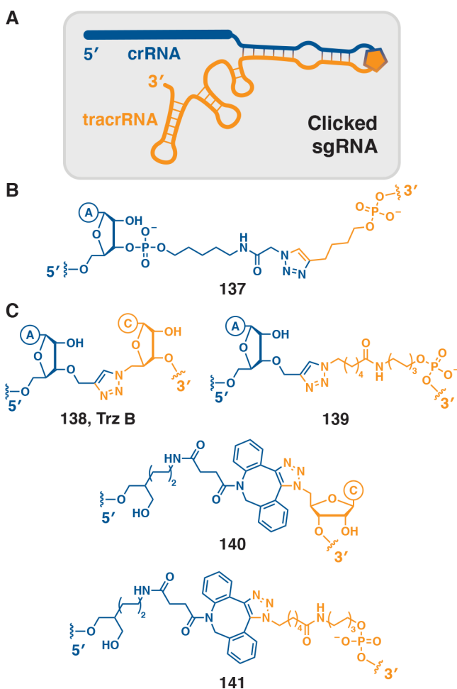
Figure 31. A 3'-azide (or alkyne) modified crRNA and a 5'-alkyne (or azide) modified Cas9-binding RNA are clicked together at the upper stem to generate a chemically ligated sgRNA construct (A) where a natural phosphate linkage is substituted by the triazole. (B) Type of triazole linkage used by Smith and co-workers. 196 Type of triazole linkages used by Brown and co-workers. 197
