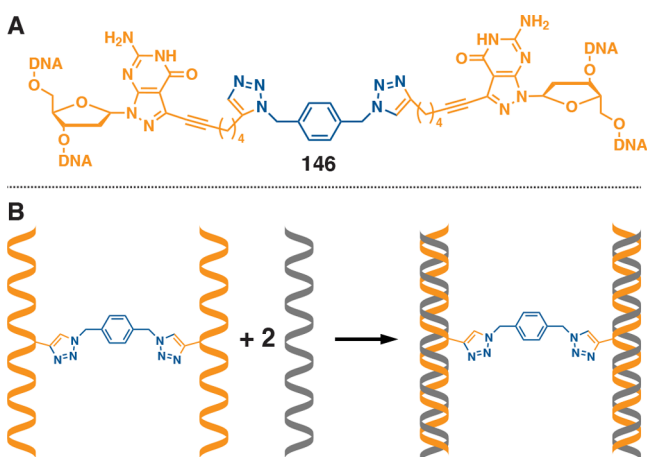
Figure 34. Bis-click strategy where an interstrand click cross-linker (A) was used by Seela and co-workers to generate a fourstranded DNA structure consisting of two cross-linked duplexes (B). 201
