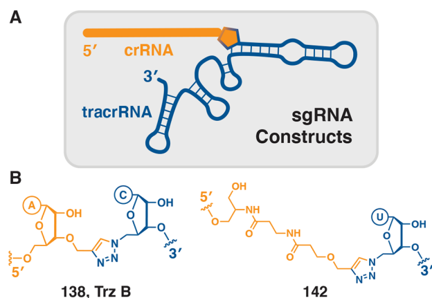
Figure 32. (A) 3'-Alkyne modified variable RNA (20mer) and a 5'-azide modified Cas9-binding RNA (79mer) are clicked together at the PAM site to make the chemically ligated sgRNA construct. (B) Structures of the artificial linkages used to conjugate the two RNA strands. 197
