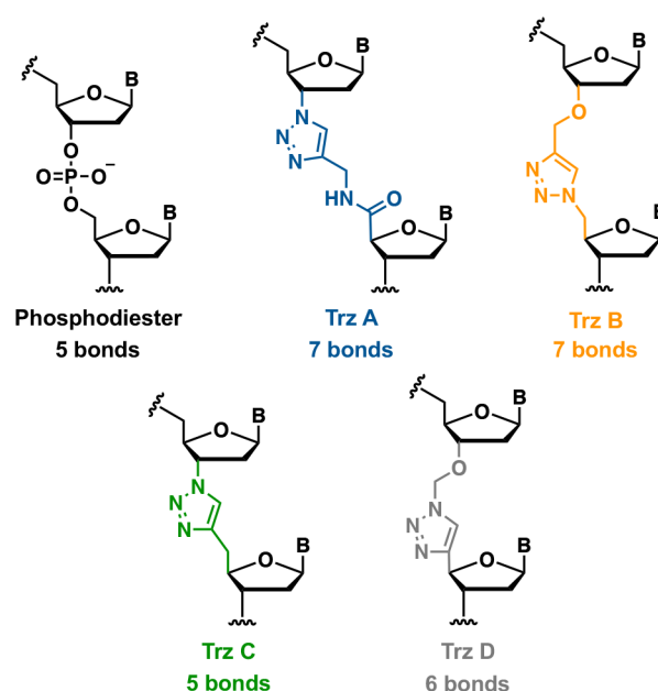
Figure 23. Canonical phosphodiester linkage and first-generation triazole linkage A (Trz A), second generation triazole linkage B (Trz B), and triazole linkage C (Trz C) in TL DNA reported by Isobe et al. and triazole linkage D (Trz D) reported by Varizhuk et al. The number of bonds between the C3' and C4' atoms of adjacent sugar rings is indicated.
