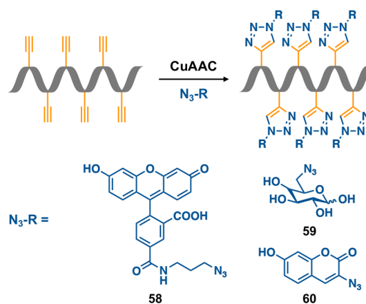
Figure 9. Strategy for high-density postsynthetic labeling of alkyne-modified DNA primers and azide labels (fluorescein azide, 58; azido-sugar, 59; and coumarin azide, 60) used in the click coupling by Carell et al. 17
