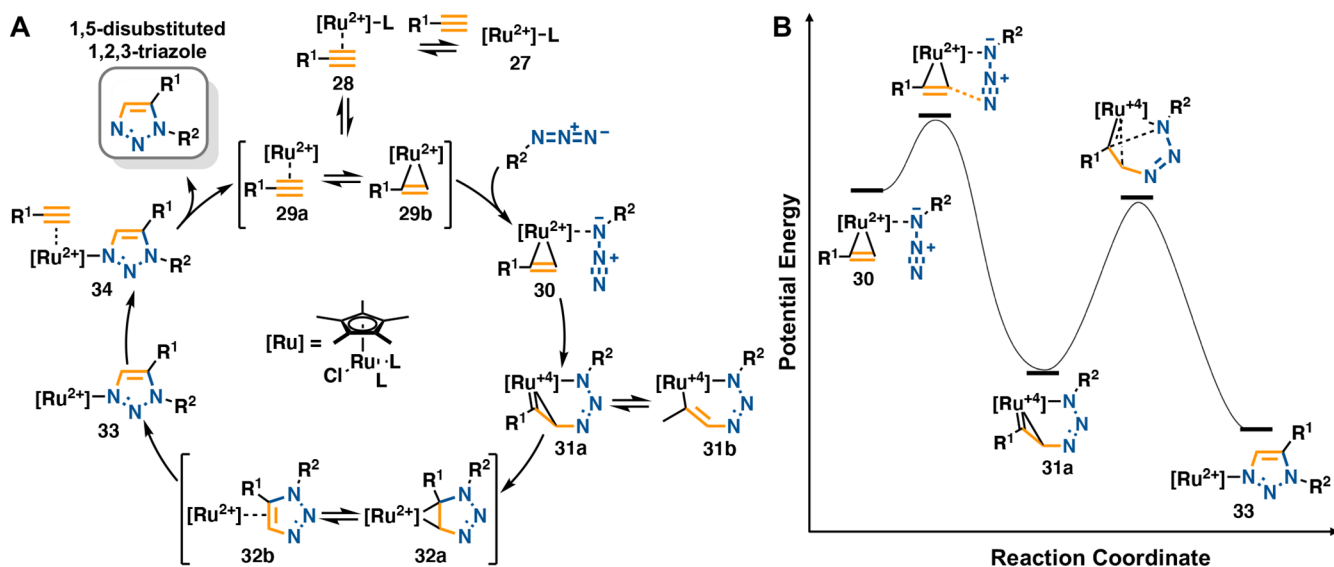
Figure 4. (A) Proposed mechanism for the Ru-catalyzed azide–alkyne cycloaddition (RuAAC). (B) Energy profile of the lowest-energy RuAAC pathway based on DFT studies. 71
