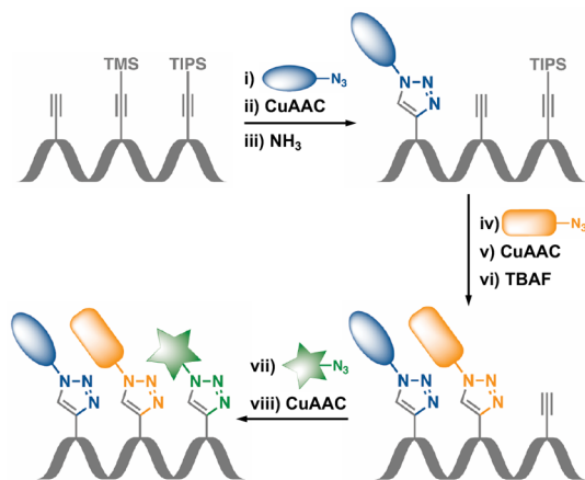
Scheme 5. Click-Click-Click Strategy Developed by Carell and Co-workers for the Sequential Labeling of Oligonucleotides with up to Three Different Probes 102
