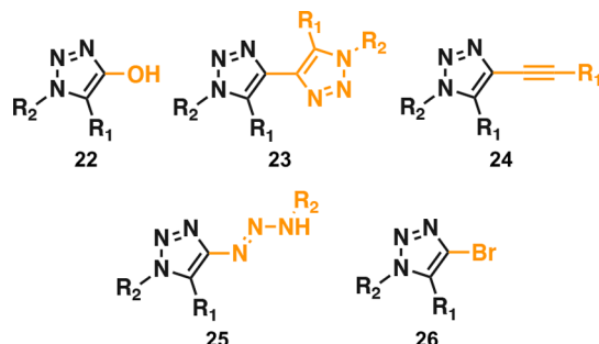
Figure 3. Possible byproducts from the reaction between metal acetylides and azides. 68
