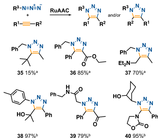
Figure 5. Regiochemistry in RuAAC coupling with internal alkynes. (a) \text{Cp}^*\text{RuCl}(\text{PPh}_3)_2 (10 mol %), benzene, 80 °C, 2.5–40 h; 74 (b) \text{Cp}^*\text{RuCl}(\text{COD}) (2 mol %), toluene, rt, 30 min. 71
