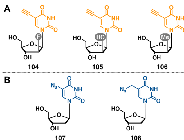
Figure 19. (A) Arabinofuranosyl-5-ethynyluridine derivatives studied for cellular metabolic labeling of DNA: F-ara-EdU (104); ara-EU (105); and Me-ara-EdU (106). 120 (B) Azide modified uridine derivatives AdU (107) and AmdU (108) used for cellular metabolic labeling of DNA. 23,153
