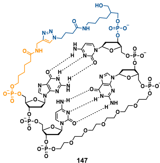
Figure 35. Chemical structure of a stable cyclic GC/GC dinucleotide mini-duplex.
