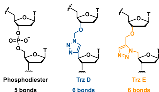
Figure 28. Canonical phosphodiester linkage beside the 1,4-disubstituted triazole D (Trz D) and the 1,5-disubstituted triazole E (Trz E).
