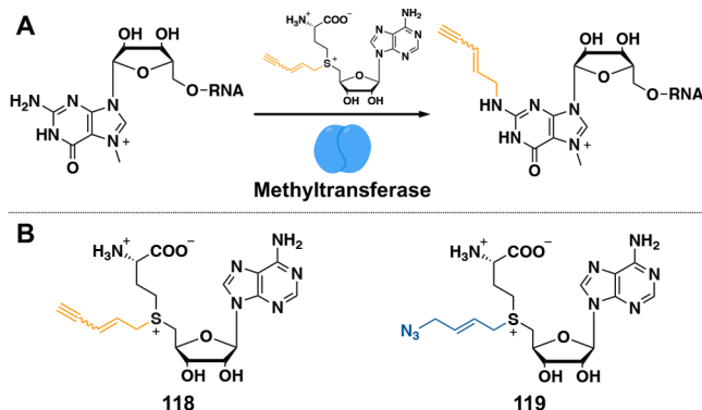
Figure 21. (A) General strategy for the metabolic labeling of RNA where a click reporter group is transferred to the N2 of m7G by a methyltransferase. (B) AdoMet derivatives used for the metabolic labeling with methyltransferases AdoEnYn (118) and AbSAM (119). 165,166
