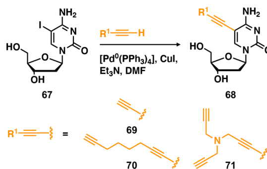
Scheme 3. Synthesis of Alkyne-Modified Nucleosides by Sonogashira Coupling 124–127
