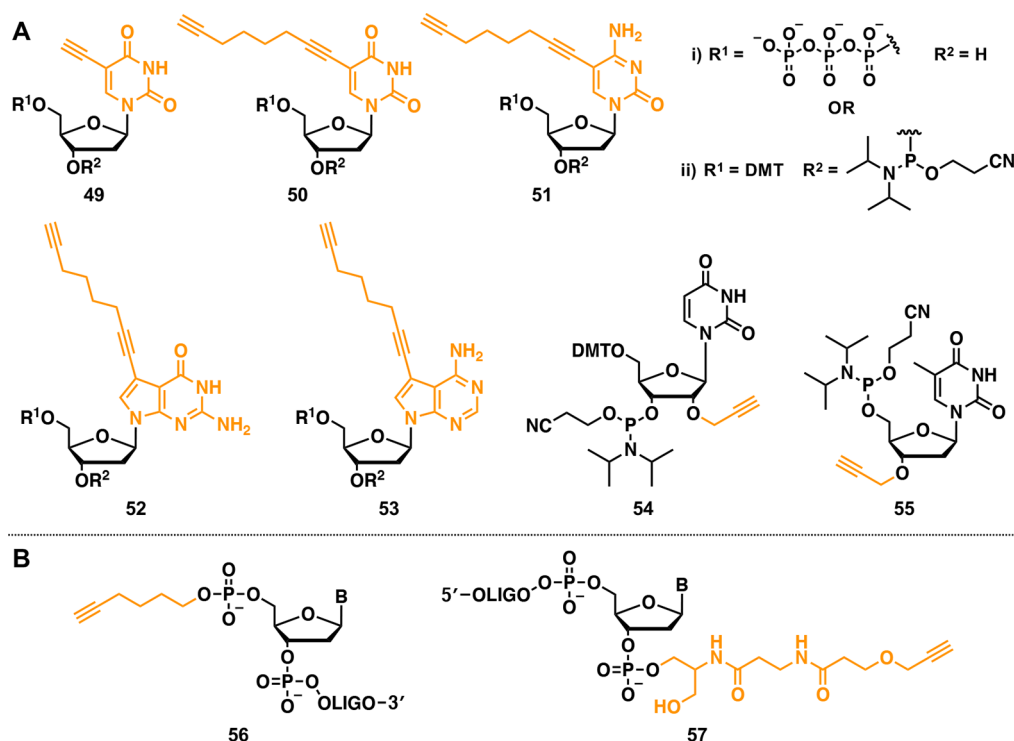
Figure 8. (A) Examples of modified nucleosides used to incorporate alkyne groups into oligonucleotides. Modifications 49–53 have been used both as triphosphates (i) and phosphoramidites (ii) monomers for PCR or solid phase synthesis, respectively; Phosphoramidites 54 and 55 have been used to introduce 2'- and 3'-O-propargyl modifications in oligonucleotides by normal and reverse phosphoramidite coupling. (B) Alkyne modifications such as hexynyl (56) and serinol (57) have been introduced through non-nucleosidic alkyne phosphoramidite monomers and solid supports on the 5'- and 3'-ends, respectively.
