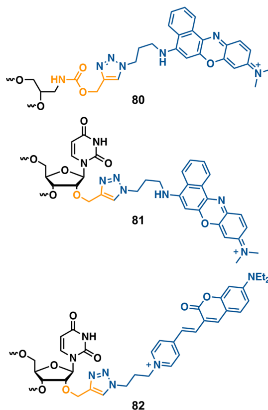
Figure 12. Fluorescent modifications (phenoxazinium azide, 80, 81; and red coumarin azide, 82) introduced through CuAAC by Wagenknecht and co-workers. 135
