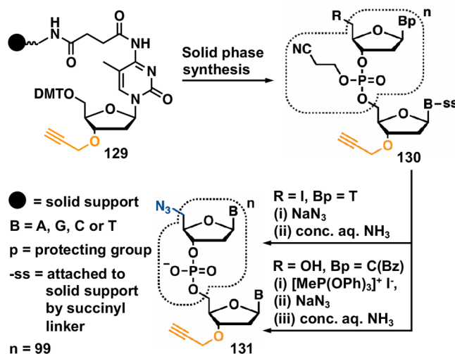
Scheme 8. Synthesis of Alkyne/Azide 100-mer Oligonucleotides for Use in Click Ligation and Cyclization 24
