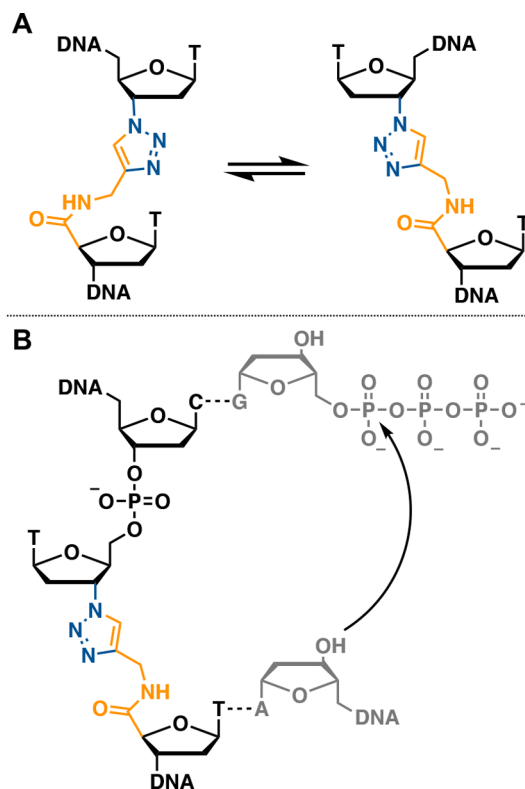
Figure 24. (A) Possible isomerization at the amide bond. (B) One of the thymine bases is skipped by the replication machinery if the configuration between the two substituents is trans . 180
