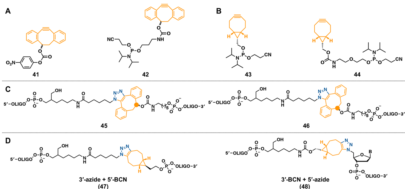
Figure 7. (A) Dibenzocyclooctyne (DIBO) oligonucleotide labeling reagents: DIBO p-nitrophenyl carbonate (41) and phosphoramidite monomer (42) for coupling at the 5'-termini of oligonucleotides. (B) Achiral bicyclo[6.1.0]nonyne (BCN) oligonucleotide labeling reagents: BCN-CEP I (43) and BCN-CEP II (44). (C) Click linkage between 3'-azide and 5'-DIBO labeled oligonucleotides. Both regioisomers of the DIBO triazole are shown. (D) Both 3'- and 5'-ends of oligonucleotides can be labeled with BCN, and its click reactions provide single regioisomers.
