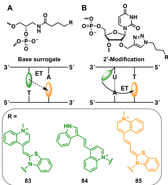
Figure 13. (A) TO (83) and TR (85) as two base surrogates allow excitonic interactions that interfere with energy transfer (ET). (B) For TO (or CyIQ, 84) as the 2'-modification, the U–A base pair blocks excitonic interactions (green, TO or CyIQ; orange, TR). 137
