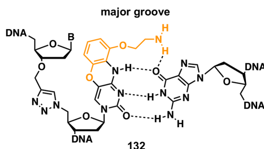
Figure 29. Structure of the triazole G-clamp base paired with guanine in complementary DNA. The additional steric bulk of the nucleobase derivative of cytosine is highlighted in orange. 177
