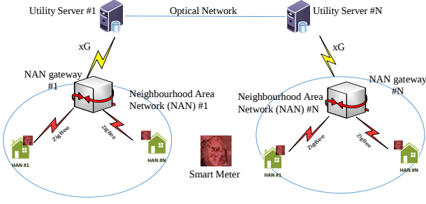
Fig. 1. Considered Smart Metering Infrastructure.
