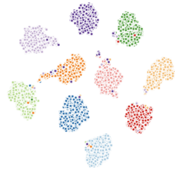
Figure 6.1.1: SCAES learn to explain different object classes with separate object capsules, thereby doing unsupervised classification. Here, we show TSNE embeddings of object capsule presence probabilities for 10000 MNIST digits. Individual points are color-coded according to the corresponding digit class.
