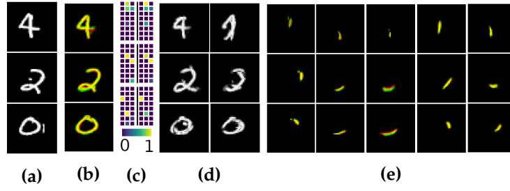
Figure 6.2.3: MNIST (a) images, (b) reconstructions from part capsules in red and object capsules in green, with overlapping regions in yellow. Only a few object capsules are activated for every input (c) a priori (left) and even fewer are needed to reconstruct it (right). The most active capsules (d) capture object identity and its appearance; (e) shows a few of the affine-transformed templates used for reconstruction.
