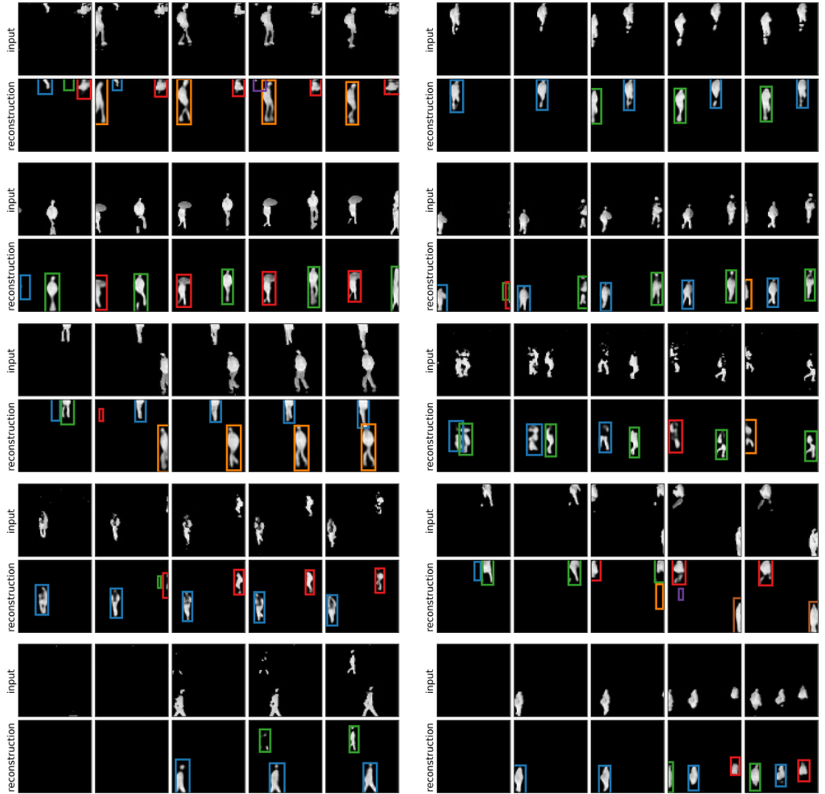
Figure 5.I.1: Sequences of input (first row) and SQAIR reconstructions with marked glimpse locations. While not perfect (spurious detections, missed objects), they are temporally consistent and similar in appearance to the inputs.
