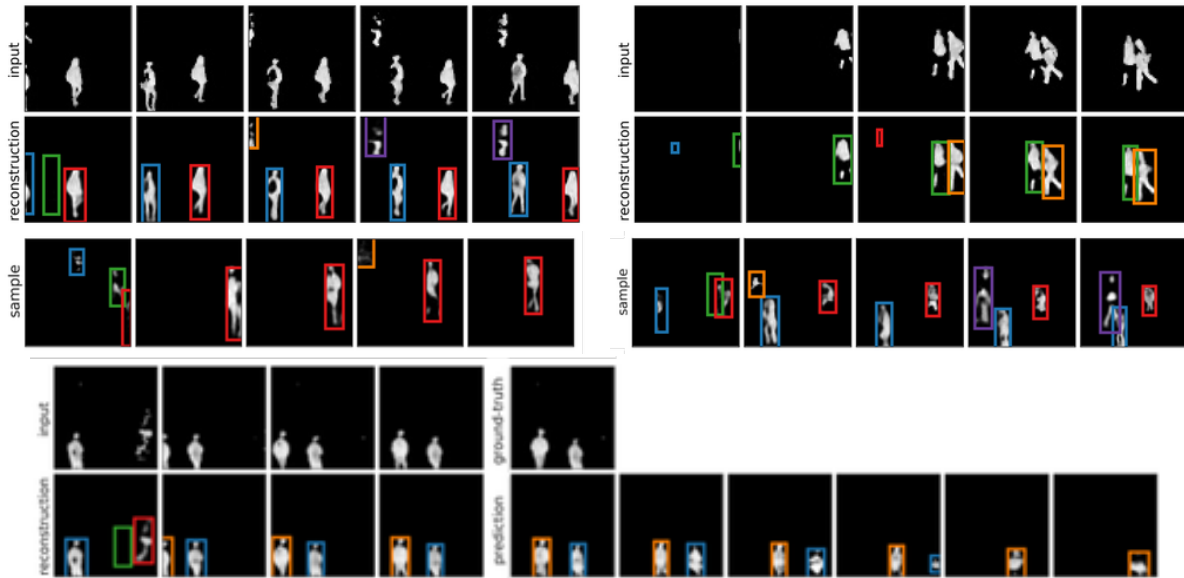
Figure 5.4.5: Inputs on the top, reconstructions in the second row, samples in the third row; rows four and five contain inputs and conditional generation: the first four frames in the last row are reconstructions, while the remaining ones are predicted by sampling from the prior. There is no ground-truth, since we used sequences of length five of training and validation.
