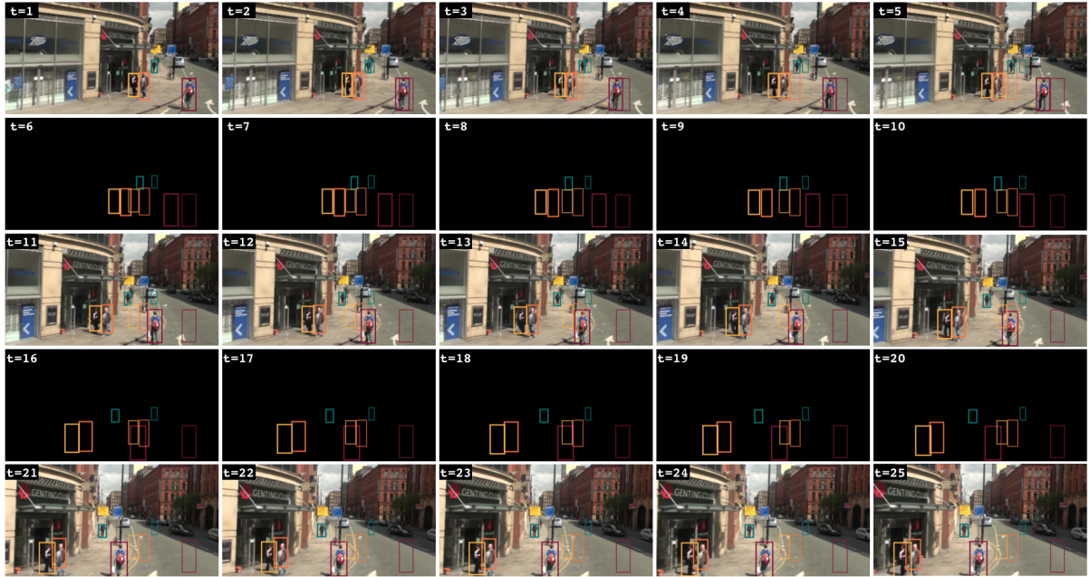
Figure 4.5.1: Camera blackout experiment on a street scene from the MOTChallenge dataset with strong ego-motion. Solid boxes are MOHART predictions (for t \geq 2 ), faded bounding boxes indicate object locations in the first frame. As the model is trained end-to-end, MOHART learns to fall back onto its internal motion model if no new observations are available (black frames). As soon as new observations come in, the model ‘snaps’ back onto the tracked objects.
