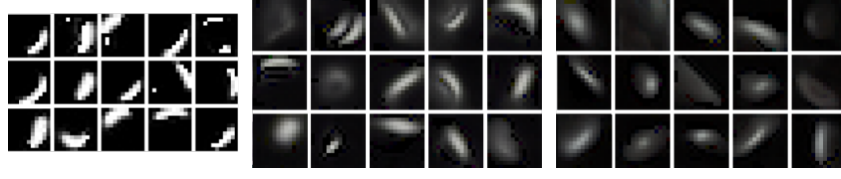
Figure 6.2.2: Stroke-like templates learned on MNIST (left) as well as sobel-filtered SVHN (middle) and CIFAR10 (right). For SVHN they often take the form of double strokes due to sobel filtering.
