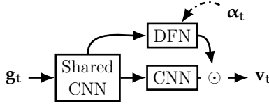
Figure 3.3: Architecture of the appearance attention. V1 is implemented as a CNN shared among the dorsal stream (DFN) and the ventral stream (CNN). The \odot symbol represents the Hadamard product and implements masking of visual features by the foreground/background segmentation.
