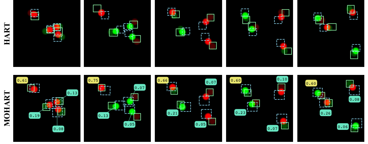
Figure 4.3.2: A scenario constructed to be impossible to solve without relational reasoning. Circles of the same colour repel each other, circles of different colour attract each other. Crucially, each circle is randomly assigned its identity in each time step. Hence, the algorithm can not infer the forces exerted on one object without knowledge of the state of the other objects in the current time step. The forces in this scenario scale with 1/\sqrt{r} and the algorithm was trained to predict one time step into the future. HART (top) is indeed unable to predict the future location of the objects accurately. The achieved average IoU is 47%, which is only slightly higher than predicting the objects to have the same position in the next time step as in the current one (34%). Using the relational reasoning module, MOHART (bottom) is able to make meaningful predictions (76% IoU). The numbers in the bottom row indicate the self-attention weights from the perspective of the top left tracker (yellow number box). Interestingly, the attention scores have a strong correlation with the interaction strength (which scales with distance) without receiving supervision.
