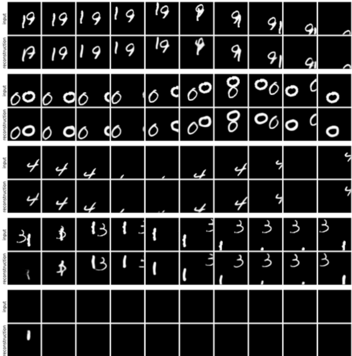
Figure 5.H.1: Sequences of input (first row) and sQAIR reconstructions with marked glimpse locations. Reconstructions are all temporally consistent.
