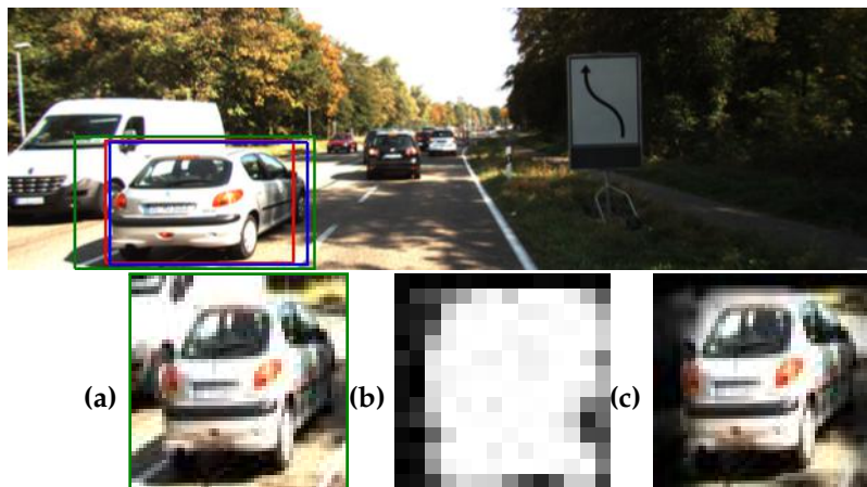
Figure 3.1: KITTI image with the ground-truth and predicted bounding boxes and an attention glimpse . The lower row corresponds to the hierarchical attention of our model: 1 st layer extracts an attention glimpse (a), the 2 nd layer uses appearance attention to build a location map (b). The 3 rd layer uses the location map to suppress distractors, visualised in (c).
