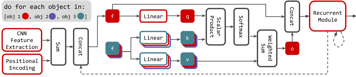
Figure 4.3.1: The relational reasoning module in MOHART based on multi-headed self-attention. Here, we show the computation of the interaction of the red object with all other objects. Object representations f_{t,m} are computed using visual features, positional encoding and the hidden state from the recurrent module. These are linearly projected onto keys ( k ), queries ( q ), and values ( v ) to compute a weighted sum of interactions between objects, yielding an interaction vector o_{t,m} . Subscripts t, m are dropped from all variables for clarity of presentation, so is the splitting into multiple heads.
