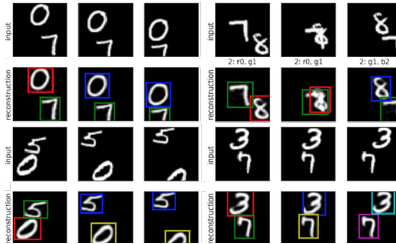
Figure 5.G.2: Examples of re-detections in MLP-SQAIR. Bounding box colours correspond to object identity, assigned to it upon discovery. In some training runs, SQAIR converges to a solution, where objects are re-detected in the second frame, and PROP starts tracking only in the third frame (left). Occasionally, an object can be re-detected after it has severely overlapped with another one (top right). Sometimes the model decides to use only DISC and repeatedly discovers all objects (bottom right). These failure mode seem to be mutually exclusive – they come from different training runs.
