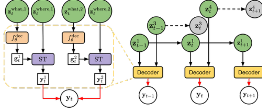
Figure 5.2.1: Left: Generation in AIR. The image mean y_t is generated by first using the glimpse decoder f_\theta^{\text{dec}} to map the what variables into glimpses g_t , transforming them with the spatial transformer ST according to the where variables and summing up the results. Right: Generation in SQAIR.
