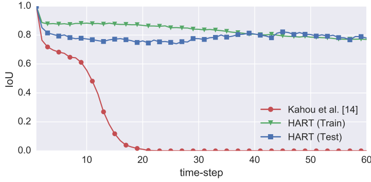
Figure 3.5: IoU curves on KITTI over 60 timesteps. HART (train) presents evaluation on the train set (we do not overfit).
