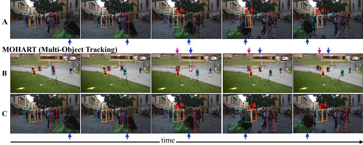
Figure 4.E.1: Tracking examples of both HART and MOHART. Coloured boxes are bounding boxes predicted by the model, arrows point at challenging aspects of the scenes. (A) & (C): Each person being tracked is temporarily occluded by a woman walking across the scene (blue arrows). MOHART, which includes a relational reasoning module, handles this more robustly (compare red arrows).
