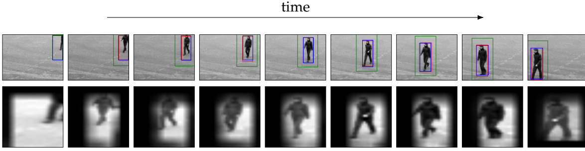
Figure 3.4: Tracking results on KTH dataset Schuldts et al. [152]. Starting with the first initialisation frame where all three boxes overlap exactly, time flows from left to right showing every 16 th frame of the sequence captured at 25fps. The colour coding follows from Figure 3.1. The second row shows attention glimpses multiplied with appearance attention.
