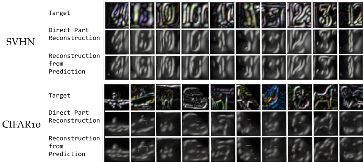
Figure 6.B.1: 10 Sample SVHN and Cifar10 reconstructions. First row shows Sobel filtered target image. Second row shows the reconstruction from Part Capsule Layer directly. Third row shows the reconstruction if we use the object predictions for the Part poses instead of Part poses themselves for reconstruction. The templates in this model has the same number of channels as the image, but they have converged to black and white templates and the reconstruction do not have color diversity. The SCAE model is trained completely unsupervised but the reconstructions tend to focus on the center digit in SVHN and filter the rest of the clutter.
