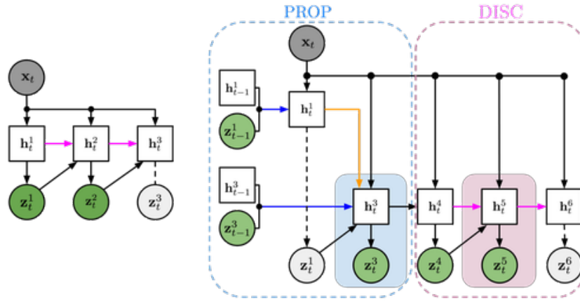
Figure 5.3.1: Left: Inference in AIR. The pink RNN attends to the image sequentially and produces one latent variable z_t^1 at a time. Here, it decides that two latent variables are enough to explain the image and z_t^3 is not generated. Right: Inference in SQAIR starts with the Propagation (PROP) phase. PROP iterates over latent variables from the previous time-step t-1 and updates them based on the new observation x_t . The blue RNN runs forward in time to update the hidden state of each object, to model its change in appearance and location throughout time. The orange RNN runs across all current objects and models the relations between different objects. Here, when attending to z_{t-1}^1 , it decides that the corresponding object has disappeared from the frame and forgets it. Next, the Discovery (DISC) phase detects new objects as in AIR, but in SQAIR it is also conditioned on the results of PROP, to prevent rediscovering objects. See Figure 5.3.2 for details of the colored RNNs.
