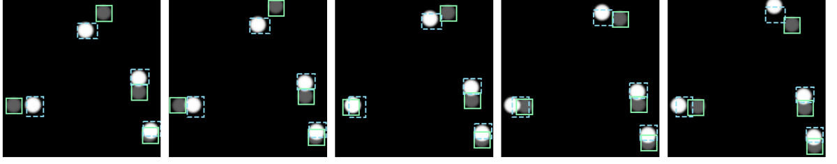
Figure 4.C.1: HART single object tracking applied four times in parallel and trained to predict the location of each circle three time steps into the future. Dashed lines indicate spatial attention, solid lines are predicted bounding boxes, faded circles show ground truth location at T + 3 . Each circle exerts repulsive forces on each other, where the force scales with 1/r , r being their distance.
