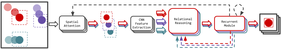
Figure 4.1.1: Multi-object hierarchical attentive recurrent tracking (MOHART). A glimpse is extracted for each object using a (fully differentiable) spatial attention mechanism. These glimpses are further processed with a CNN and fed into a relational reasoning module. A recurrent module which iterates over time steps allows for capturing of complex motion patterns. It also outputs spatial attention parameters and a feature vector per object for the relational reasoning module. Dashed lines indicate temporal connections (from time step t to t + 1 ). The entire pipeline operates in parallel for the different objects, only the relational reasoning module allows for exchange of information between tracking states of each object. MOHART is an extension of HART (a single-object tracker), which features the same pipeline without the relational reasoning module.
