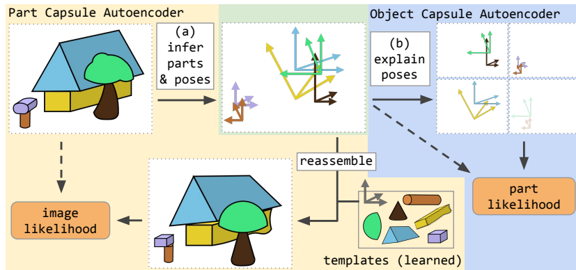
Figure 6.1.2: Stacked Capsule Autoencoder (SCAE): (a) part capsules segment the input into parts and their poses. The poses are then used to reconstruct the input by affine-transforming learned templates. (b) object capsules try to arrange inferred poses into objects, thereby discovering underlying structure. SC AE is trained by maximizing image and part log-likelihoods subject to sparsity constraints.
