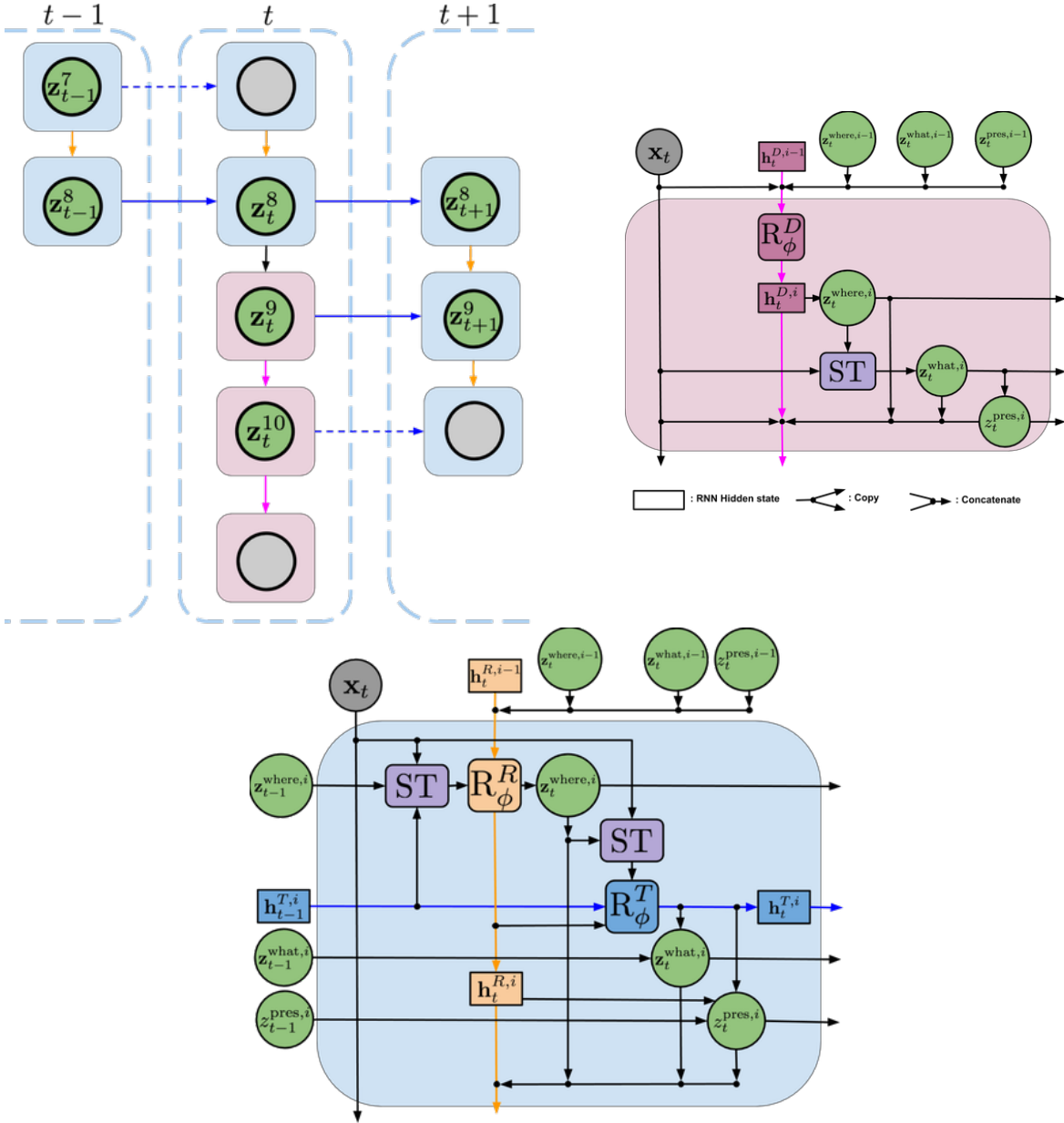
Figure 5.3.2: Left: Interaction between PROP and DISC in SQAIR. Firstly, objects are propagated to time t , and object i = 7 is dropped. Secondly, DISC tries to discover new objects. Here, it manages to find two objects: i = 9 and i = 10 . The process recurs for all remaining time-steps. Blue arrows update the temporal hidden state, orange ones infer relations between objects, pink ones correspond to discovery. Bottom: Information flow in a single discovery block ( left ) and propagation block ( right ). In DISC we first predict where and extract a glimpse. We then predict what and presence . PROP starts with extracting a glimpse at a candidate location and updating where . Then it follows a procedure similar to DISC, but takes the respective latent variables from the previous time-step into account. It is approximately two times more computationally expensive than DISC. For details, see Algorithms 2 and 3 in Section 5.A.
