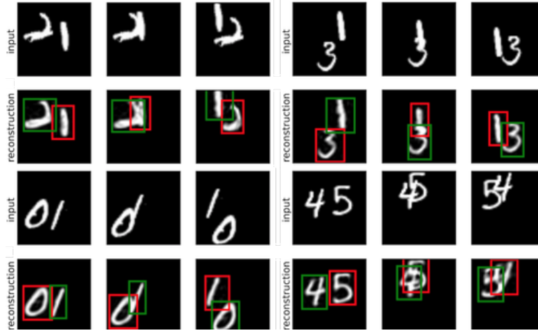
Figure 5.G.1: Examples of ID swaps in a version of SQAIR without proposal glimpse extraction in PROP (see Section 5.A for details). Bounding box colours correspond to object index (or its identity). When PROP is allowed the same access to the image as DISC, then it often prefers to ignore latent variables, which leads to swapped inference order.
