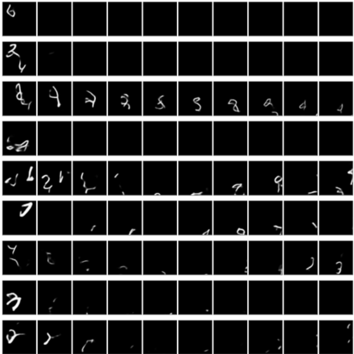
Figure 5.H.4: Samples from CONV-VRNN. They show lack of temporal consistency. Objects in the generated frames change between consecutive time-steps and they do not resample digits from the training set.
