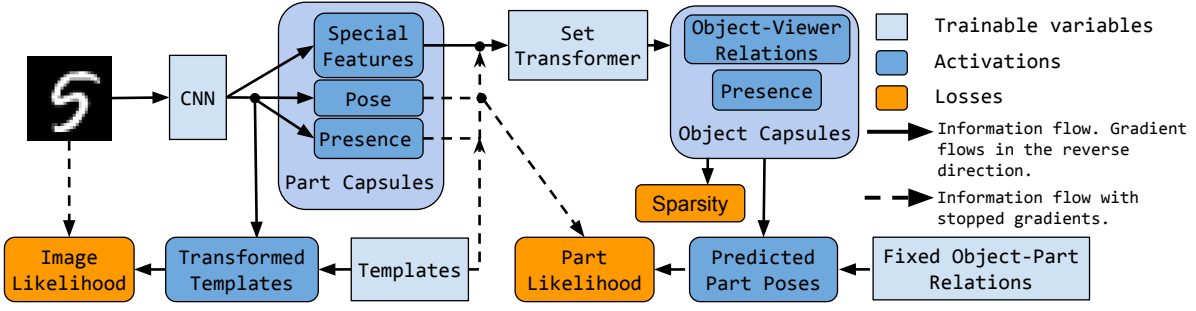
Figure 6.2.4: SCAE architecture.
