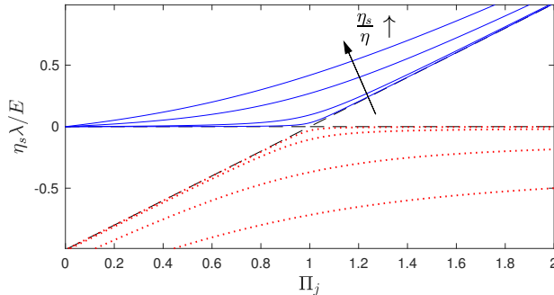
FIGURE 4. Growth rates of the linear buckling modes, \eta_s \lambda / E , against the scaled load \Pi_j in (3.6). Curves with \eta_s/\eta = 10^{-3} , 0.01, 0.1 and 0.3 are shown; the dashed lines show the limit \eta_s/\eta \rightarrow 0 .
