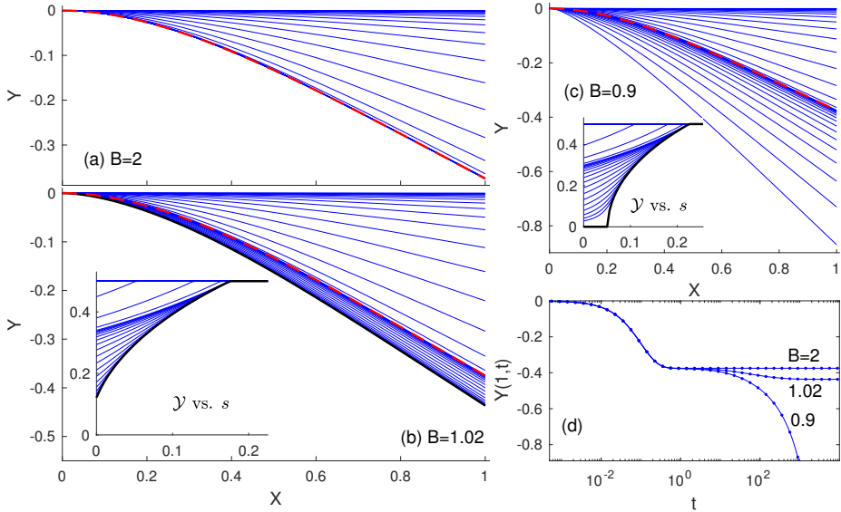
FIGURE 9. Droop of an elasto-visco-plastic cantilever with E = 1 , \eta_s = 0.1 and \eta = 10 . Shown are snapshots of the centerline for (a) B = 2 , (b) B = 1.02 and (c) B = 0.9 . The red dashed lines show the purely elastic equilibrium ( cf. figure 3). In (b), the darker solid line is the final elasto-viscoplastic state. The insets in (b) and (c) show snapshots of the evolving yield surface \mathcal{Y}(s, t) , with darker solid lines showing (5.21). In (d), we plot Y(1, t) for the three solutions; the dots indicate the times of the snapshots in (a)–(c).
