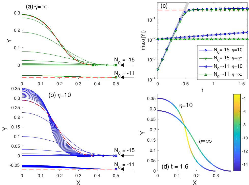
FIGURE 5. Snapshots of non-linear buckling solutions, (X(s, t), Y(s, t)) , with \eta_s = 0.01 , E = 1 and either N_0 = -11 or -15 , initiated with a small deflection from a straight beam. In (a) we show the solution for the Kelvin limit ( \eta \rightarrow \infty ), and in (b), we show the case with \eta = 10 , plotting half of the (symmetrical) beam in each case. The two solutions with N_0 = -11 are offset for clarity, and the circles mark the ends of the beam. Dashed lines show the expected elastic solutions (satisfying (2.40)-(2.42) with M = -\frac{1}{3}\kappa E and calculated numerically). In panel (c), we plot the maximum deflection Y(0, t) of the solutions against time. The grey lines show the expected linear buckling behaviour, and points indicate the times of the snapshots in (a) and (b). The shapes of the two cases at the final time are shown in panel (d), with shading corresponding to local tension N .
