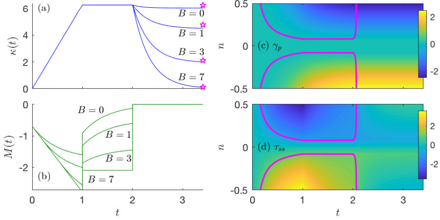
FIGURE 8. Curled elasto-viscoplastic ribbon solutions, showing (a) curvature and (b) bending moment with B = 0, 1, 3 or 7 , E = 1 , \eta = \frac{1}{2} and \eta_s = \frac{1}{3} . Here \kappa = 2\pi \min(t, 1) is imposed for 0 < t \leq 2 , and M = 0 for t > 2 . The stars in (a) mark the prediction from (5.15). Panels (c) and (d) show the plastic strain \gamma_p(n, t) , and the axial stress \tau_{ss}(n, t) for the case B = 1 , with the lines marking the position of the yield surfaces.
