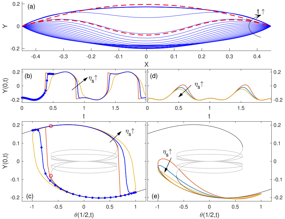
FIGURE 6. Buckled viscoelastic beams with periodically varying end angles \theta(\pm\frac{1}{2}, t) = \cos(2\pi t) , for \eta \rightarrow \infty and E = 1 , and with the horizontal distance between the ends being shortened by 0.1. (a) Snapshots for equally spaced time intervals spanning half the cycle as \theta(\frac{1}{2}, t) varies from 1 to -1 radians, for \eta_s = 0.01 . (b,d) Vertical displacement of the mid point Y(0, t) as a function of time over two cycles and (c,e) phase portraits on the (\theta(\frac{1}{2}, t), Y(0, t)) -plane, for \eta_s = 10^{-3} , 0.01 and 0.05 (panels (b) and (c)), and \eta = 0.15, 0.2 and 0.4 (panels (d) and (e)). In (b) and (c), the dots correspond to the snapshots in panel (a). In (c) and (e), the stable elastic equilibrium solutions are shown as black lines, while the grey lines show unstable branches. The two red dashed lines in (a) show the elastic equilibria solution either side of the saddle node (calculated numerically from (2.40)-(2.42) with M = -\frac{1}{3}\kappa E ), as indicated by the circles in (c).
