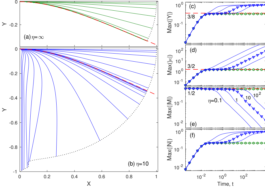
FIGURE 3. Snapshots of viscoelastic cantilevers for E = 1 , \eta_s = 10^{-2} and (a) \eta = \infty and (b) \eta = 10 . The dotted line shows the locus of the ends. On the right, we plot the maxima in (c) |Y| , (d) |\kappa| , (e) |M| and (f) |N| . The points indicate the times of the snapshots in (a)–(b); the circles show the \eta \rightarrow \infty solution. The dashed (red) lines show the expected, low-curvature, elastic solution Y(X) = -X^2(X^2 - 4X + 6)/8 (which, from (2.40)–(2.43), satisfies s \approx X , M \approx -\frac{1}{3}\kappa E , \kappa \approx Y'' , M'' \approx -1 , N \approx 0 and Y(0) = Y'(0) = M(1) = M'(1) = 0 ).
