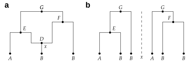
Fig. 2. A classical eARG. a. Standard graph depiction with breakpoint x associated with the recombination node D. Nodes E, F, and G are common ancestor events. b. Corresponding local trees to the left and right of breakpoint x (note these are shown in the conventional form in which only coalescences within the local tree are included hence D is omitted; see Appendix E for a discussion of this important point).
