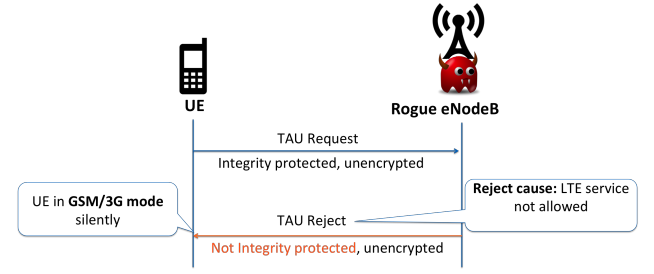
Fig. 8. DoS attack - denying LTE network services (D1)
