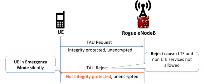
Fig. 9. DoS attack - denying all mobile network services (D2)
