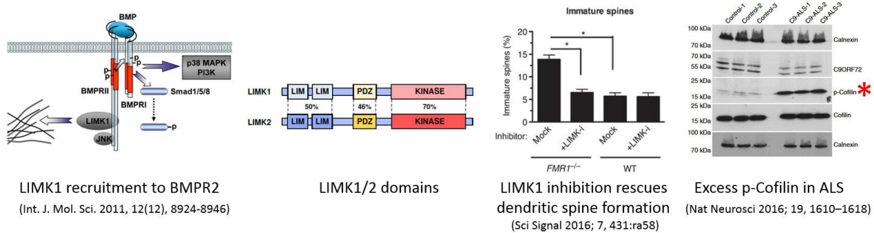
Fig.2 Domains and (dys)function of LIMK1
