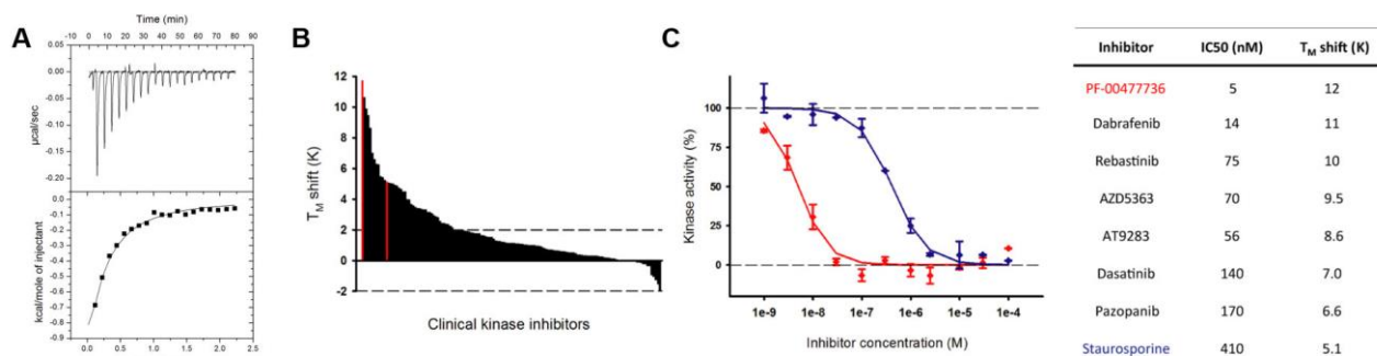
Fig. 5. In vitro assays. (A) ITC measurement of the binding of the LIMK1 LIM-LIM domains (a.a. 18-172) to a BMPR2 peptide (SNLKQVETGVAKMNTINAA) shows a K_D value of 60 \mu M. (B) Summary plot of a thermal shift assay screen of ~150 clinical kinase inhibitors. Red lines indicate the range of inhibitors chosen for IC 50 determination. (C) RapidFire mass spectrometry assay showing IC 50 values for selected compounds.
