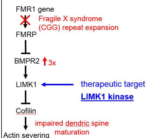
Fig. 1. Schematic of LIMK1 upregulation
