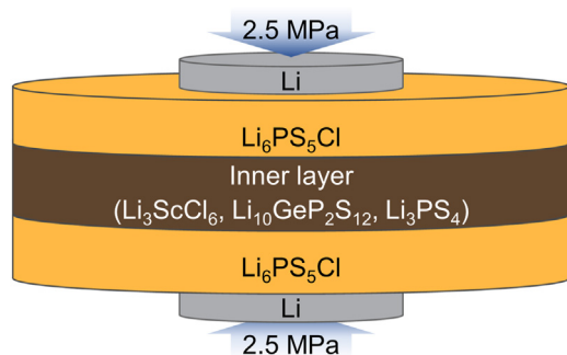
Figure 1. Schematic of solid-state cell with multi-layered solid electrolyte architecture
