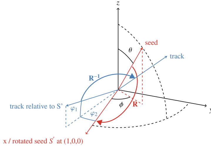
Figure 12. The auxiliary angular coordinates \varphi_1 and \varphi_2 are measured with respect to the rotated Seed track S' that aligns with the x-axis. They behave as standard angular coordinates.
