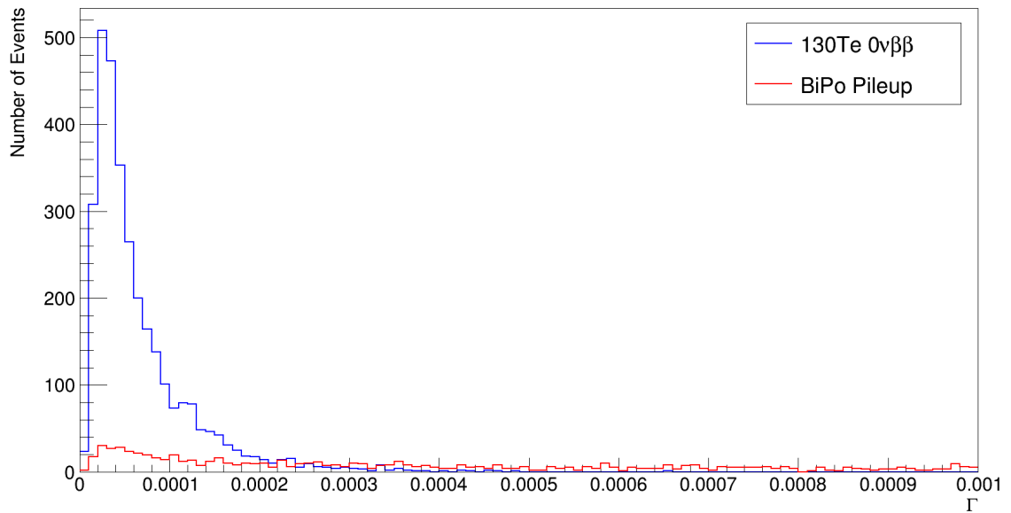
Figure 6.10: Distributions of \Gamma , as calculated using Equation 6.3, for ^{130}\text{Te } 0\nu\beta\beta (blue) and ^{214}\text{BiPo} pileup (red) events. Once again, ^{130}\text{Te } 0\nu\beta\beta events generally have much smaller values of \Gamma than the BiPo pileup events, which can have \Gamma much larger than the range shown here.
