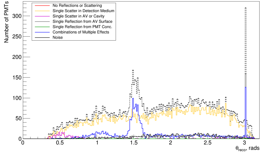
Figure 5.29: The reconstructed scattering angle \theta of all accepted photons in a simulation of 5000 laser head pulses with n_\gamma = 1500 , emitted at a wavelength of 405nm from fibre FS025, separated by the optical process(es) each photon was subject to before triggering the corresponding accepted PMT. The summation of all contributions is shown by the dashed line. The reconstruction method used the PMT's central position and the photon's calculated total path time.
