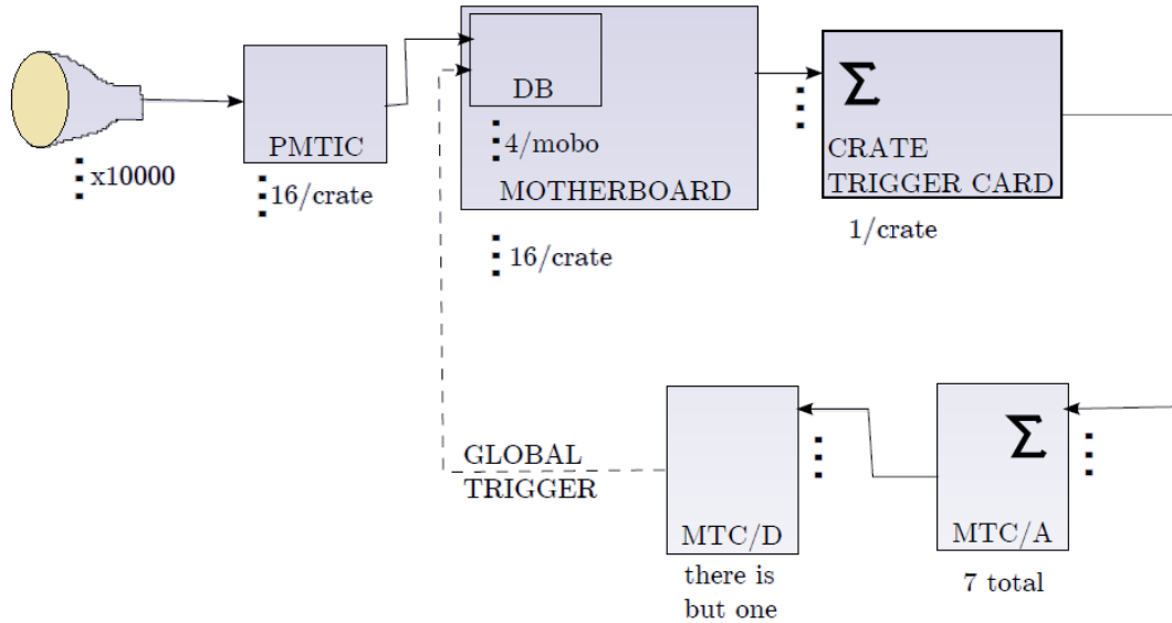
Figure 1.2: A basic overview of the SNO+ electronics flow, from a single PMT through the PMT Interface Card (PMTIC), the daughter board (DB) that is located on the mother board, through the Crate Trigger Card and on to the Analog and Digital Master Trigger cards (MTC/A and MTC/D respectively). Not shown are the XL3 boards that read out the non-trigger information from each mother board. This image has been adapted from [5].
