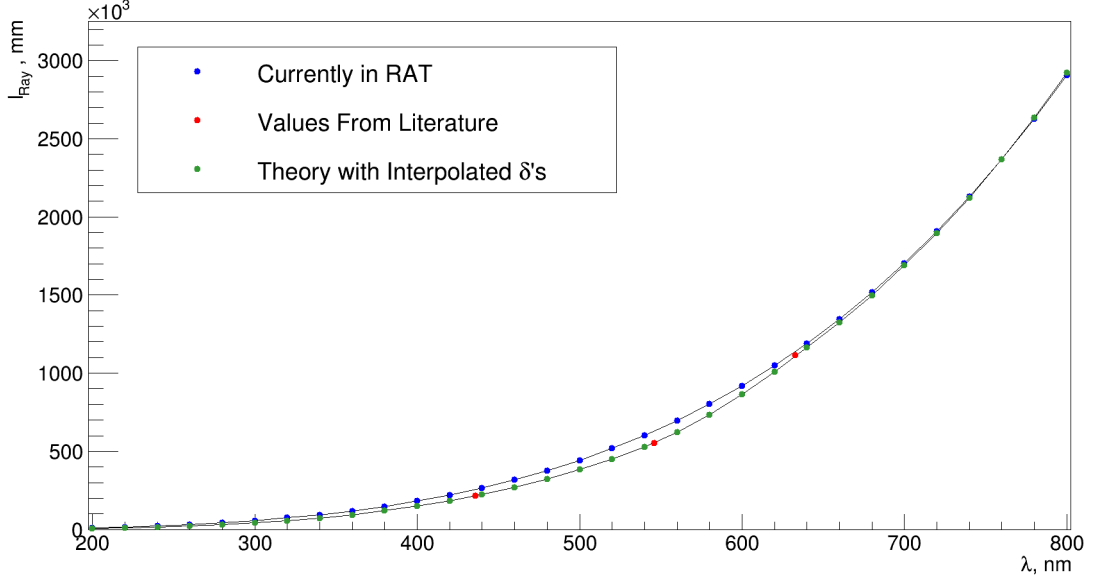
Figure 3.2: Values of the Rayleigh scattering length l_{Ray} of pure water at different wavelengths, originally derived from SNO's optical calibration data (blue). These values are now used in RAT for the simulation of scattering in pure water. Also shown are the values of l_{Ray} corresponding to the explicitly measured values of \delta discussed in Section 3.3 (red), and theoretical values of l_{Ray} calculated using Equation 3.29 (green), with the various equation parameters discussed in the main text. The errors on the literature values are too small to show on this graph.
