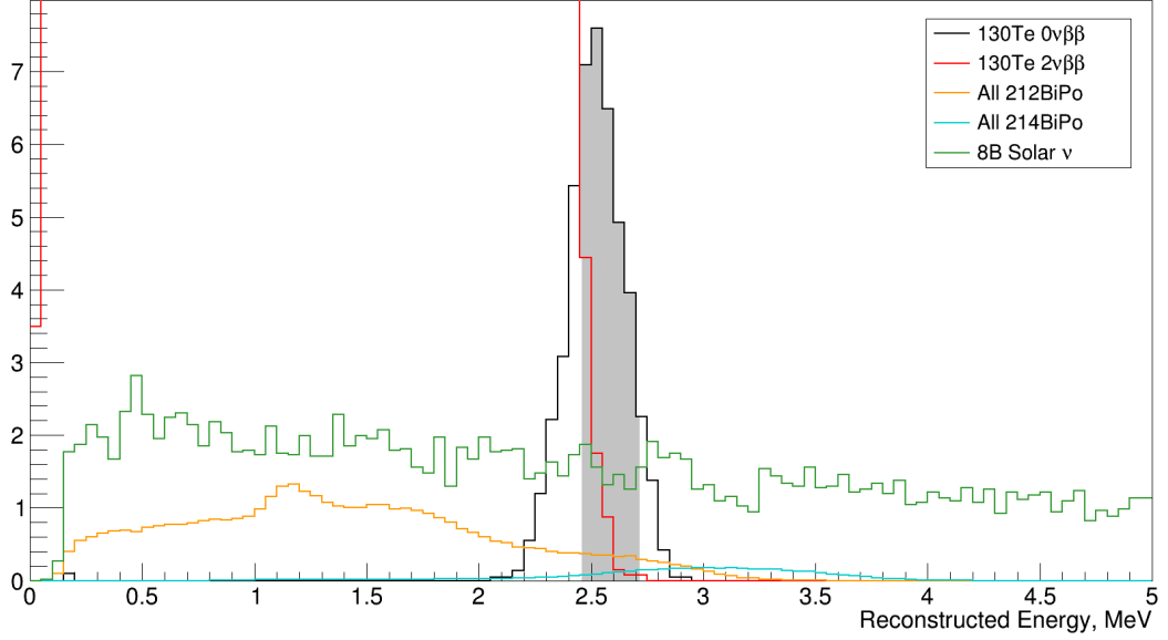
Figure 6.3: The reconstructed energy spectra of ^{130}\text{Te } 0\nu\beta\beta (black), ^{130}\text{Te } 2\nu\beta\beta (red), ^{8}\text{B} (green) and the two BiPo chains: ^{212}\text{BiPo} (orange) and ^{214}\text{BiPo} (blue) in Te_LABPPO, after application of only the fiducial volume cut as described in the main text. The distributions have been normalised to be consistent with the expected number of events in the region of interest - shown in grey - as given in Table 6.1. The 2\nu\beta\beta distribution is significantly larger than the others - peaking at a value of \sim 61000 , hence why its full height has been truncated.
