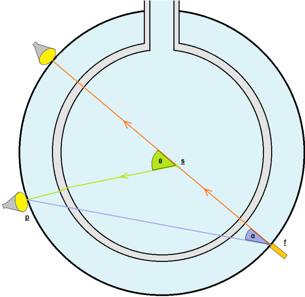
Figure 5.6: An illustration of the SNO+ detector (not to scale) showing a SMELLIE fibre located at position \underline{f} (with respect to the centre of the detector). A photon is emitted from the fibre, and (in this example) scatters at a location \underline{s} in the detection medium, before going on to trigger a PMT located at position \underline{p} , as shown by the green line. The orange line indicates the path the photon would have taken had it not scattered. The scattering angle \theta is shown (green), and \alpha (purple) indicates the angle between the fibre's forward direction and the triggered PMT at \underline{p} .
