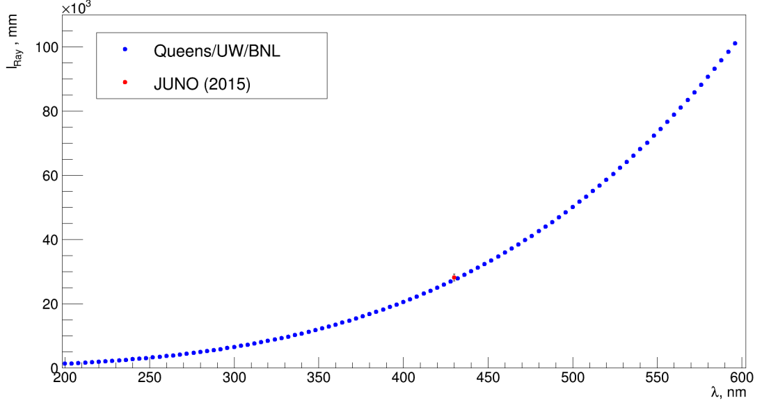
Figure 3.6: Measurements (blue) of the Rayleigh scattering length l_{Ray} of LABPPO at different wavelengths, originally measured at Queens University for SNO+ [87]. Also shown is the recent measurement of the Rayleigh scattering length at \lambda = 430 nm by the JUNO experiment [85] (red), which is in agreement with the measurements from Queen's.
