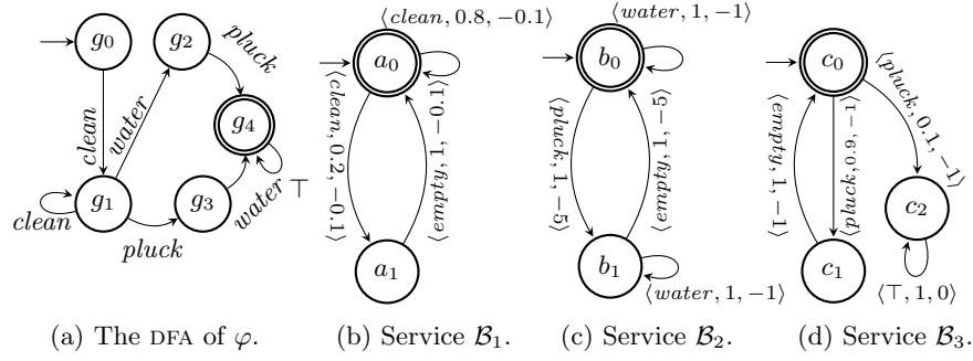
Fig. 1: The garden bot systems and the DFA of the \text{LTL}_f goal.
