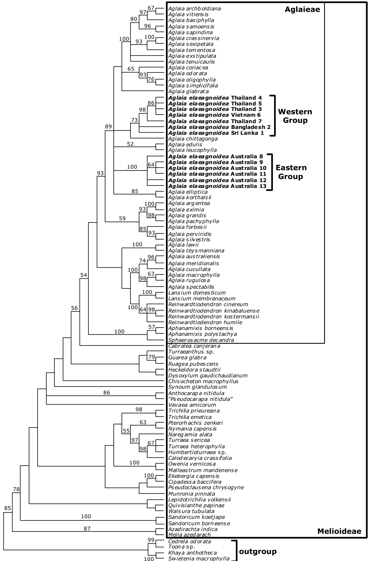
Fig. 2 Strict consensus tree of 288 trees obtained from the maximum parsimony analysis of the ITS dataset of 94 Meliaceae accessions. Numbers are bootstrap percentages (1 000 replicates).
