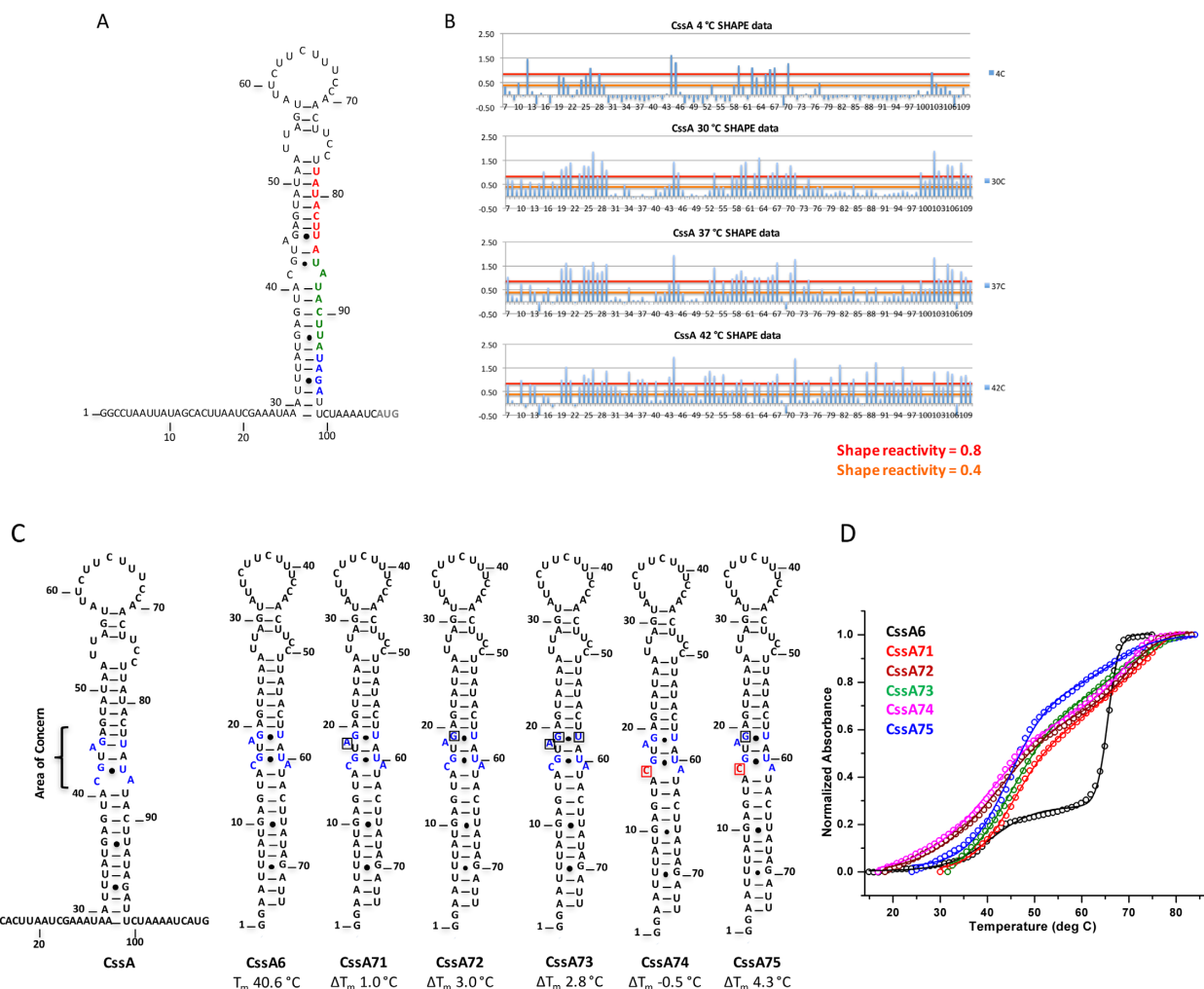
Figure 2. Per residue SHAPE reactivity and mutations introduced to stabilize the structure of the CssA thermometer. (A) Secondary structure of the CssA thermometer as predicted by mfold (35). Red and green colored nucleotides correspond to the two copies of the 8 bp sequence (TATACTTA), whereas blue colored nucleotides correspond to the RBS. The dark gray colored AUG represents the translation start site. (B) Quantification of SHAPE reactivity over the temperature range 4–42°C. Reactivity is classified as follows: 0.4–0.8 and >0.8 correspond to reactive and highly reactive sites, respectively. At 4°C, nucleotides at the 5' and 3'-single stranded regions, the apical loop and the internal AG-U are chemically modified, indicative of a flexible, open structure; as the temperature increases, the flexibility spreads from the apical loop further down the structure; by 42°C, the entire RNA structure becomes reactive. (C) Secondary structure of various mutated thermometers ( CssA 6, 71, 72, 73, 74 and 75), where single nucleotide substitutions were introduced to alter the thermodynamic stability of the thermometer. Except for CssA 74, all mutations generated a more stable RNA. The area highlighted in blue within the secondary structure is the region where mutations were introduced. Red colored nucleotides represent the mutated residue. (D) Thermal melting results for CssA 6, CssA 71, CssA 72, CssA 73, CssA 74 and CssA 75, shown in black, red, wine, olive-green, magenta and blue colors, respectively. The CssA thermometer and its variants have two unfolding transitions around 39–45°C and 69°C, as is most evident in the black melting curve corresponding to CssA . This behavior is due to the formation of a dimeric, more stable RNA structures at the concentrations required for optical melting studies, which are not physiologically relevant.
