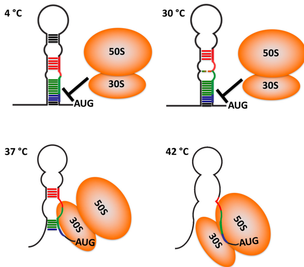
Figure 6. Model for the thermosensing activity of the CsaA thermometer. Cartoon representation of temperature induced unzipping the thermometer, as revealed by NMR spectroscopy and SHAPE assays. Dark colored lines represent stable base pairs, whereas dotted lines correspond to weaker base-pairs which open up at the higher temperatures. At 4°C, all base pair regions are stably formed, and the ribosome cannot access the RBS which is fully occluded. As the temperature is raised toward 30°C, the RNA structure opens up, starting near the apical loop and the A44G45-U84 bulge in center of the repeated 8 bp elements, shown in red and green, respectively. At this temperature, the RBS, shown in blue color, is still inaccessible and protein synthesis inhibited. By 42°C, the thermometer structure is fully open, leading to efficient translation. Around the narrow transition temperature range near 37°C, the thermometer exists in equilibrium between closed and open states. The ribosome (depicted in orange) samples the population of open thermometers to recognize the RBS and initiate translation.
