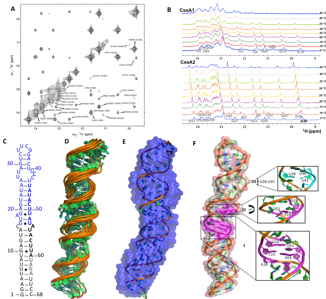
Figure 4. Structural analysis of the Cssa thermometer. (A) Imino-region of the NOESY spectrum of Cssa2, which allowed assignments of the base pair resonances. (B) Temperature dependence of the imino spectra for Cssa1 (top) and Cssa2 (bottom) reveals opening of the structure at the level of individual base pairs. (C) Schematic representation of the secondary structure of Cssa2, based on the NMR structure. Residues corresponding to Cssa3 and Cssa4 are highlighted in blue and black, respectively, to show how the complete structure was constructed by splicing together the two segments. (D) NMR ensemble of 10 refined structures of Cssa2 (residues 1–64). (E) The lowest energy structure of Cssa2 in cartoon representation superposed on the SAXS model shown in blue color; the SAXS results were not used for refinement, they therefore provide independent validation of the structure. (F) Complete structure of Cssa2, highlighting local structural features of the Cssa core structure: (I) A14-U55, C15-A54, G16-U53; (II) A18G19-U51 in magenta and (III) U28-U41 in light green color.
