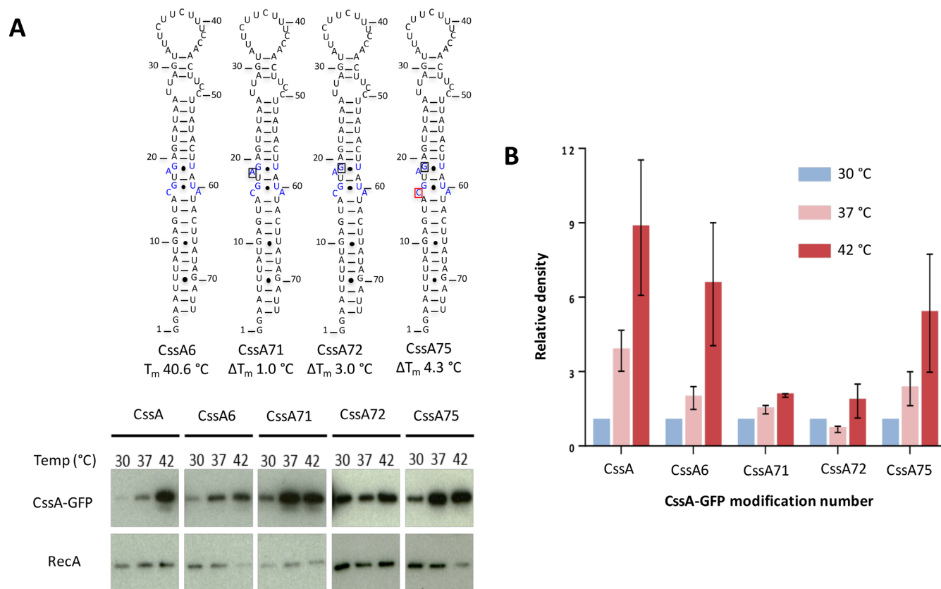
Figure 3. Correlation of thermosensing activity in Escherichia coli with thermodynamic stability. (A) Western blot analysis of CssA-GFP expression. Total protein isolated from indicated strains were subject to western blot analysis. Membranes were probed with antibodies recognizing GFP or RecA. Nucleotide shown in black box is removed in the respective sequence whereas the nucleotide in red box is mutated to U. Their respective melting temperature is shown ( in^\circ\text{C} ) at the bottom of secondary structure. The blue colored residues in CssA6 are mutated/deleted in CssA71, CssA72 and CssA75. (B) Thermosensing properties of the CssA RNA constructs averaged over three biological replicates. The bar chart shows average expression of GFP relative to the loading control RecA, together with their standard deviations.
