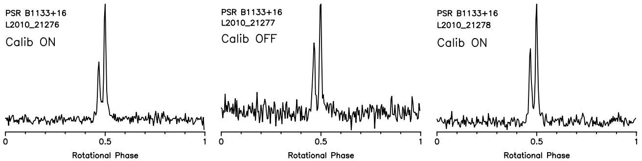
Fig. 11. Three consecutive 20 minute LBA observations of PSR B1133+16 taken on 2010 Nov 5. In between these observations, the station calibration was alternately turned off and then back on. The profiles are all scaled to have the same peak height and as can be seen, the S/N of the cumulative pulse profile decreases by roughly a factor of 3 when the static calibration table is not applied. Five Dutch stations were combined incoherently in these observations, and as such the S/N difference is the average calibration gain for all these stations.
