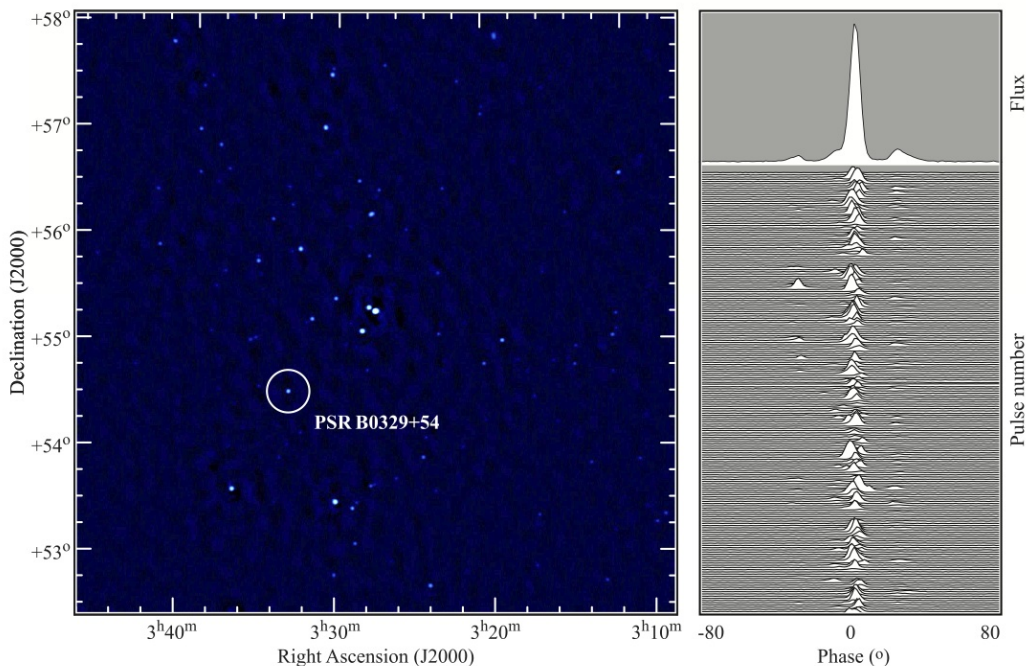
Fig. 12. Left: LOFAR HBA image (139 – 187 MHz) of a 5^{\circ}.5 \times 5^{\circ}.5 field including PSR B0329+54, which is circled. The phase center of the image was pointed to the brightest nearby source, the 40 Jy: 3C 86. The dynamic range in the image is about 1600 and the resolution about 100'' . Right: Pulse stack of roughly 200 individual pulses from PSR B0329+54, detected in simultaneously acquired beamformed data. The cumulative profile of these pulses is shown at the top.
