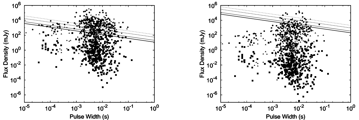
Fig. 3. Sensitivity curves for the HBAs (left panel) and LBAs (right panel) to single pulses as a function of pulse width at a central frequency of 150 MHz (HBAs) and 50 MHz (LBAs) and assuming a bandwidth of 48 MHz. Single pulse widths for 787 pulsars were calculated by assuming them to be one third of the width of the average pulse and then scatter broadened assuming the relationship of Bhat et al. (2004). It was assumed that broadening of the pulse due to uncorrected dispersive smearing was negligible. Single pulse fluxes were determined based on the assumed pulse width and, if known, 100 MHz fluxes from Malofeev et al. (2000) were used. Otherwise, fluxes were extrapolated to 150 MHz from either 400 MHz or 1400 MHz measurements (whichever was available, Manchester et al. 2005) using a known spectral index or a typical spectral index of -1.8 . The symbols are the same as in Figure 2. The lines in all cases correspond to the sensitivity of a single international station (fine dashed line), the incoherent sum of 20 core stations (heavy dashed line), incoherent sum of all the LOFAR stations (filled line) and the coherent sum of 20 core stations (bold line).
