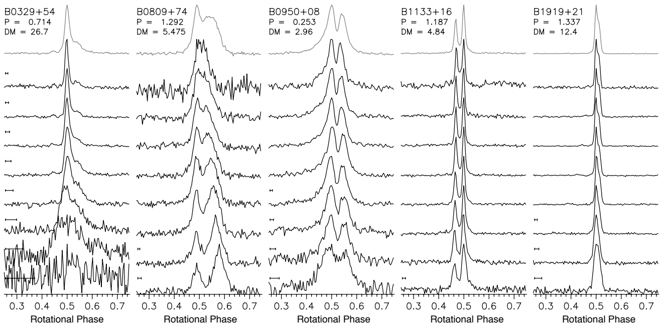
Fig. 15. A sample of average profiles of five pulsars observed with the LBAs using a total of 48 MHz with a channel bandwidth of 12.2 kHz and sampled at a rate of 1.3 ms. In all cases 17 stations were combined incoherently and the observation duration was 2 hr, except for PSR B1919+21 which was observed for 1 hr. The lower 8 profiles correspond to observations with 6 MHz of bandwidth centered at frequencies, from lowest to highest, of 35, 41, 47, 53, 59, 65, 71 and 77 MHz respectively. The top profile shows the summed profile from all 8 bands. At present there is no flux calibration for the LOFAR data hence no flux density scale is shown and profiles have been normalised to the peak intensity. The bar on the left hand side indicates the smearing due to dispersion across the 12.2 kHz channels and is shown only when it exceeds 3 ms. The periods are given in seconds and the dispersion measure in \text{pc cm}^{-3} .
