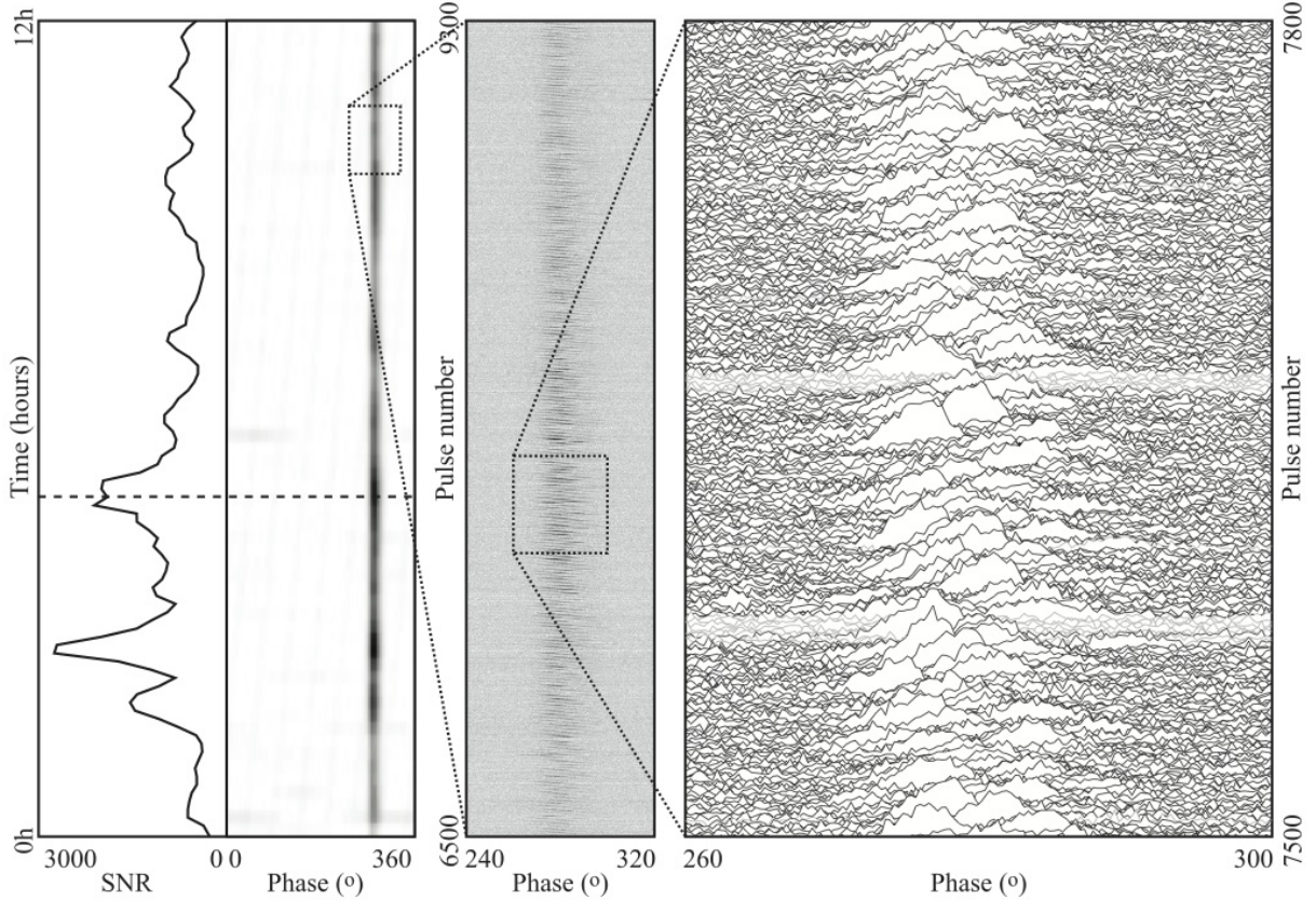
Fig. 13. A 12 hr observation of PSR B0809+74 made with 4 incoherently added HBA stations in the frequency range 140–164 MHz. The left-most plots highlight how the S/N varies throughout the observation, mostly due to scintillation but also from the changing telescope sensitivity with zenith angle. The dashed line marks the time when the pulsar crosses the meridian. The S/N value shown in the left hand plot is calculated for each 7.2 min integration. The middle plot shows an hour of data when the pulsar most frequently nulled and exhibited mode changing. The right-most plot zooms in on two long nulls (grey), that are easily distinguished from the on-pulses (black). Note the quality of the data even in this region when the pulsar was not particularly bright, and at a high zenith angle, where the sensitivity of LOFAR is reduced by a factor of roughly two.
