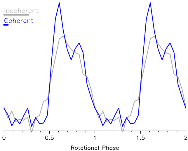
Fig. 17. For comparison, two consecutive 20-minute observations of the 1.88-ms pulsar J0034-0534 at a central observing frequency of 143 MHz and with a spectral resolution of 12kHz (corresponding time resolution of 82\mu\text{s} ) are shown. The data for the “Incoherent” profile has only been corrected for dispersion by applying a frequency dependent time delay to the spectral channels in the offline post-processing. In contrast, the data for the “Coherent” profile has also been coherently dedispersed on-line in order to remove the intra-channel dispersive smearing. The increased effective time resolution of the coherently dedispersed data is evident from comparing the two profile morphologies; e.g., two profile components are visible in the “Coherent” profile which are washed out in the “Incoherent” profile. The off-pulse noise has been scaled to the same level to facilitate comparison of the S/N. The effective time resolution is represented by the two horizontal bars on the left-hand side, and reflects the intra-channel smearing in the case of the incoherently dedispersed profile.
