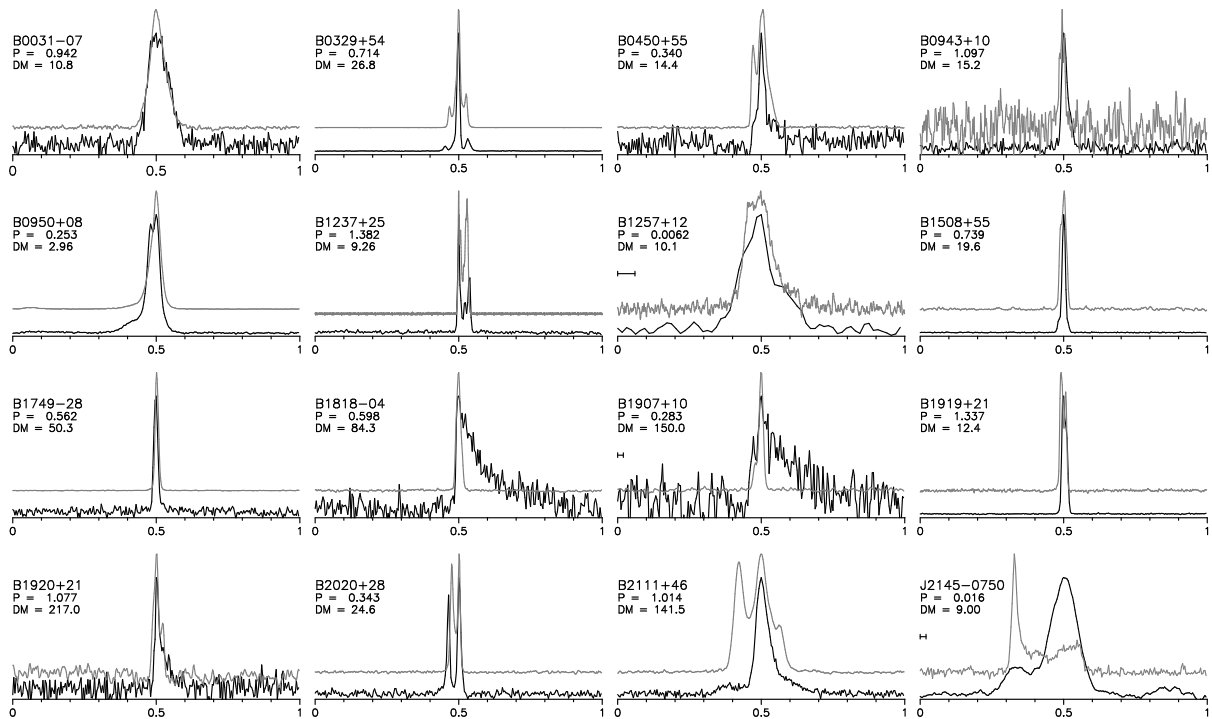
Fig. 4. A sample of average pulse profiles from LOFAR observations of various pulsars made during the commissioning period. The dark line corresponds to LOFAR observations made with the HBAs with 48 MHz of bandwidth, divided into 3968 channels, at a central frequency of 163 MHz. Typically about 12 stations were used and they were combined incoherently. At present there is no flux calibration for the LOFAR data, hence no flux scale is shown. The majority of the observations are \sim 1000 s in duration, except for PSR B1257+12, which was observed for 3 hr. The dispersion measure smearing is less than two bins for the majority of the pulsars shown; if the smearing is large, this is indicated by a bar on the left hand side. The lighter line corresponds to observations made at 1408 MHz by Gould & Lyne (1998) except for the observations of PSR B0943+10 which was at 608 MHz and PSR B1237+25 which was at 1600 MHz (from van Hoensbroech & Xilouris 1997). All archival profiles are from the EPN database ( www.mpifr-bonn.mpg.de/div/pulsar/data/browser.html ); they are shown for illustration purposes and are manually aligned. Both the LOFAR and EPN profiles have been normalised to the peak intensity. The periods are given in seconds and the dispersion measures in \text{pc cm}^{-3} .
