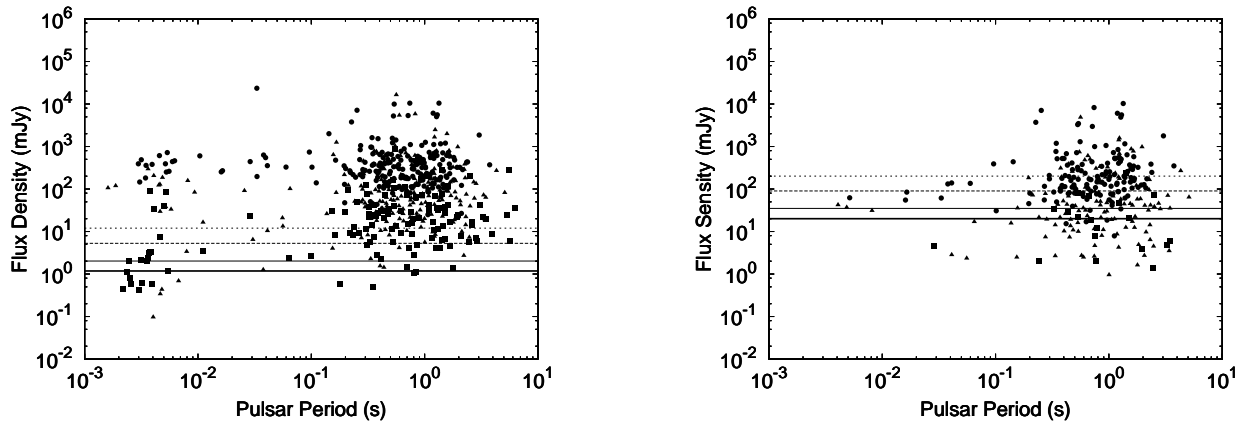
Fig. 2. Sensitivity curves for 600-s observations using the HBAs (left) and the LBAs (right) with a bandwidth of 48 MHz, compared to the extrapolated flux densities of 787 known pulsars at 150 and 50 MHz respectively. Flux densities were determined using, if known, 100 MHz fluxes from Malofeev et al. (2000) (circles) otherwise fluxes at either 400 MHz (triangles) or 1400 MHz (diamonds) (Manchester et al., 2005), whichever were available, were used and scaled to 150 MHz using a known spectral index or a typical spectral index of -1.8 (squares). All of these flux densities were scaled by \sqrt{W/(P-W)} , where W is the effective pulse width and P is the period of the pulsar, to incorporate broadening of the profile by scattering in the ISM. W was determined by combining the pulse width at high frequencies with the broadening due to scattering in the ISM, based on the model of Bhat et al (2004). If W > 0.75P then the pulsar was deemed undetectable. It was assumed that broadening of the profile due to uncorrected dispersive smearing was negligible. MSPs are shown by the open symbols and “normal” pulsars by filled symbols. The lines in both cases correspond to the sensitivity of a single international station (fine dashed line), the incoherent sum of 20 core stations (heavy dashed line), incoherent sum of all LOFAR stations (filled line) and the coherent sum of 20 core stations (bold line).
