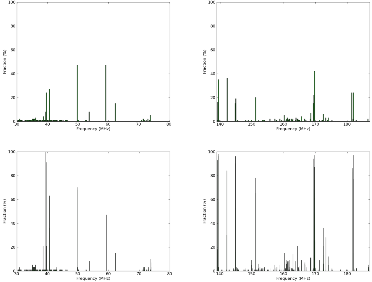
Fig. 9. An initial summary of the RFI situation across our most commonly used sections of the LBA (left-hand panels) and HBA (right-hand panels) frequency ranges. The upper and lower panels correspond to a frequency channel width of 195 kHz and 12 kHz, respectively. Each line in the plot corresponds to the percentage of observations in which the particular frequency channel was affected by RFI.
