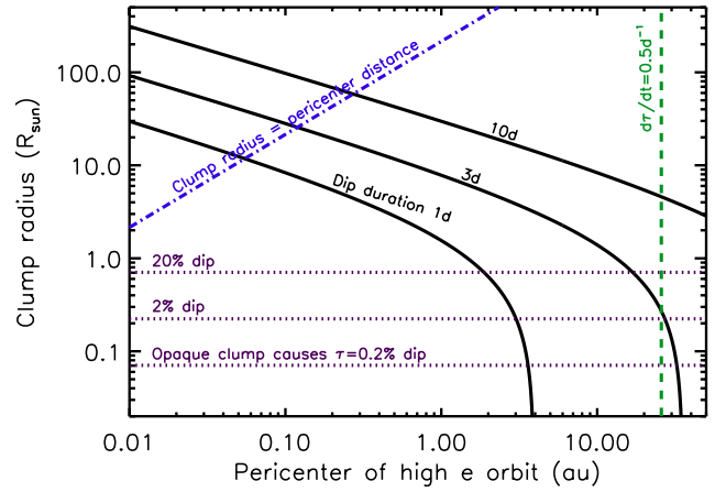
Figure 13. Size vs. pericenter parameter space for high eccentricity comet-like orbits. Dotted lines show lower limits on the clump sizes from the dip depths. The dashed line is the outer limit set by the light curve gradient, noting that this limit decreases with decreasing optical depth, e.g., the limit would be at a pericentre that is 25 times smaller than that plotted if the clumps have optical depth of 0.2 (line not shown in figure). The dot-dashed line is where the clump radius equals the pericenter distance, though the clumps could exist above here if they are elongated along the orbital direction. The solid lines are of constant dip duration.
