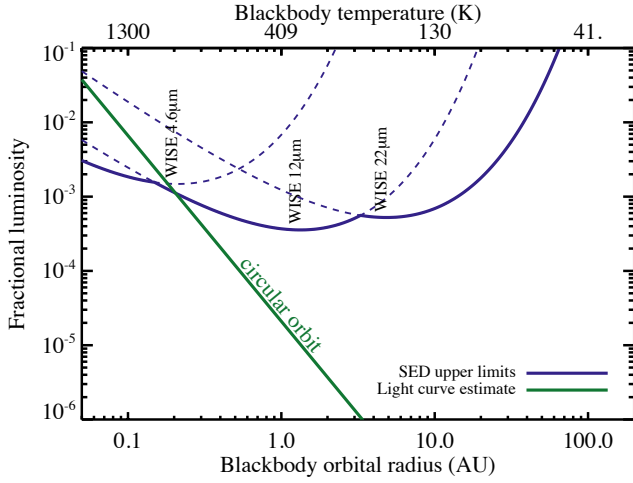
Figure 11. Fractional luminosity limits (blue lines) and an estimate of the system dust content from the light curve (green line). The dust level is constrained to lie below the blue line by the WISE photometry (4.6 \mu\text{m} , 12 \mu\text{m} , and 22 \mu\text{m} ). The green line integrates the optical depth in the light curve assuming that clumps are similar in size to the star and on circular orbits. If the clumps lie beyond about 0.2 AU the IR non-detection of the dust is unsurprising, although many scenarios require more emission than that from dust seen to pass along our line-of-sight to the star. Refer to Section 4 for details.
