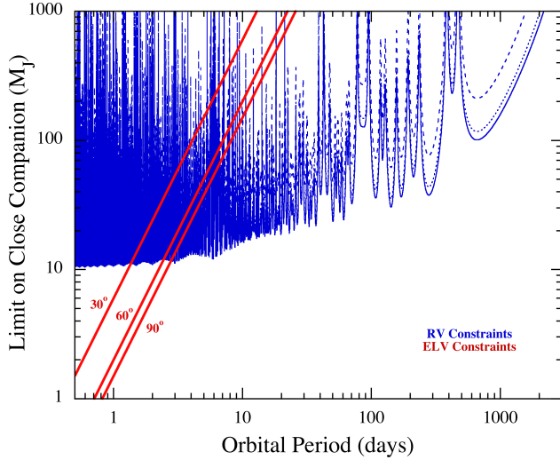
Figure 9. Upper limits (2- \sigma confidence) to a hypothetical companion mass from the lack of ELVs (red curves) and lack of RV variations on four occasions (blue curves). Each type of constraint is shown for three different assumed orbital inclination angles (30°, 60°, 90°); these are marked directly on the ELV constraint curves, and can be inferred from the dashed, dotted, and solid curves, respectively, for the RV constraints. These results indicate that there are no objects heavier than a super-Jupiter in close orbits with P_{\text{orb}} \lesssim 2 days, and likely no heavier in mass than a brown dwarf for P_{\text{orb}} \lesssim 300 days. Refer to Section 2.6 for details.
