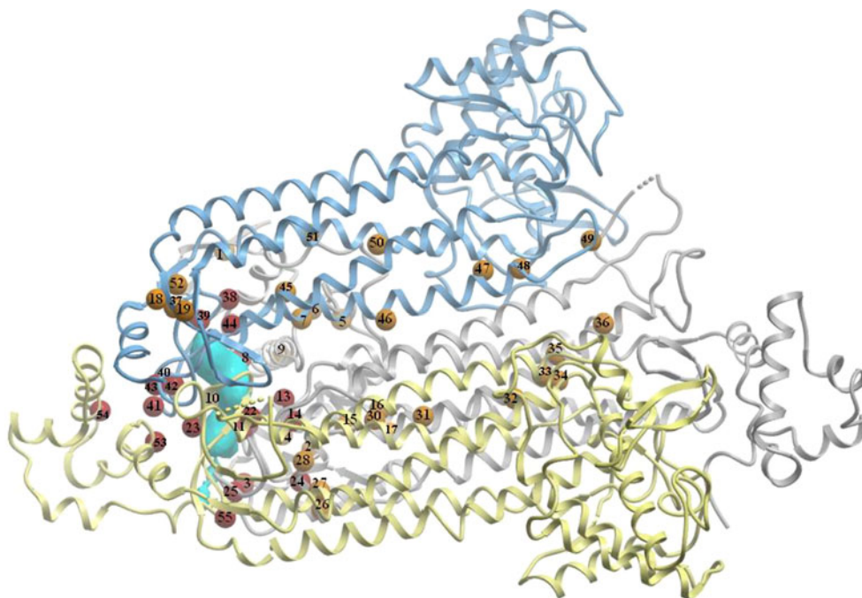
Fig. 2 Clustering of human fumarase missense mutations observed in FHD, MCUL1 and HLRCC. The active site is highlighted in cyan. Positions of amino acid mutations are indicated as small spheres and numbered according to Table 2. The positions around the active site are indicated in red, mutations affecting inter- or intrasubunit interactions are indicated in dark yellow. For clarity, one monomeric subunit is omitted
