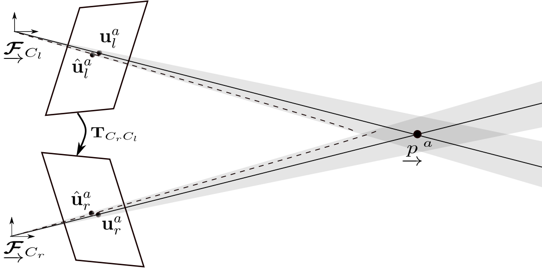
Figure 2.2: An illustration of the process of triangulating a 3D world point, \underline{p}^a , from two image correspondences. The true image points, \mathbf{u}_l^a and \mathbf{u}_r^a , satisfy the epipolar constraints and are the intersection of each image plane with the solid lines connecting \underline{p}^a and the camera centers, \underline{\mathcal{F}}_{C_l} and \underline{\mathcal{F}}_{C_r} . The observed points, \hat{\mathbf{u}}_l^a and \hat{\mathbf{u}}_r^a , are corrupted by noise and therefore do not satisfy the epipolar constraints, i.e., their epipolar lines (dashed) are skew and do not intersect. The shaded regions represent the uncertainty envelopes caused by this sensor noise, and the region where they overlap represents the uncertainty in the triangulated position of \underline{p}^a . The transform, \mathbf{T}_{C_r C_l} , represents the baseline transform in a stereo pair, or the motion of the camera in a monocular system.
