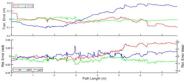
Fig. 7. The translational and rotational errors for the egomotion of the camera over its path compared to ground-truth trajectory data. Errors are reported in the egocentric camera frame with the z-axis along the optical axis, and the y-axis down.
