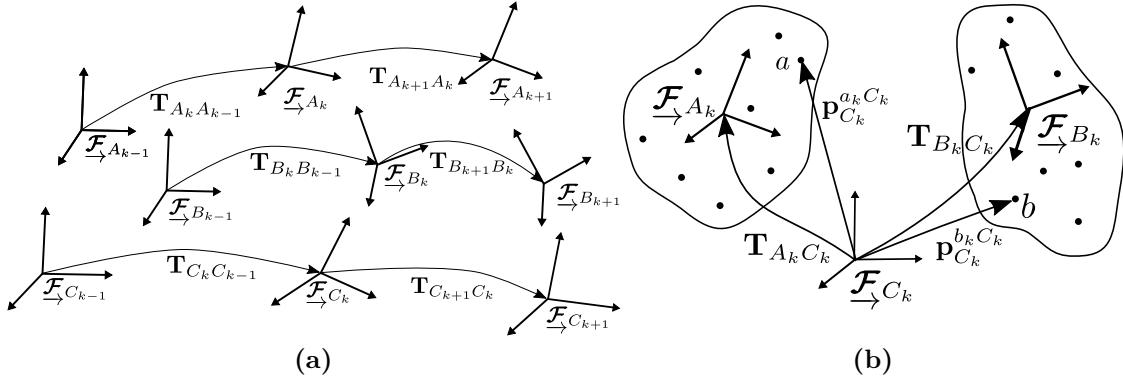
Figure 3.1: Illustrations of the MEP showing the motion of frames through time, (a), and the relative point observations, (b). A series of two independent third-party motions, \mathcal{F}_{\rightarrow A} and \mathcal{F}_{\rightarrow B} , are observed by a moving camera, \mathcal{F}_{\rightarrow C} , through feature measurements on the objects, \mathbf{p}_{C_k}^{a_k} and \mathbf{p}_{C_k}^{b_k} . Solving the problem requires simultaneously segmenting and estimating the set of measurements.
