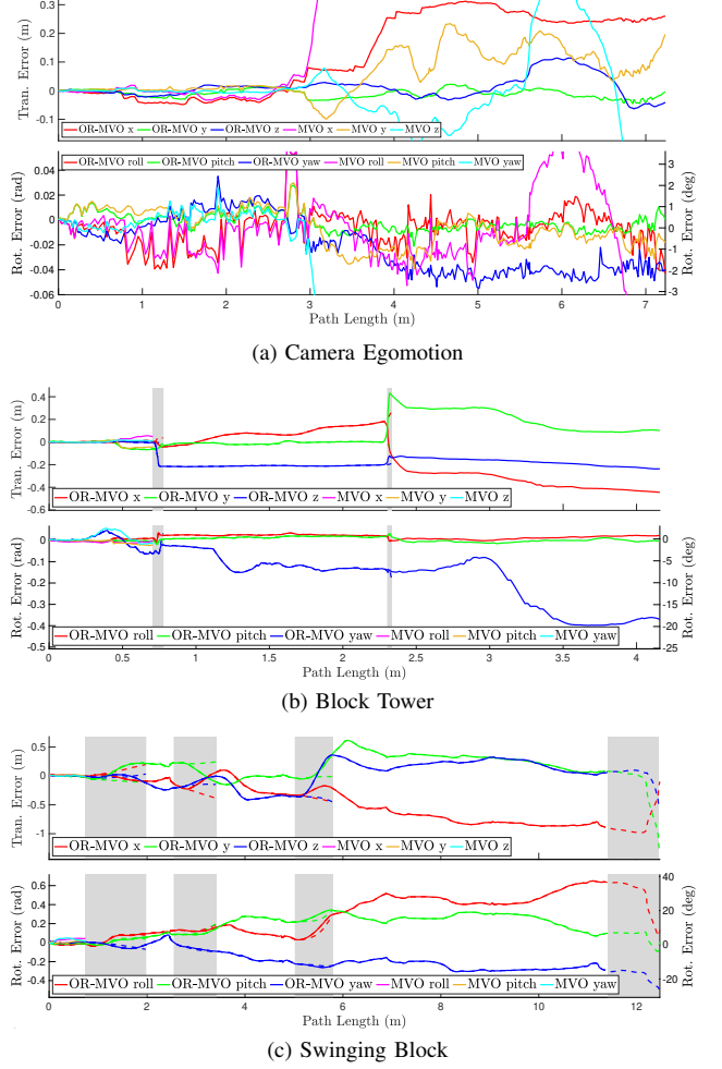
Fig. 5. The translational and rotational errors in the estimated motion of the camera (a), the block tower (b), and the swinging block (c) for a 300-frame section of occlusion_2 unconstrained segment of the OMD. The occlusion-robust MVO errors are displayed in red-green-blue, and the original MVO errors are displayed in magenta-yellow-cyan. Each object is compared to ground-truth trajectory data and errors are reported in an arbitrary geocentric frame with the z-axis up and arbitrary x- and y-axes. Grey regions show when the swinging block was occluded by the tower, or when the tower was stationary and effectively part of the background. Dashed lines represent the extrapolation error and the solid lines represent the error in the direct or interpolated estimates. As expected, the original MVO pipeline failed to track the blocks past their first occlusions. This also led to significant errors in the egomotion estimate that have been cropped in (a).
