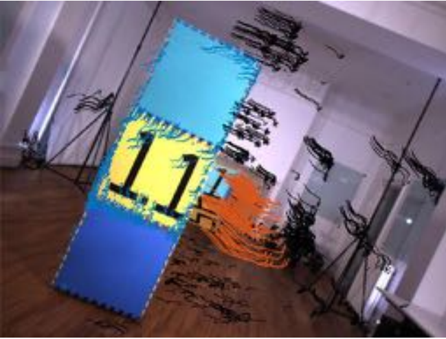
Fig. 7. Motion segmentation produced by Multimotion Visual Odometry [7] for the unconstrained SE(3) camera segment of the occlusion section of the dataset. The egomotion of the camera is estimated from the static points in the scene shown in black. The occluded block (red) is tracked until it moves behind the block tower (blue).
