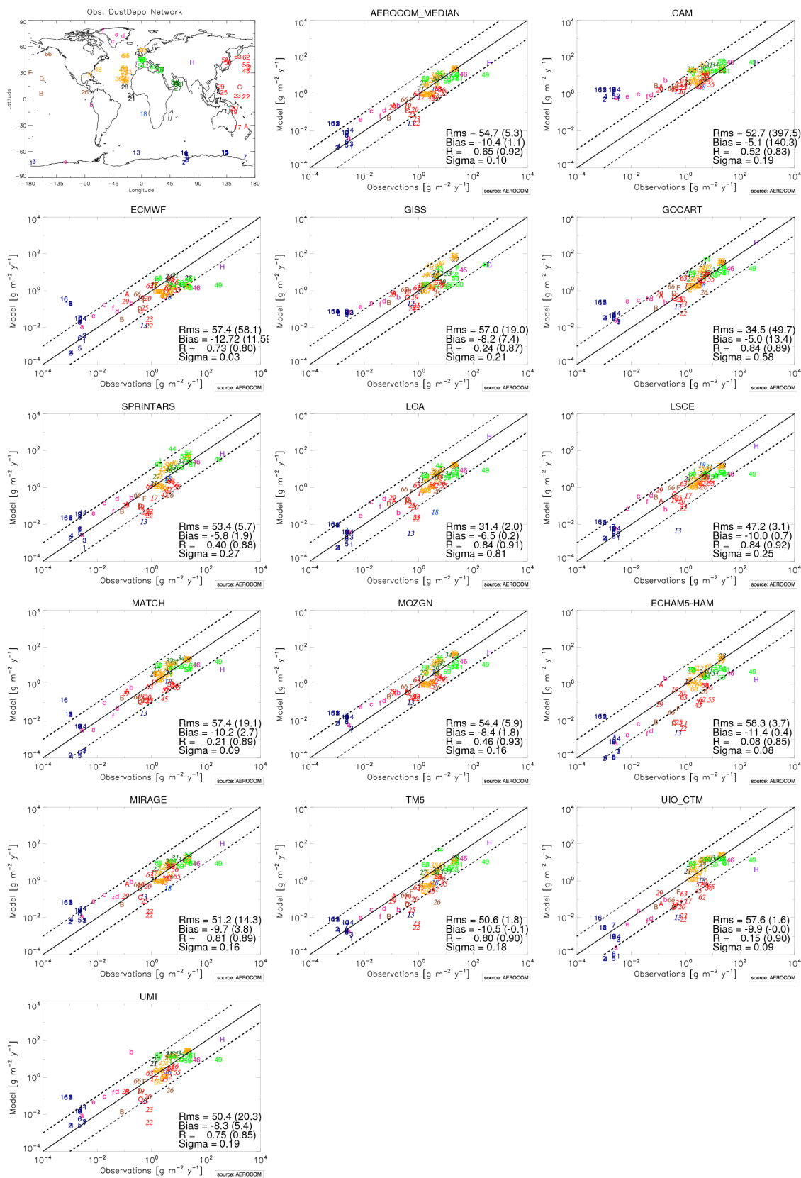
Fig. 1. Measured yearly deposition fluxes versus modeled ones; units are \text{g m}^{-2} \text{yr}^{-1} . Location for each data point in the scatter plot is given in the upper left subfigure. West/East Pacific (red/brown), North/Tropical/South Atlantic (orange/black/light-blue), Middle East/Asia/Europe (violet/purple/light green), Indian/Southern Ocean (dark green/dark blue) and Antarctica (dark brown), (North/South Atlantic (orange/black/light-blue), Middle East/Asia/Europe (violet/purple/light green), Indian/Southern Ocean (dark green/dark blue) and Antarctica (dark brown) from Ginoux et al. (2001)/Mahowald et al. (2009)/DIRTMAP/Mahowald et al. (1999) are indicated by letters; non-italic numbers/italic numbers/lower-case letters. Root mean square error (RMS), bias, ratio of modeled and observed standard deviation (sigma) and correlation ( R ) are indicated for each model in the lower right part of the scatterplot. Mean normalized bias and normalized root mean square error are given in parenthesis next to R . Black continuous line is the 1:1 line whereas the black dotted lines correspond to the 1:1 and 1:10 lines. Names and locations for each selected station are given in Table S1 in the Supplement.
