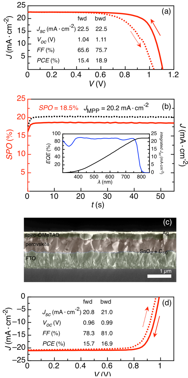
Fig. 3: Forward and backward JV characteristics (a), SPO curve (b) (inset: EQE spectrum), and a cross-sectional colour-enhanced SEM image (c) of the champion (FA_{0.83}MA_{0.17})_{0.95}Cs_{0.05}Pb(I_{0.9}Br_{0.1})_3 solar cell in planar n-i-p configuration. (d) JV characteristics of the best (FA_{0.83}MA_{0.17})_{0.95}Cs_{0.05}Pb(I_{0.9}Br_{0.1})_3 cell in p-i-n configuration.
