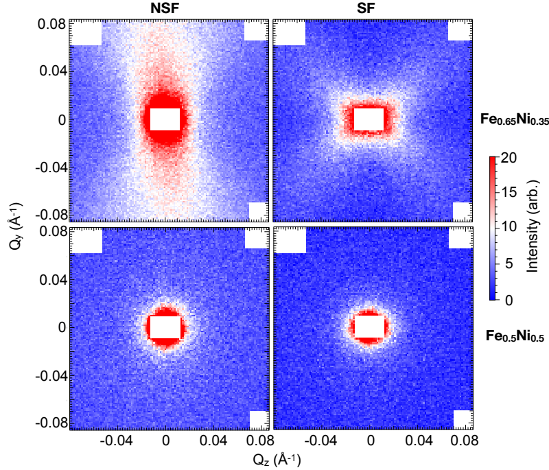
Figure 2. SANS with polarization analysis at 300 K and 0.6 T for INVAR Fe_{0.65}Ni_{0.35} (top row) and non-INVAR Fe_{0.5}Ni_{0.5} (bottom row). The left column shows the average non-spin-flip cross-section and the right column shows the spin-flip cross-section
