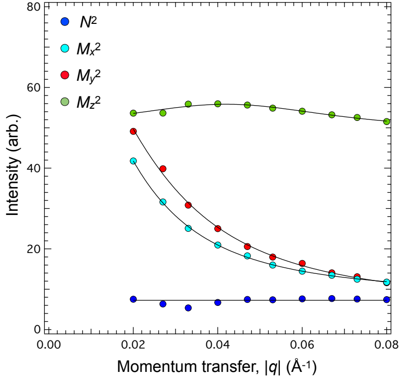
Figure 4. Individual SANS components, nuclear N^2(q) (blue), transverse magnetic M_x^2(q) (cyan) and M_y^2(q) (red) and longitudinal magnetic M_z^2(q) (green) measured on \text{Fe}_{0.65}\text{Ni}_{0.35} at 300 K and 0.6 T extracted using Eqs. 2. The lines are fits to a Lorentzian form.
