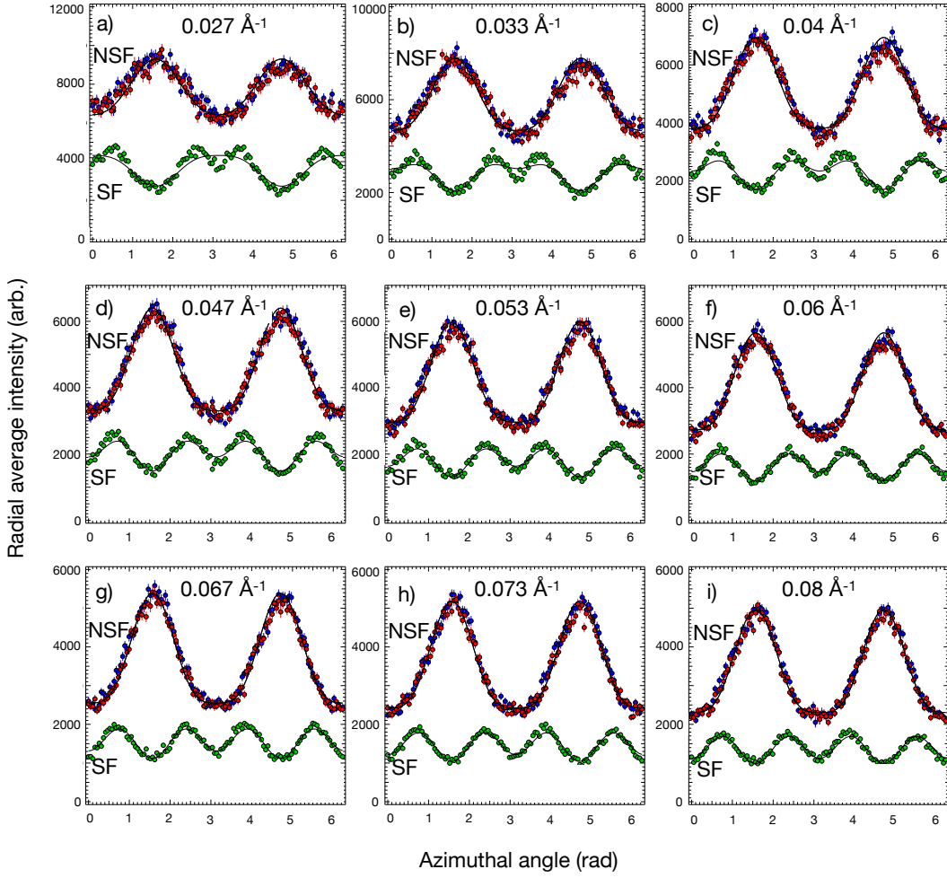
Figure 3. Radially averaged plots at constant |q| of the NSF (blue: (d\Sigma/d\Omega)^{++} , red: (d\Sigma/d\Omega)^{--} ) and average SF (green) SANS from Fe_{0.65}Ni_{0.35} at 300 K and 0.6 T, plotted against the azimuthal angle \phi . Plots a) through i) show the SANS at 0.027 \leq |q| \leq 0.08 . The solid lines through the data are fits to Eqs. 2.
