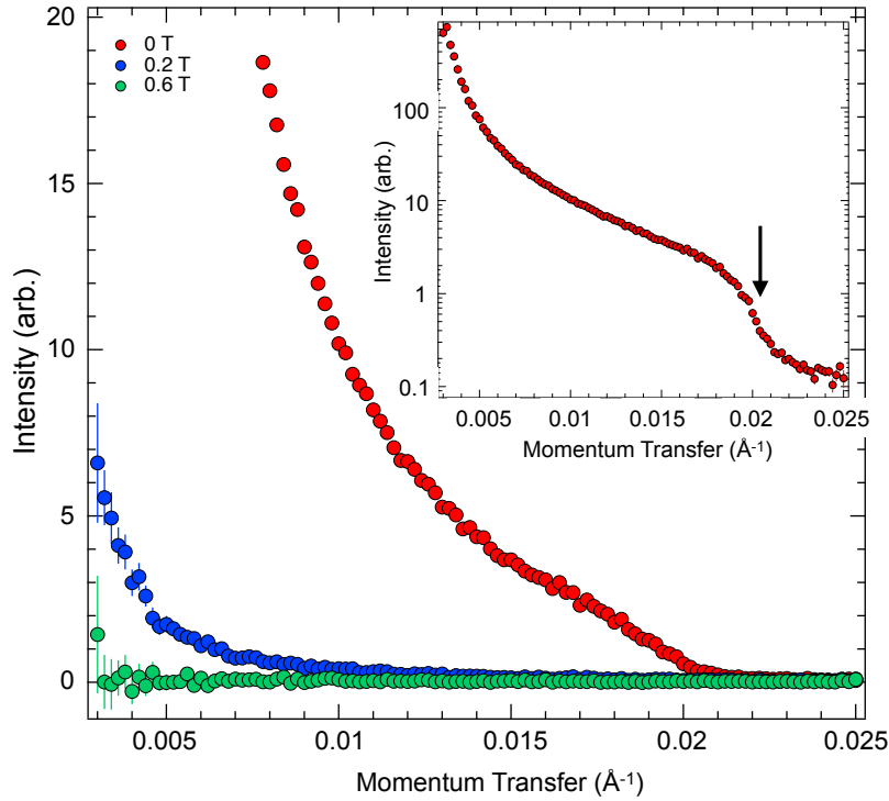
Figure 1. Radially averaged SANS in Fe_{0.65}Ni_{0.35} as a function of field. The SANS measured at 2 T has been subtracted. By 0.6 T the magnetic domain SANS is suppressed and the sample is single domain. The inset shows unsubtractred data taken at zero field with the arrow indicating the spin-wave scattering cut-off.
