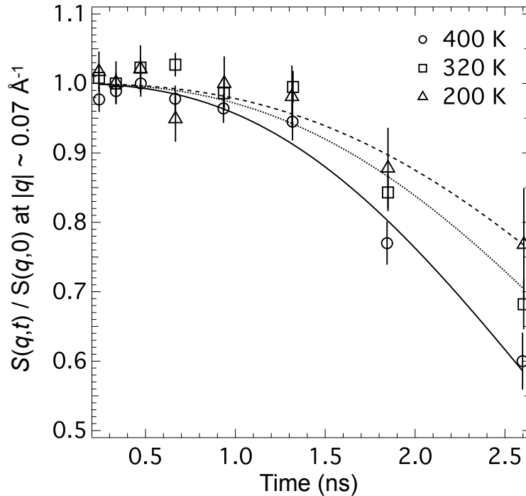
Figure 5. The normalised intermediate scattering function S(Q,t)/S(Q,0) with |q| \simeq 0.07 \text{ \AA}^{-1} measured on Fe_{0.65}Ni_{0.35} using the IN11 spin-echo spectrometer as a function of temperature. These show evidence of slow spin-fluctuations in the ordered ferromagnetic state. Lines are fits to a stretched exponential decay in order to loosely quantify the relaxation time.
