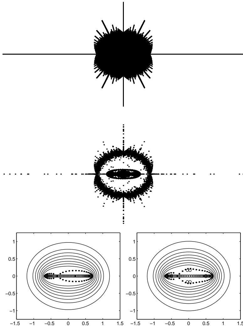
FIGURE 4. Real single-entry perturbations to T(a) and T_n(a) for a(t) = t + \frac{1}{9}t^{-1} and \Omega = [-5, 5] . The top picture is the union of \text{sp}_\Omega^{(j,k)} T(a) over (j, k) \in \mathbf{N} \times \mathbf{N} . The middle picture shows computed eigenvalues of 1000 single-entry perturbations to T_{50}(a) , where the perturbed entry is chosen by random anywhere in the matrix, and the perturbation itself is randomly chosen from the uniform distribution on [-5, 5] . The interior elliptical region of high eigenvalue concentration in the middle picture is an artifact of finite precision arithmetic; this is revealed by the two bottom pictures, which show the boundaries of the pseudospectra \text{sp}_\varepsilon T_{50}(a) (left) and \text{sp}_\varepsilon (T_{50}(a) + \omega e_5 e_4^*) with \omega = -3 (right) for \varepsilon = 10^{-1}, 10^{-3}, \dots, 10^{-15} . Dots ( \cdot ) denote computed eigenvalues, circles ( \circ ) show the true eigenvalue locations.
