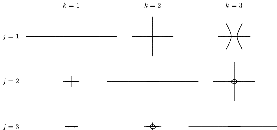
FIGURE 1. The sets \Lambda(a) \cup H_{\Omega}^{jk}(a) for a(t) = t + \frac{1}{9}t^{-1} , \Omega = [-5, 5] , and the nine possible choices of (j, k) with j, k \in \{1, 2, 3\} .
