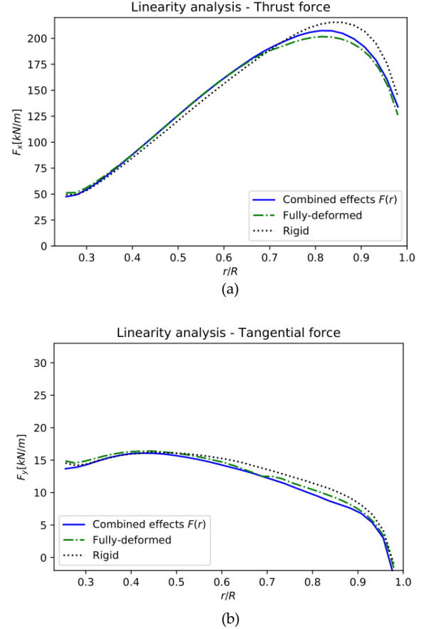
Fig. 13. Linearity superposition analysis of the different deformation components for the thrust (a) and for the tangential (b) forces at a tip-speed ratio of 7.0. Three cases are presented: The rigid blade, the fully-deformed, and the combined effects F(r) according to eq. 8.
