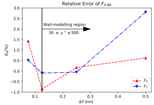
Fig. 8. Relative error for the different first element thickness values. Notice the increasing error in (a) thrust and (b) the tangential force at 0.8R when \Delta Y < 0.125 [mm]: It is caused by the model entering a buffer region where 5 < Y^+ < 30 . In this region, the wall-modelling approach is no longer valid, but the mesh is still too coarse to resolve the boundary layer.
