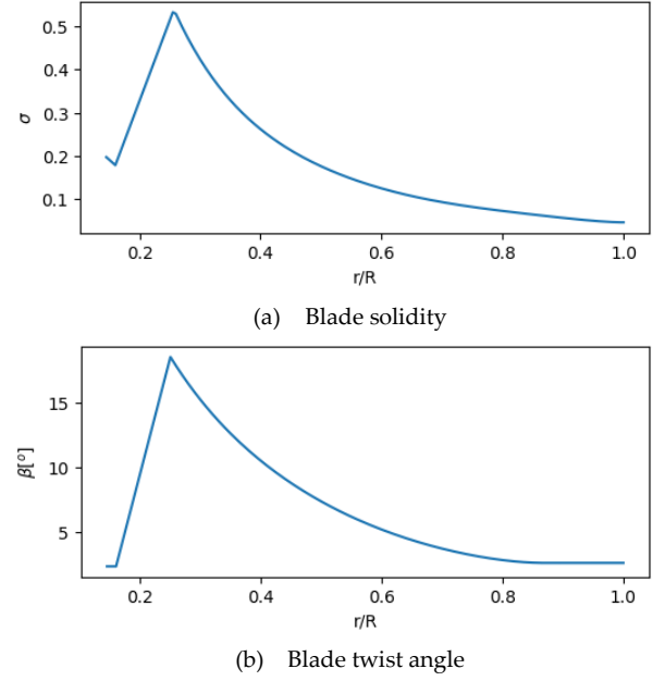
Fig. 3. Original rotor geometric characteristics as functions of the radial position [14].
