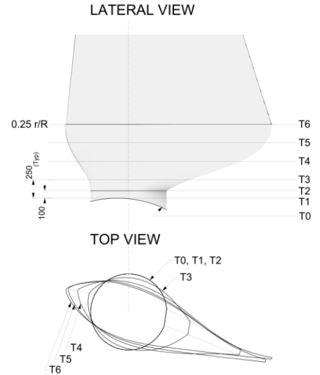
Fig. 4. Details of the modified blade root section. The lateral and top views display the soft transition between the blade and the nacelle. Dimensions are in millimetres.
