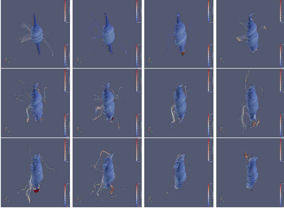
Figure 7: Plot of stream tube of the magnetic field \mathbf{B}_h obtained with Algorithm 1 with R_e = \infty, R_m = \infty, h = 1/16 and \Delta t = 1/1000 . The lines with arrows show \mathbf{u}_h . The plot shows a sequence of magnetic tubes as time goes from top left to going right and then at the next row from left to right, each of which corresponds to time level, T = 0.05, 0.1, 0.2, 0.3, 0.4, 0.5, 0.6, 0.7, 0.8, 0.9, 1.0 and 1.1 .
