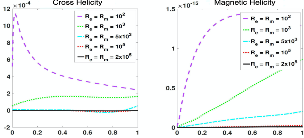
Figure 4: Changes in the right hand side of the equation for \mathcal{H}_c (left) (29) and \mathcal{H}_m (right) (26) obtained by Algorithm 1 with various choices of R_e and R_m . Here h = 1/16 and \Delta t = 1/1000 .
