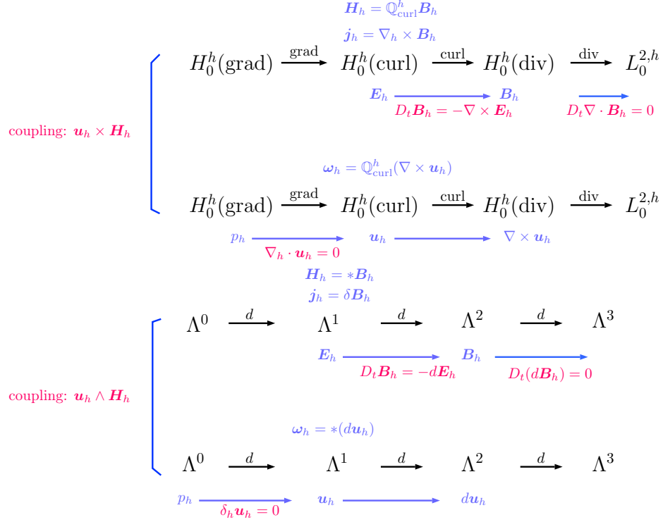
Figure 1: Choice of variables, spaces and their relations. Top: functions and differential operators. Bottom: differential form point of view.
